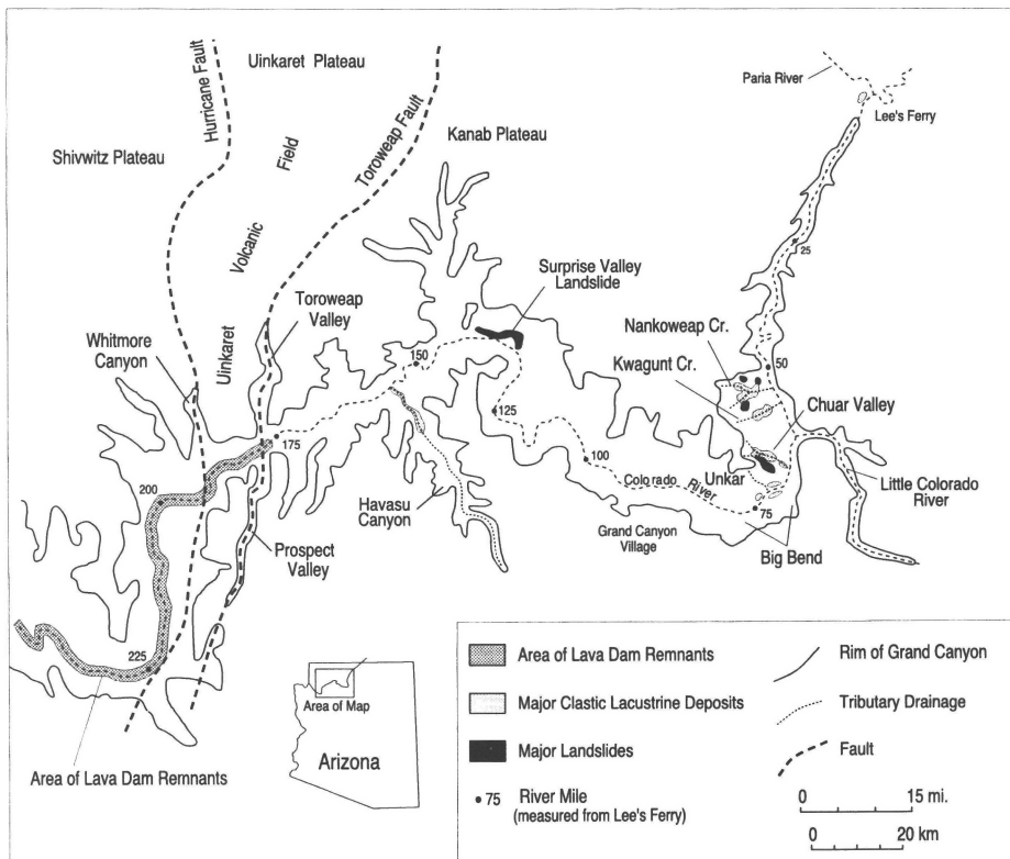
Figure 1. Location and Geologic Map of Grand Canyon, Arizona.
