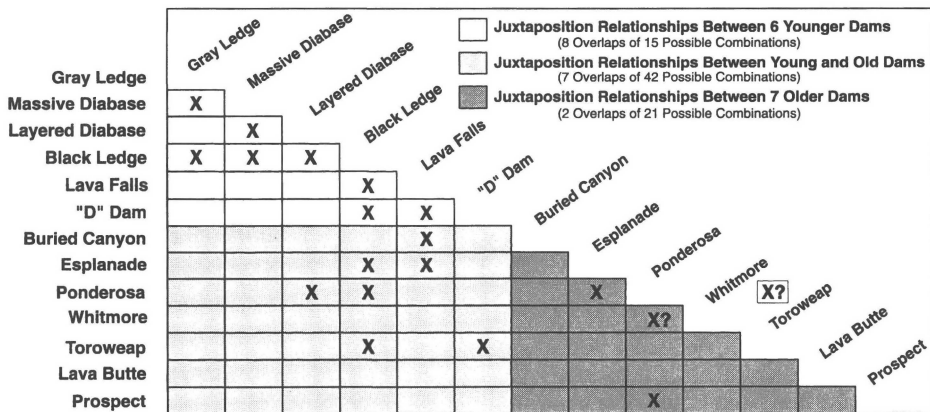
Figure 3. Relative Age / Juxtaposition Relationships of Lava Dams.
