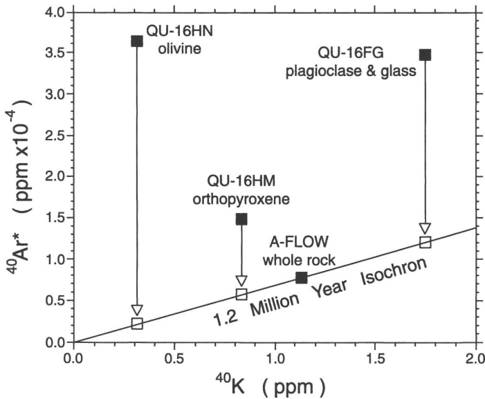
Figure 2. K-Ar plot for basalts of Toroweap Dam. If the lava dam has an "age" of 1.2 Ma, the three QU-16 mineral concentrates should plot as a line on the 1.2 Ma reference isochron with whole rock sample "A-FLOW" (arrows indicate where each mineral concentrate should plot). Instead the mineral concentrates plot significantly above the 1.2 Ma reference isochron, arguing that the lava dam contains significant "excess radiogenic argon." Can any basalt sample from the Toroweap Dam be assumed to be free of "excess radiogenic argon?"
