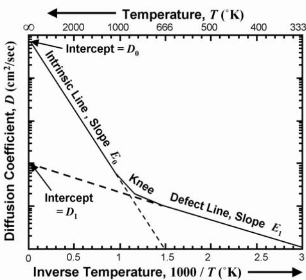
Figure 4(a) Typical Arrhenius plot.
