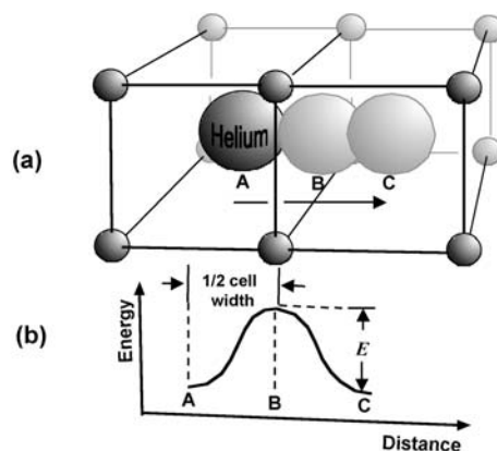
Figure 3 Helium atom moving through crystal.
