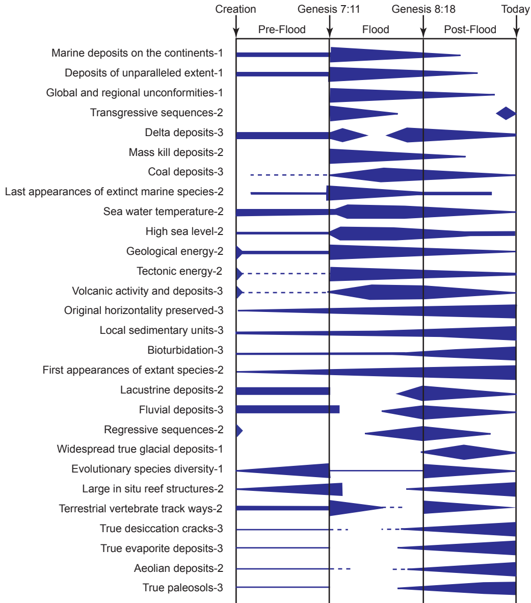
Figure 1. The thickness of a line indicates the relative importance of a particular process during a time period. The number following each criterion (1, 2, or 3) is a rank of how important we feel each criterion is within a Flood model (1 being the highest).
