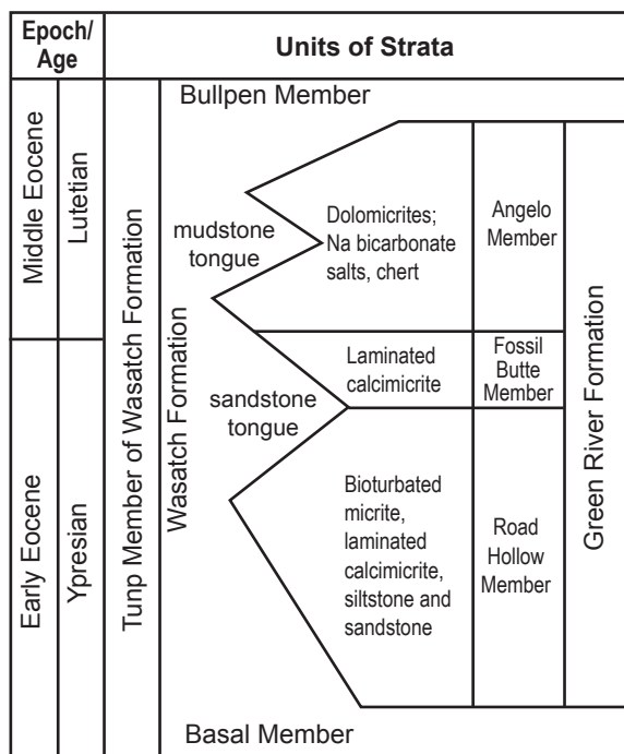
Figure 9. The Wasatch Formation interfingers with the Green River Formation. Figure modified from Buchheim and Eugster (1998).
