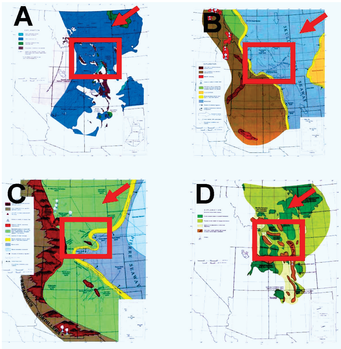
Figure 3. Maps showing changes that take place in aerial depositional extent of formations during A-deposition of the Madison Formation, B-deposition of the Thermopolis Shale, C-deposition of the Lance Formation, and D-deposition of the Fort Union Formation. Formations indicated by red arrows. The state of Wyoming is highlighted in red. Note the aerial extent of deposition changes rapidly from C to D. This is also a change from dominantly marine to dominantly non-marine. Figures modified from the Geologic Atlas of the Rocky Mountain Region , 1972: A—Craig, p. 105; B—McGookey, p. 200, C—McGookey, p. 225; D—Robinson, p. 237.
