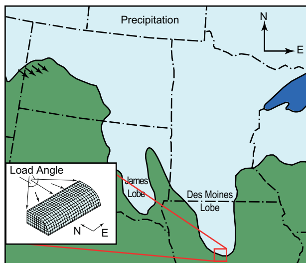
Figure 2. Global continental scale picture of the Laurentide Ice Sheet with the local scale Des Moines Ice Lobe Section illustrating the finite element mesh and boundary condition used. The global continental scale was influenced by precipitation rates far north of the local scale. The local scale boundary velocities were retrieved from previous global simulations of Horstemeyer and Gullett (2003) and applied to the back edge of the Des Moines front edge lobe illustrated here.
