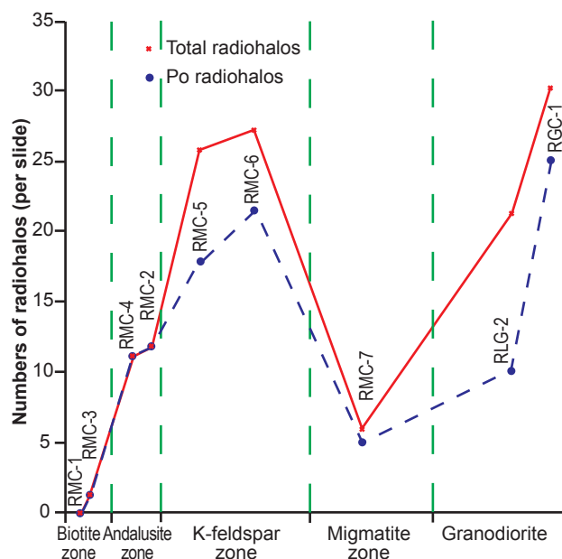
Figure 6. Plot of numbers of radiohalos per slide in each sample along the west-east traverse shown in Figure 2. The different metamorphic zones and the granodiorites are marked along the horizontal axis, and the relative lateral distances between sample locations are approximately to scale.
