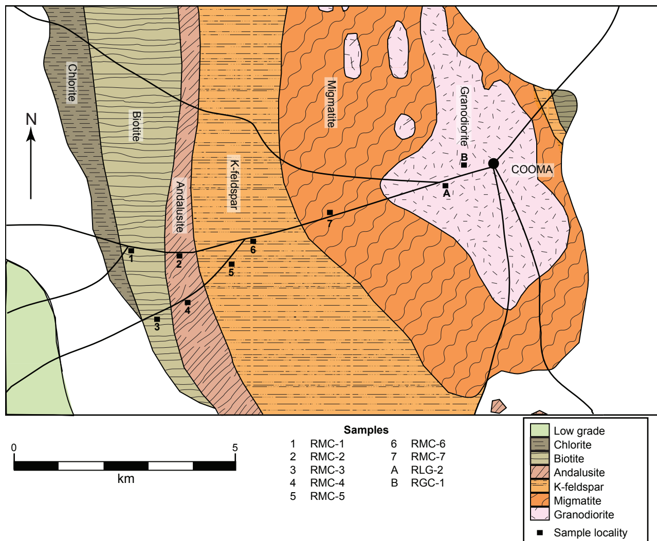
Figure 2. Enlargement of the area marked in Figure 1, showing an enlarged view of the regional metamorphic zones west of the Cooma granodiorite centered on the town of Cooma. The sample locations are shown along major roads.
