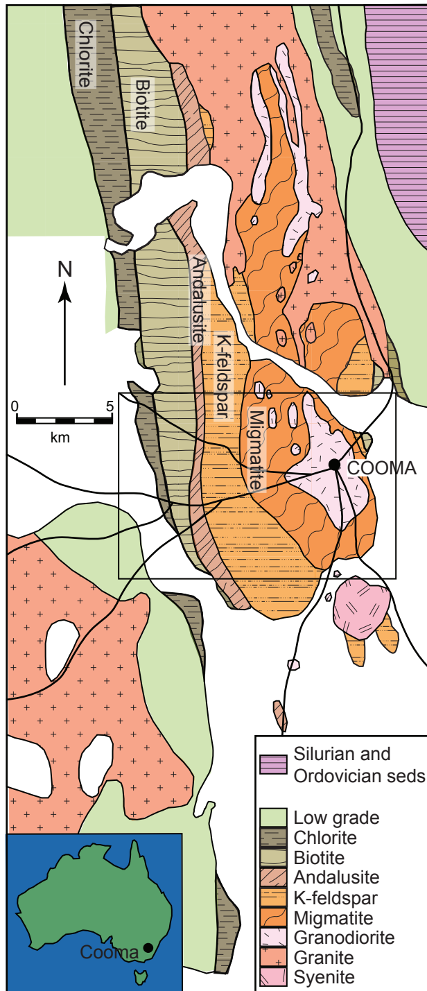
Figure 1. The Cooma metamorphic complex, southeastern Australia, showing the zones of regional metamorphism of increasing grade surrounding a central granodiorite, coinciding with the town of Cooma. The marked area is enlarged in Figure 2.
