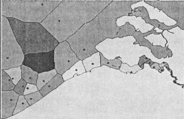
Figure 3.4. Stations proximities map by Thie-
