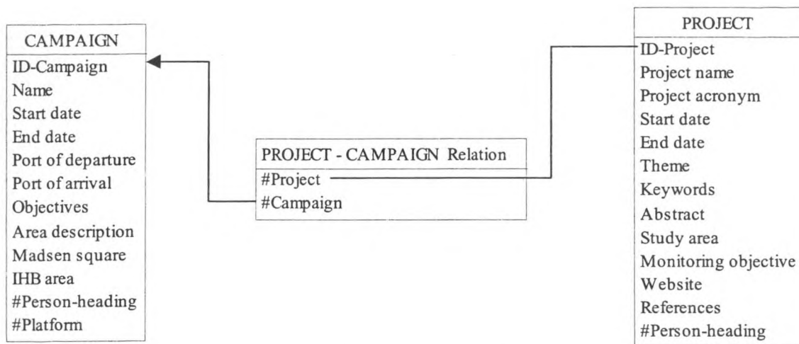
Figure 19. Logical datamodel.
