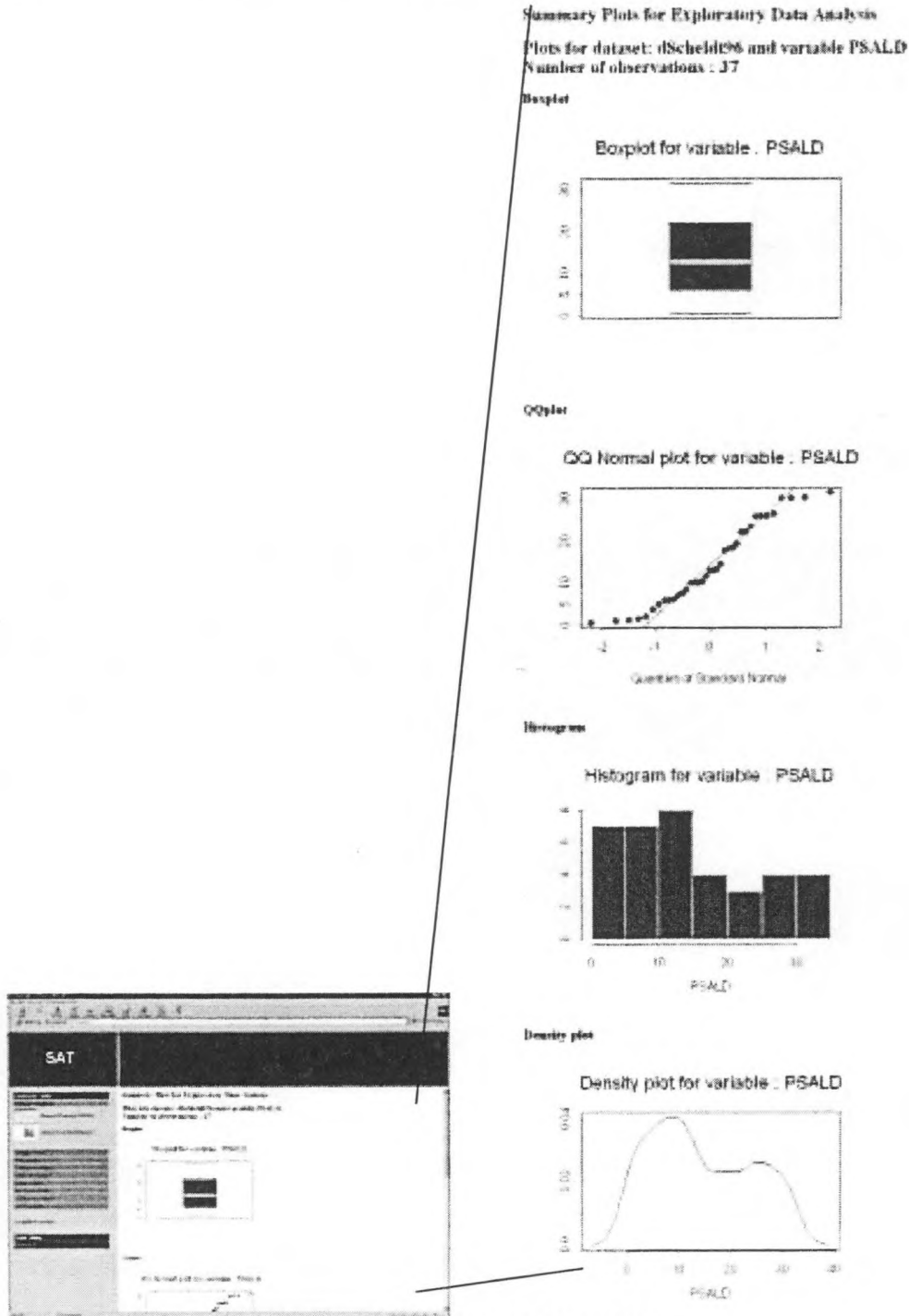
Figure 15: Example of the Graphical Summary Statistics function
