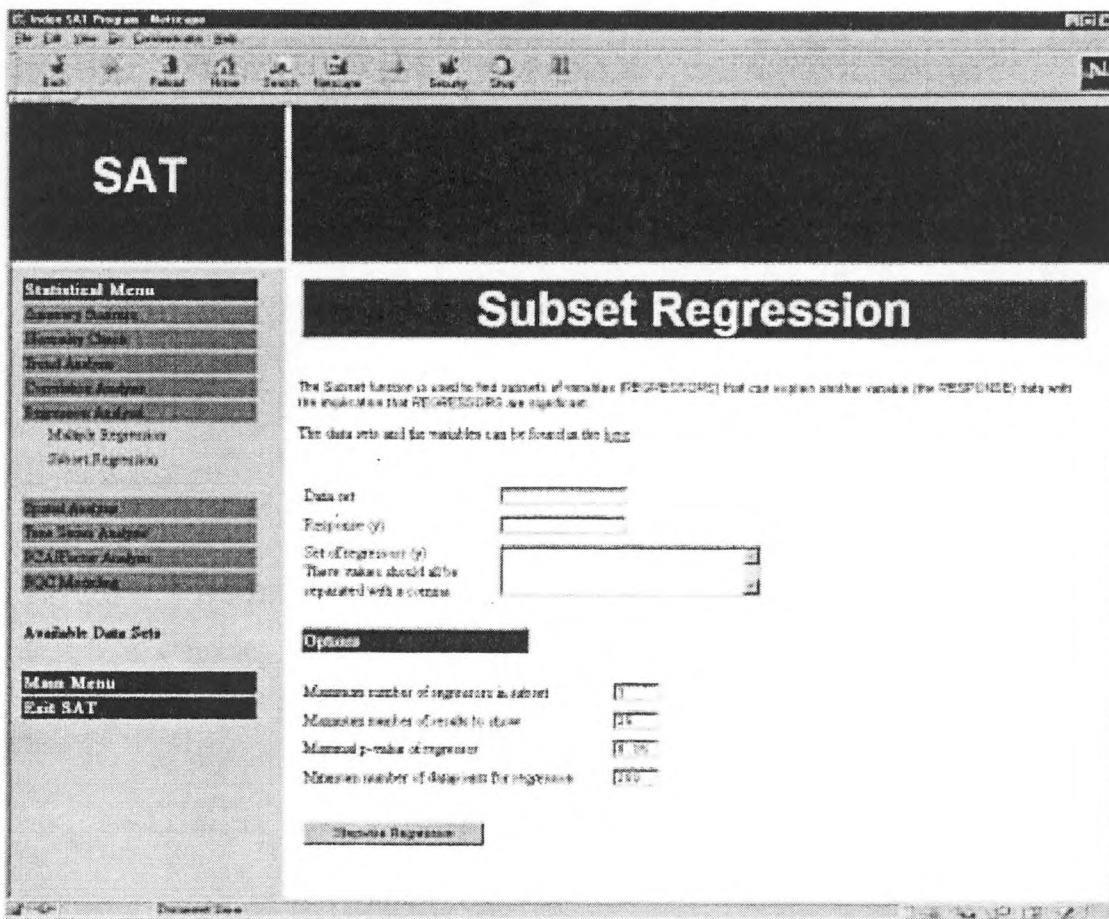
Figure 26: The subset regression function
