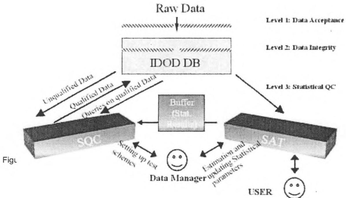
Figure 1: Overall QA-approach
