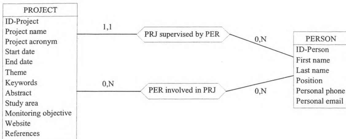
Figure 20. Conceptual datamodel.
