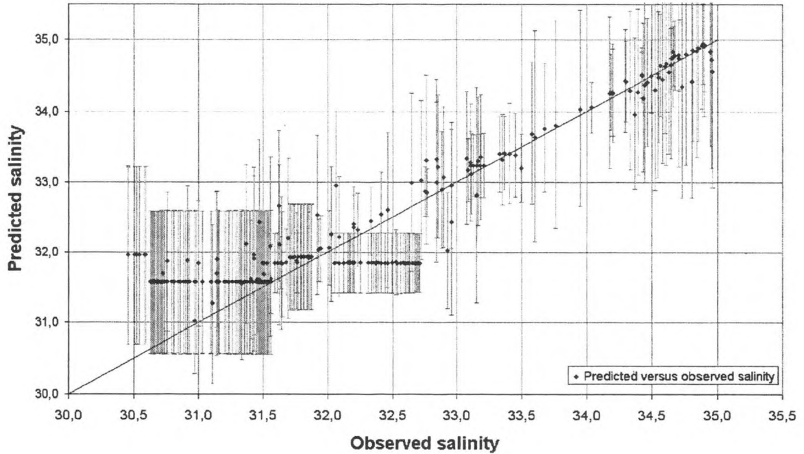
Predicted versus observed salinity and 95% confidence interval
