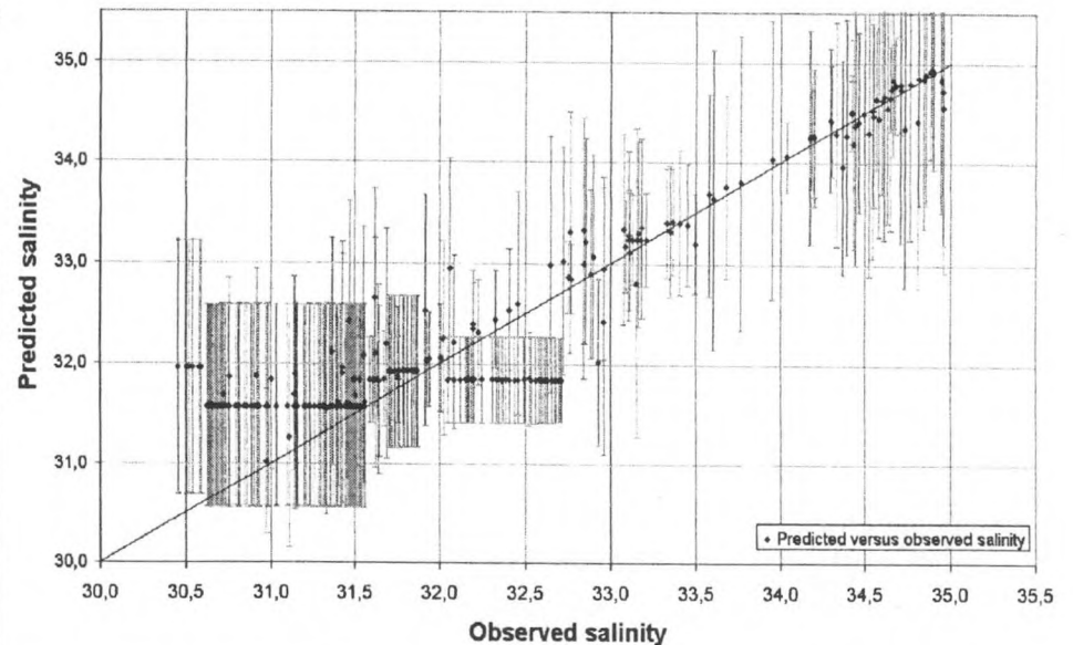
Predicted versus observed salinity and 95% confidence interval
