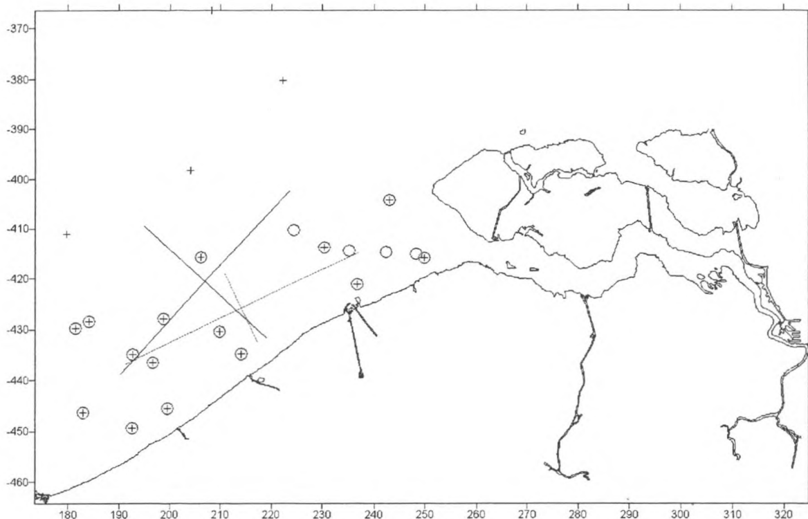
Main axes of the dispersion ellipses for the 9601 (black) and 9629 (red) campaigns
