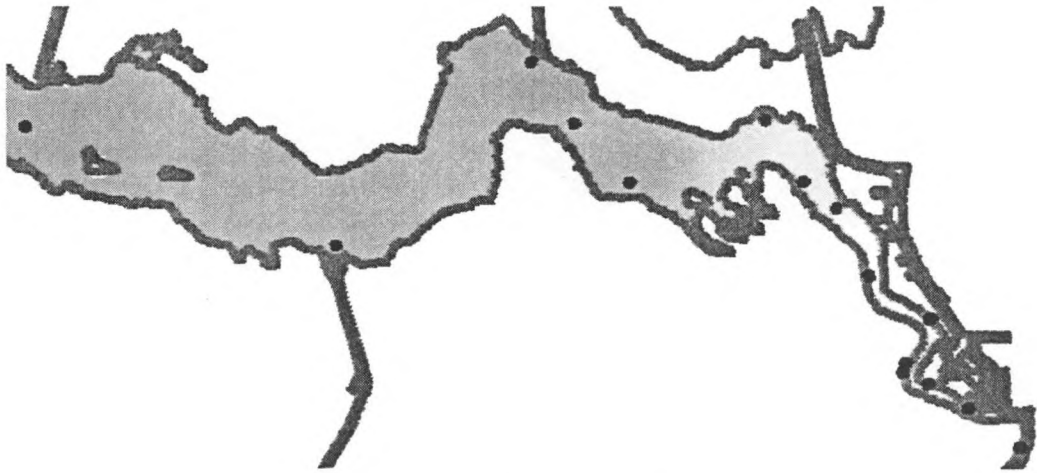
Inverse distance to power 2.
