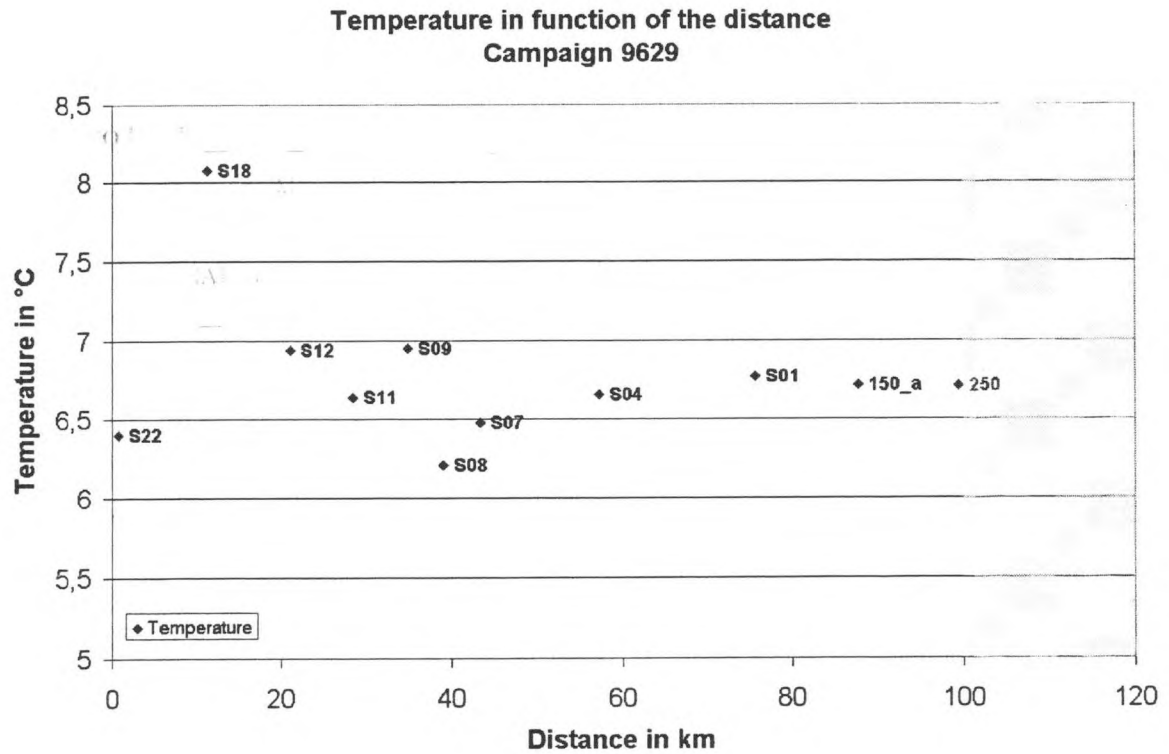
Figure 8: Temperature - distance scatter plot along the Scheldt estuary for the campaign 9629
