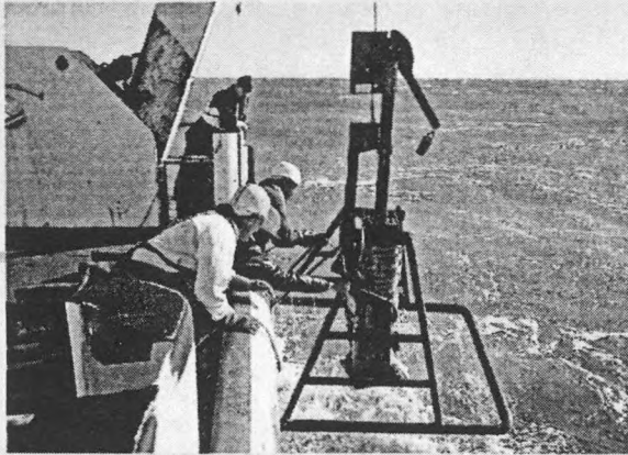
Sampling with boxcorer
