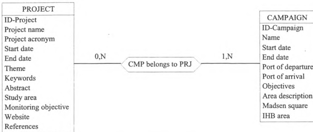
Figure 18. Conceptual datamodel.
