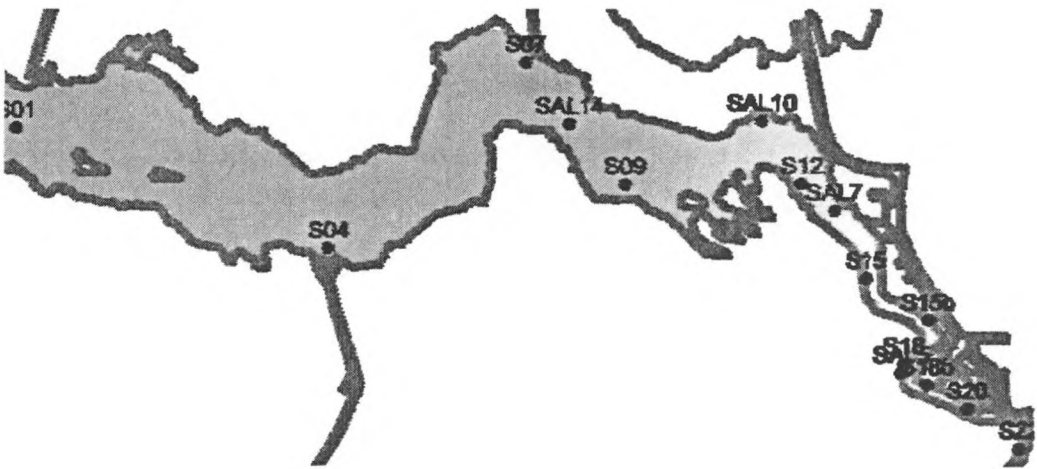
Kriging.
