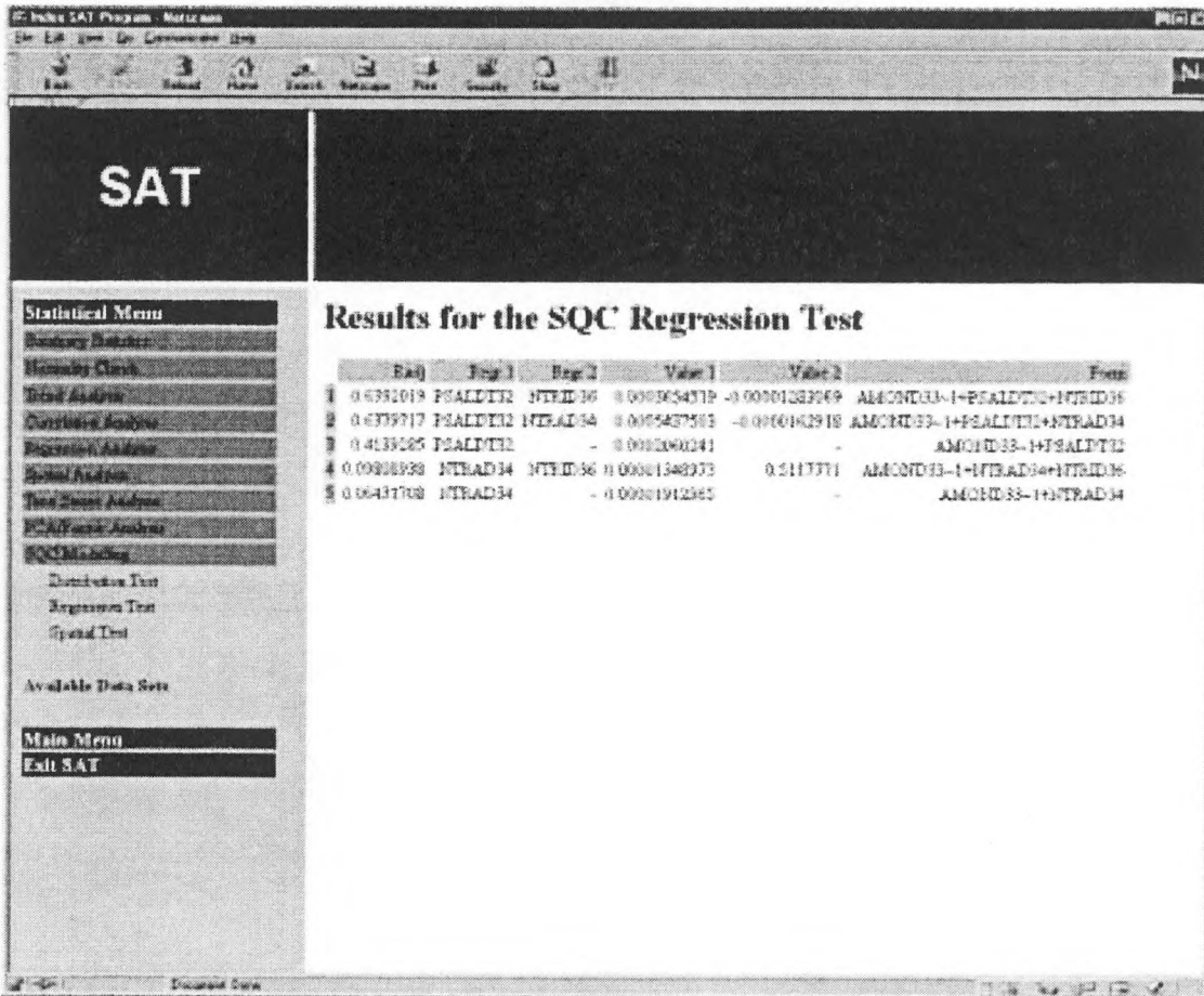
Figure 35: Example of the SQC Regression test
