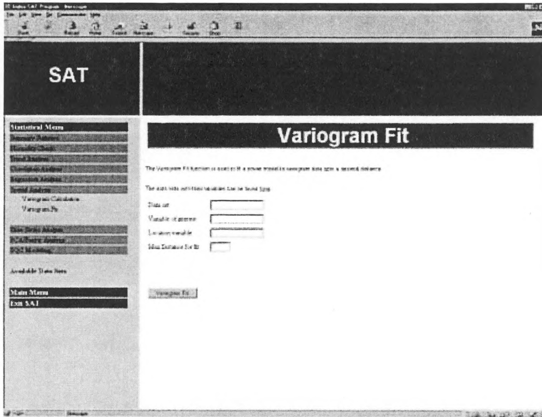
Figure 30: Variogram Fit function
