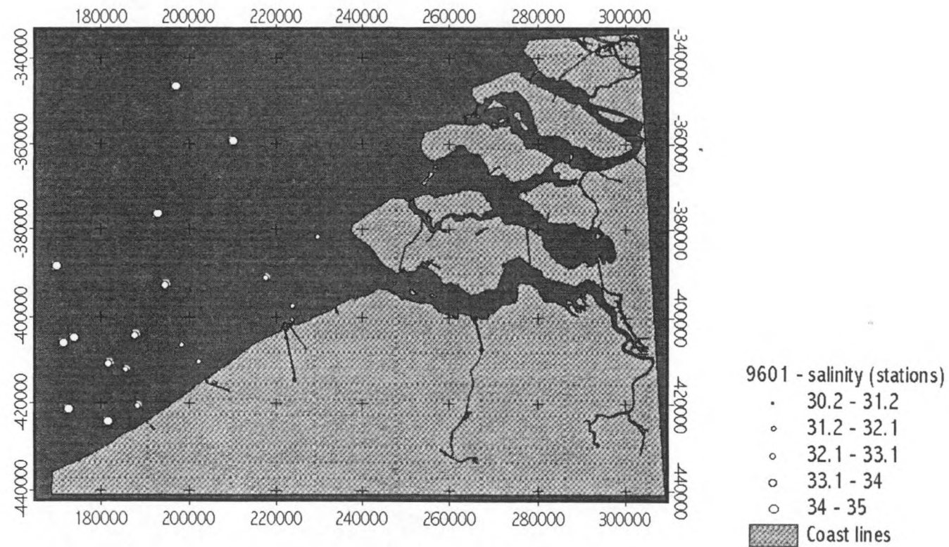
Campaign 9601 - data - salinity (stations)
