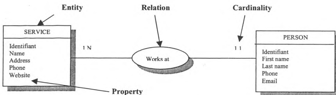
Figure 4. E/R formalism design.
