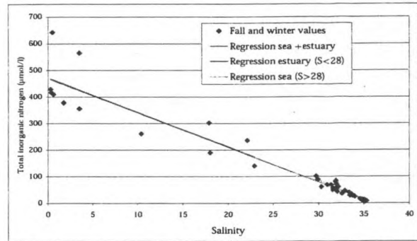
Figure 5.1. Regression of total inorganic nitrogen (Winter 1998)
