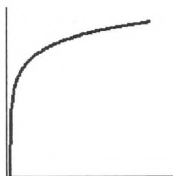
Logarithmic Model
