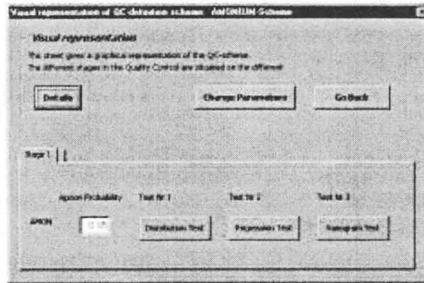
Figure 45: Visual representation of QC-scheme
