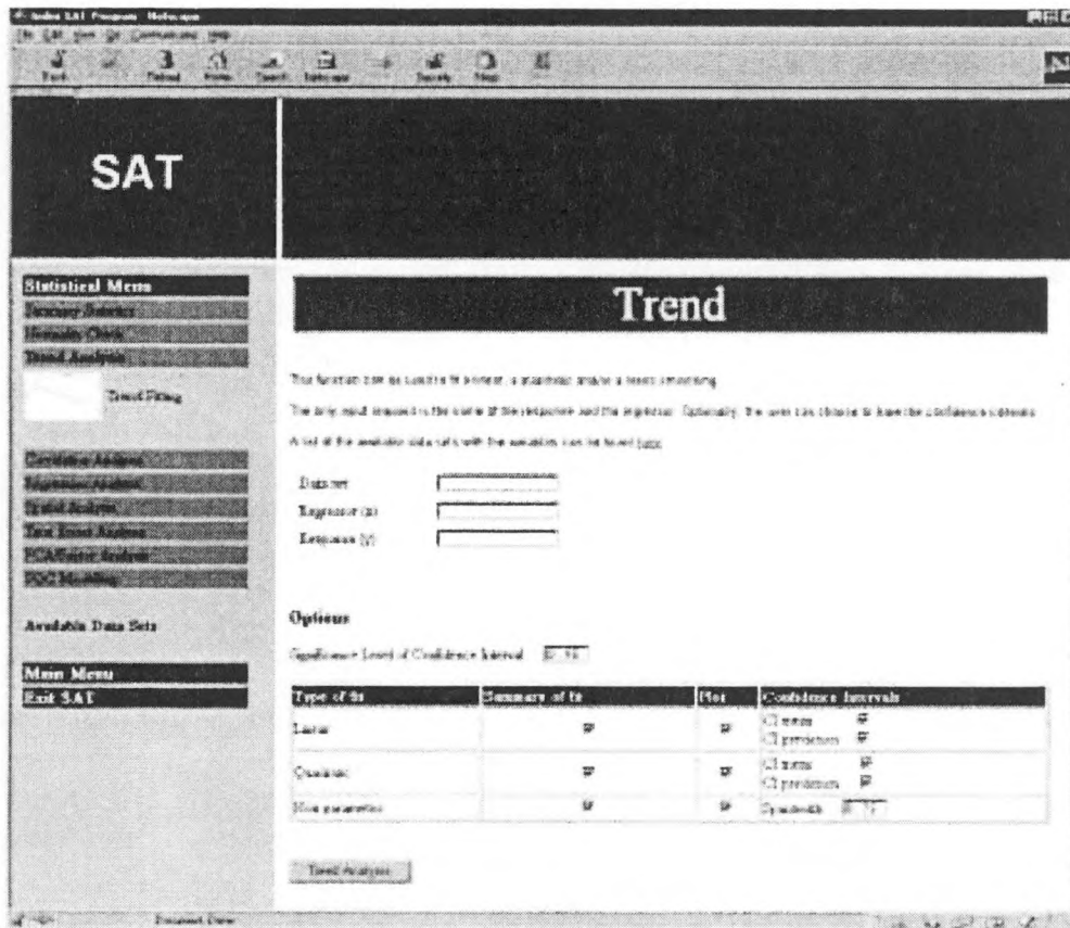
Figure 18: The trend fitting function
