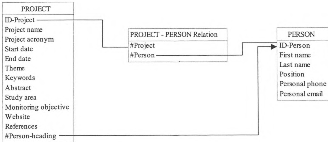
Figure 21. Logical datamodel.
