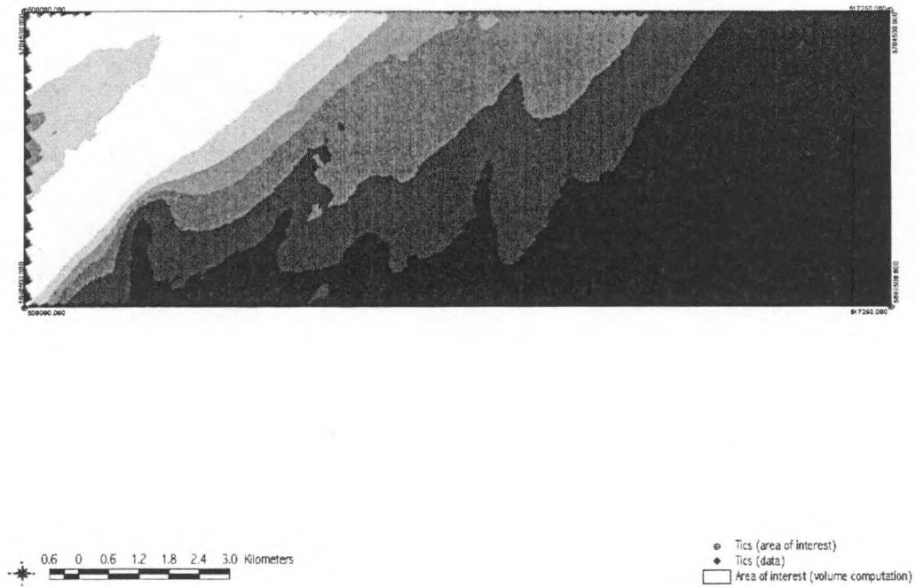
Figure 7 : LATTICE computed using a linear interpolation method with a 10 m resolution.
