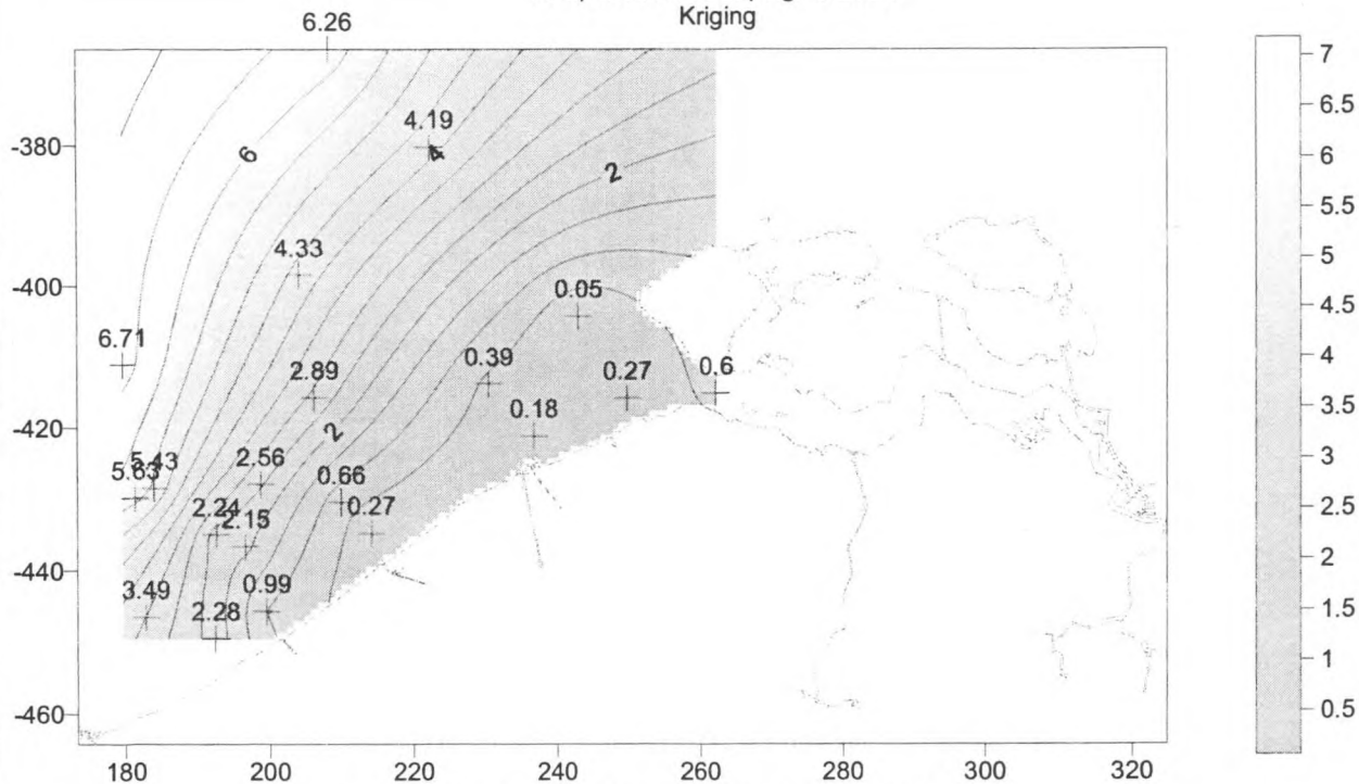
Figure 3.3. Map of sea temperatures by kriging.
