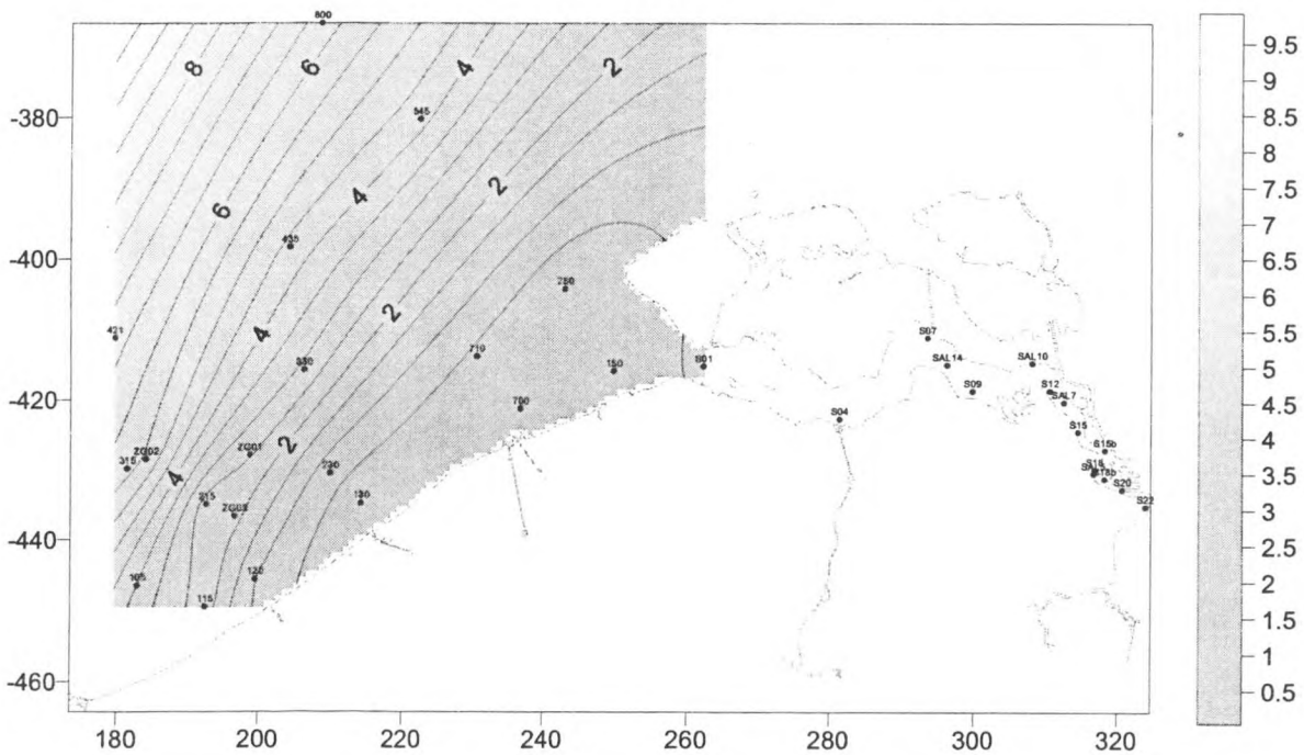
Temperature - Campaign BE96/1. Kriging
