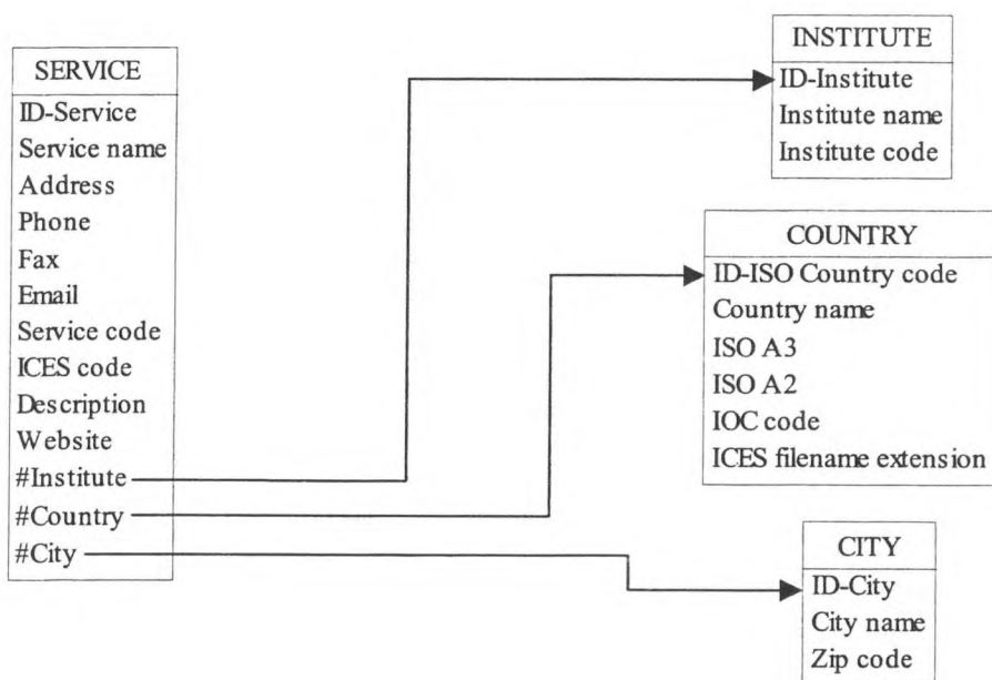
Figure 17. Logical datamodel.
