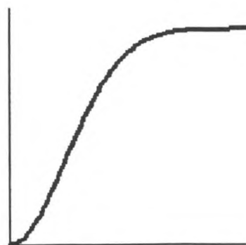
Gaussian Model
