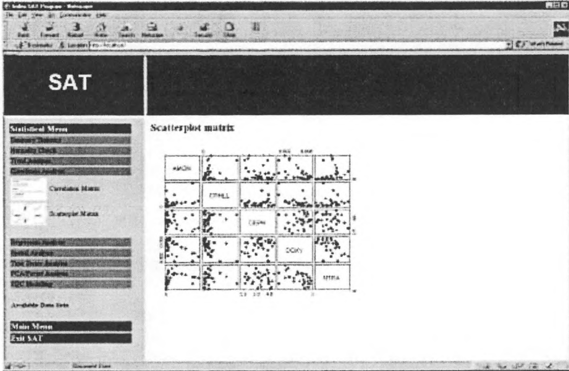
Figure 23: Example of the scatter plot matrix function
