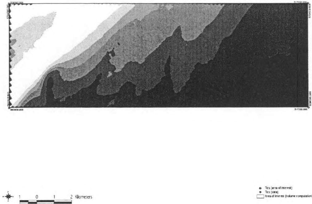
Figure 6 : LATTICE computed using a linear interpolation method with a 5 m resolution.
