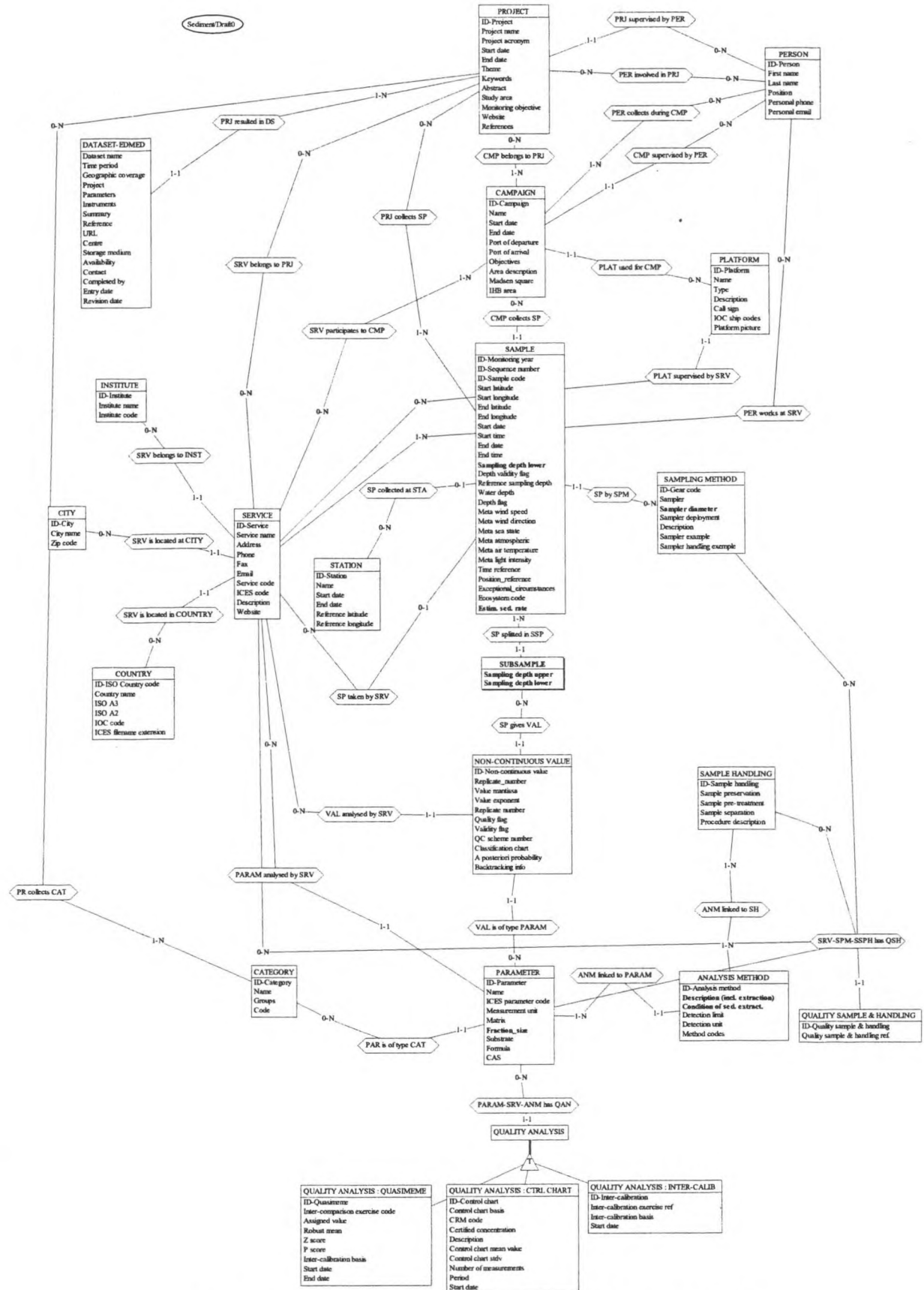
■ Figure 5. Conceptual scheme for sediment (Version Draft0)
