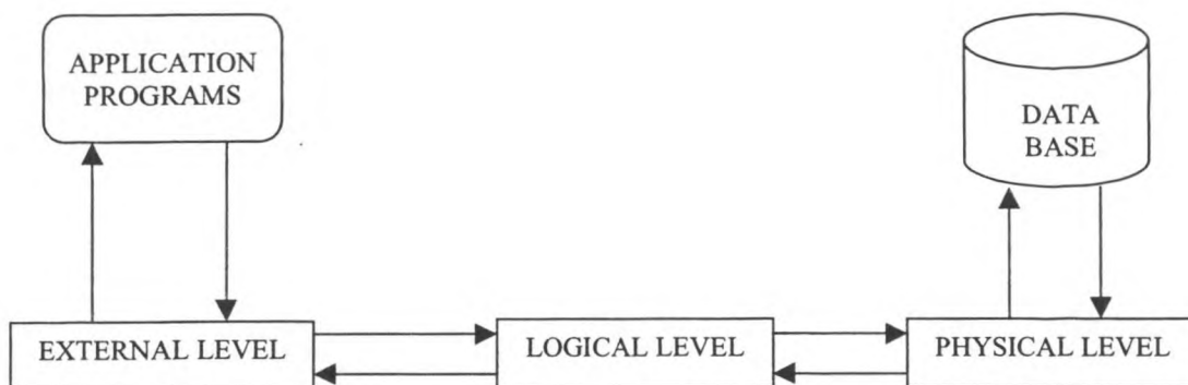
Figure 3. Access to a database through an application program.
