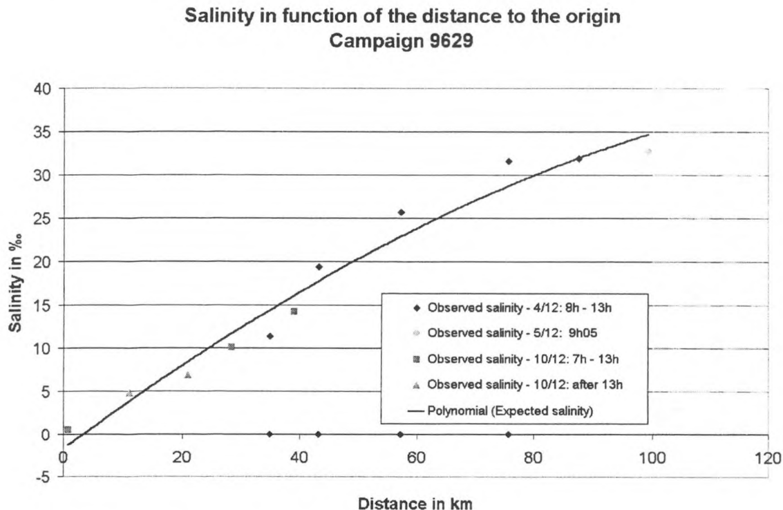
Figure 5: Salinity in function of the distance (campaign 9629)
