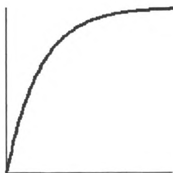
Exponential Model
