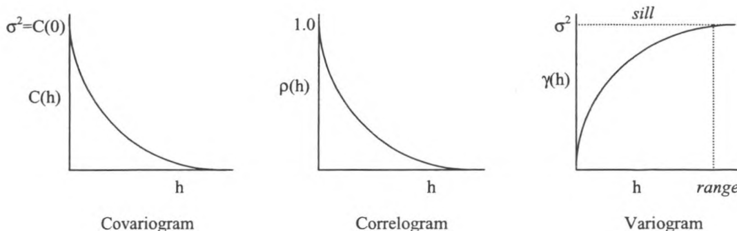
Figure 3. Covariogram, correlogram and variogram.
