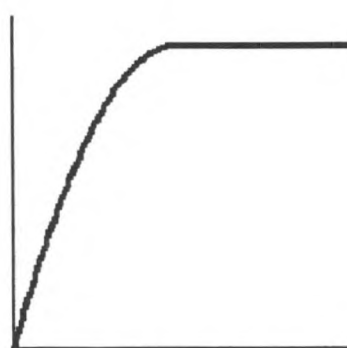
Quadratic Model
