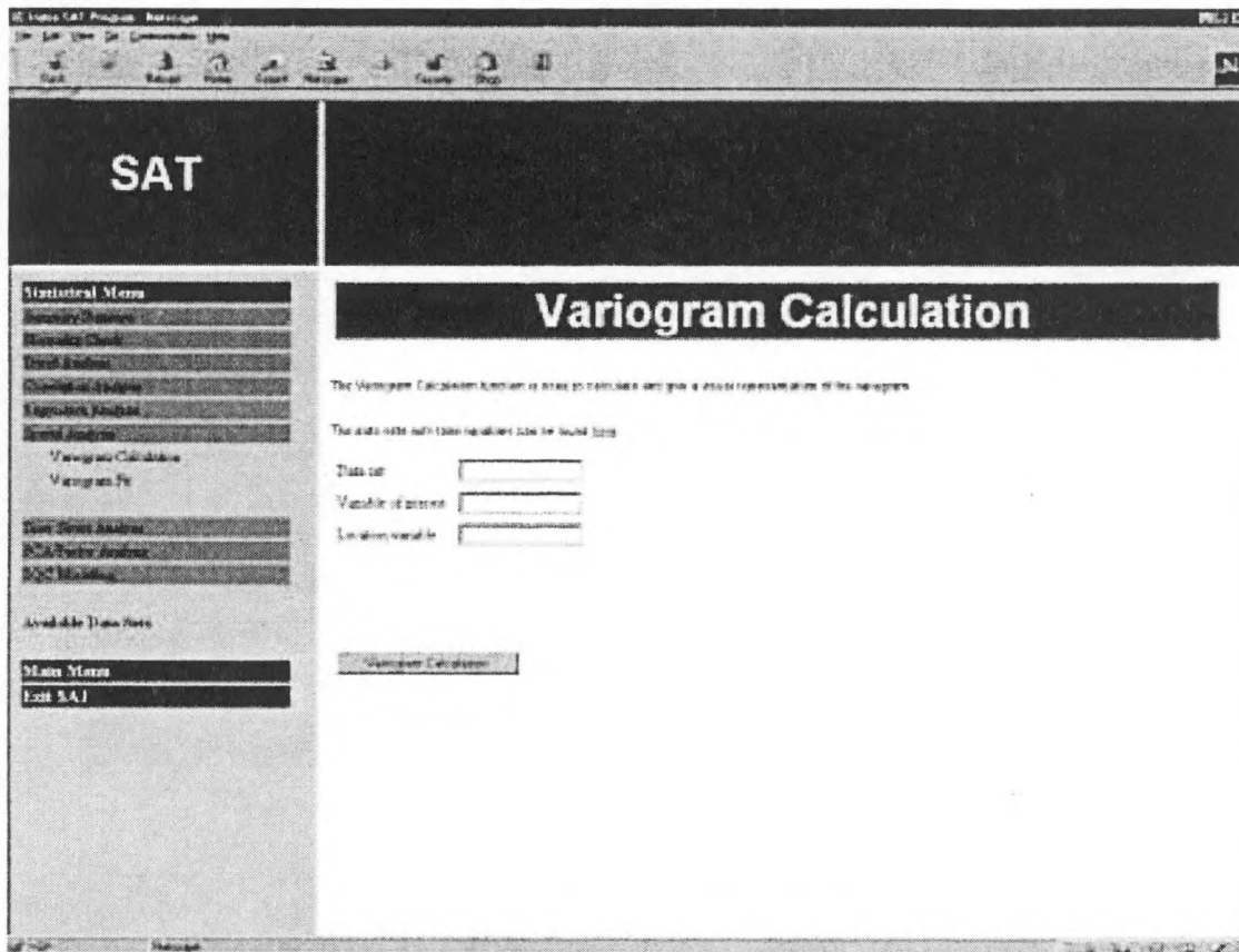
Figure 28: The Variogram Calculation Function
