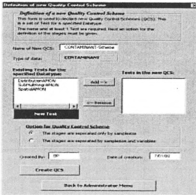
Figure 57: Definition of new Quality Control Scheme
