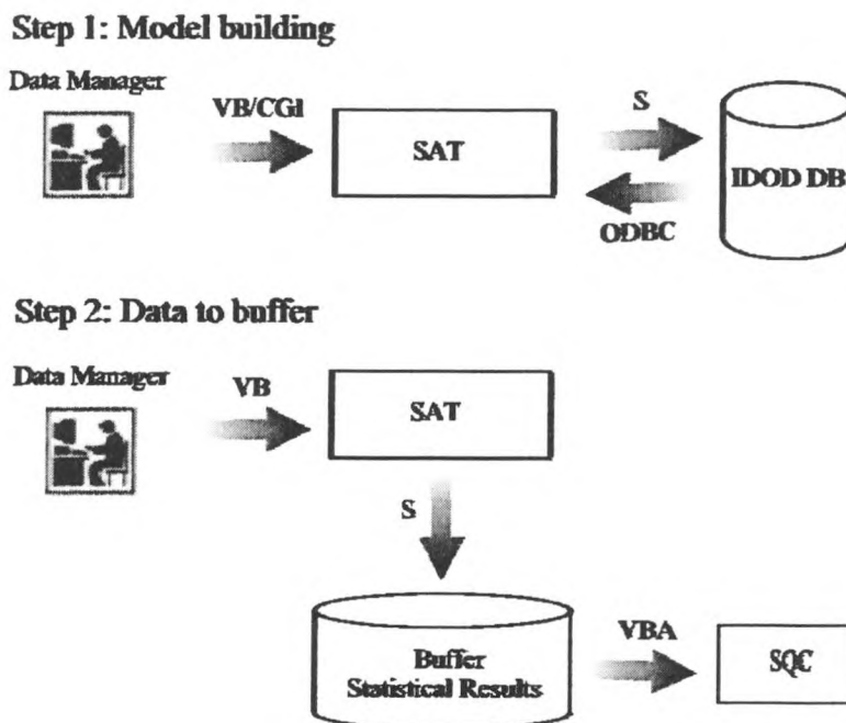
Figure 3: Methodology for the data manager to derive models
