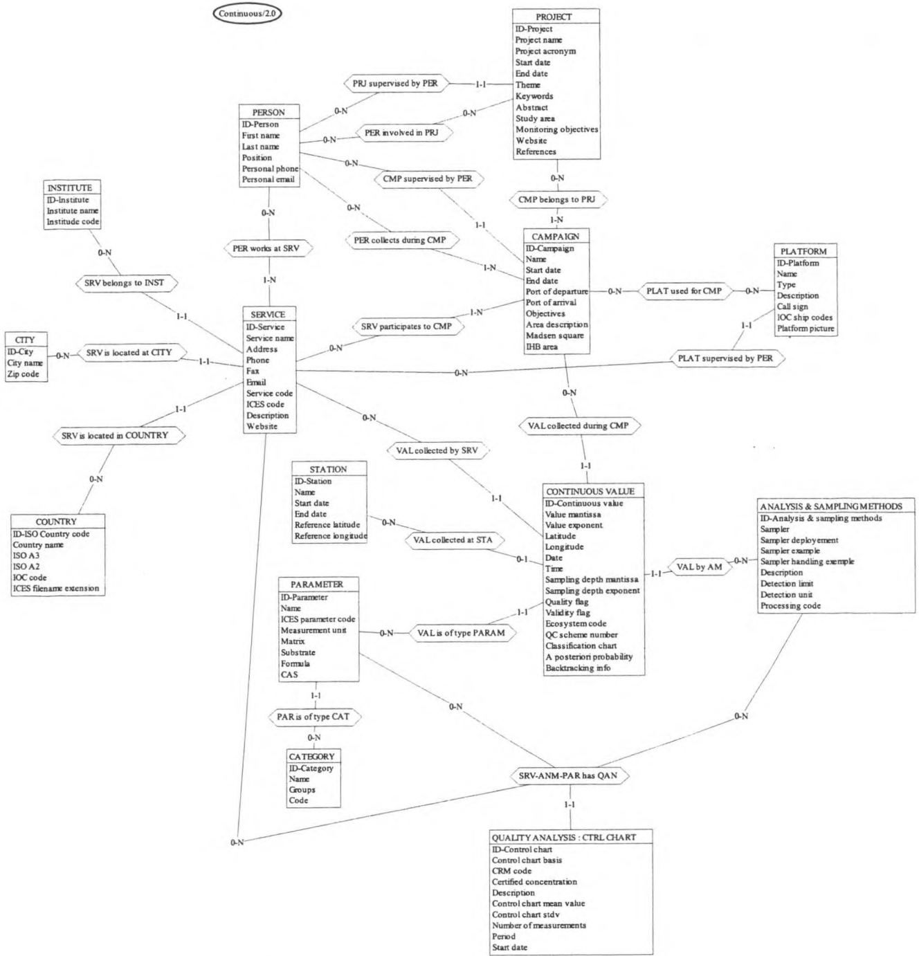
Figure 14. The conceptual datamodel for continuous values.
