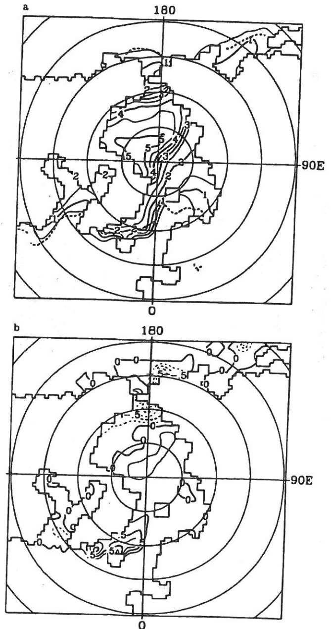
Fig. 2a,b. Ice thickness (in metres) for March in the Arctic. a Experiment OP; contour interval is 0.5 m. The dashed line represents the observed ice edge in March (Gloersen et al. 1992), defined as the 15% ice concentration. b OP minus CL; contour interval is 0.25 m
