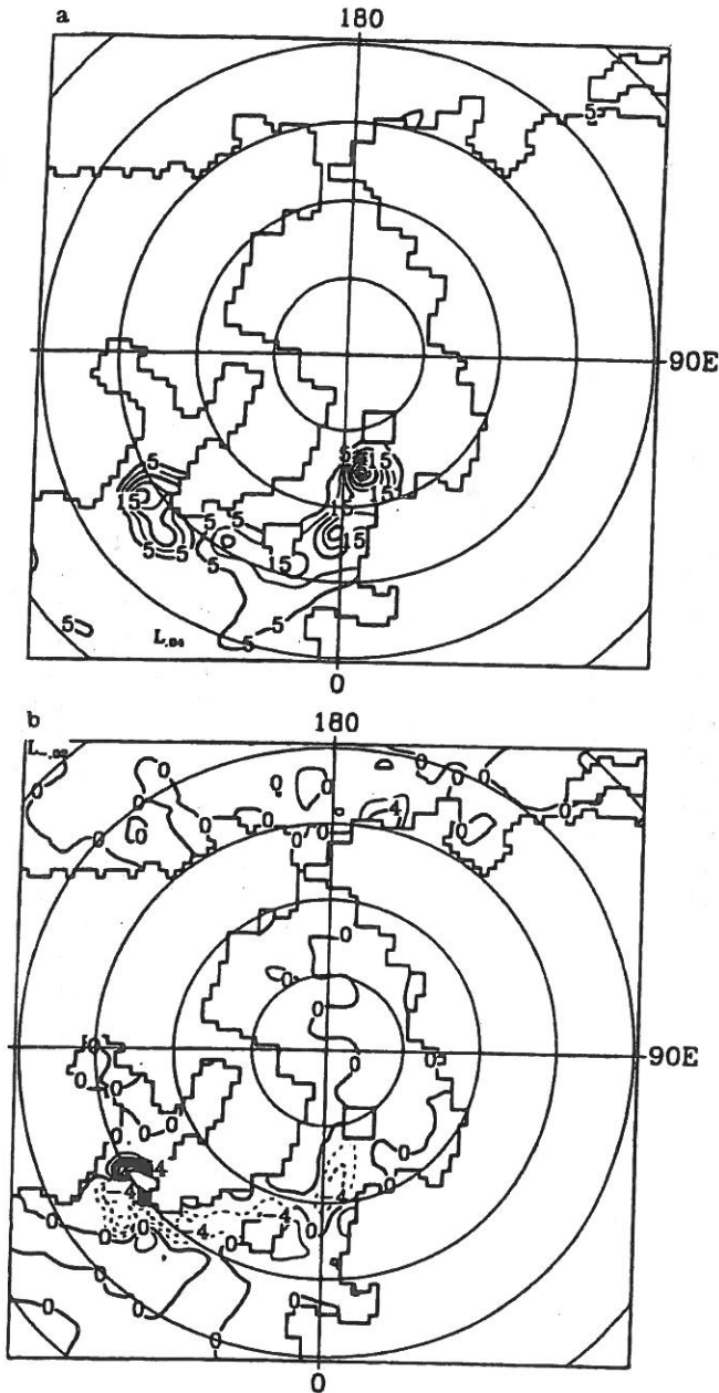
Fig. 4a, b. Energy dissipated by convective adjustment. a Experiment OP; contour interval is 5 \times 10^{-3} \text{ Wm}^{-2} . b OP minus CL; contour interval is 2 \times 10^{-3} \text{ Wm}^{-2}
