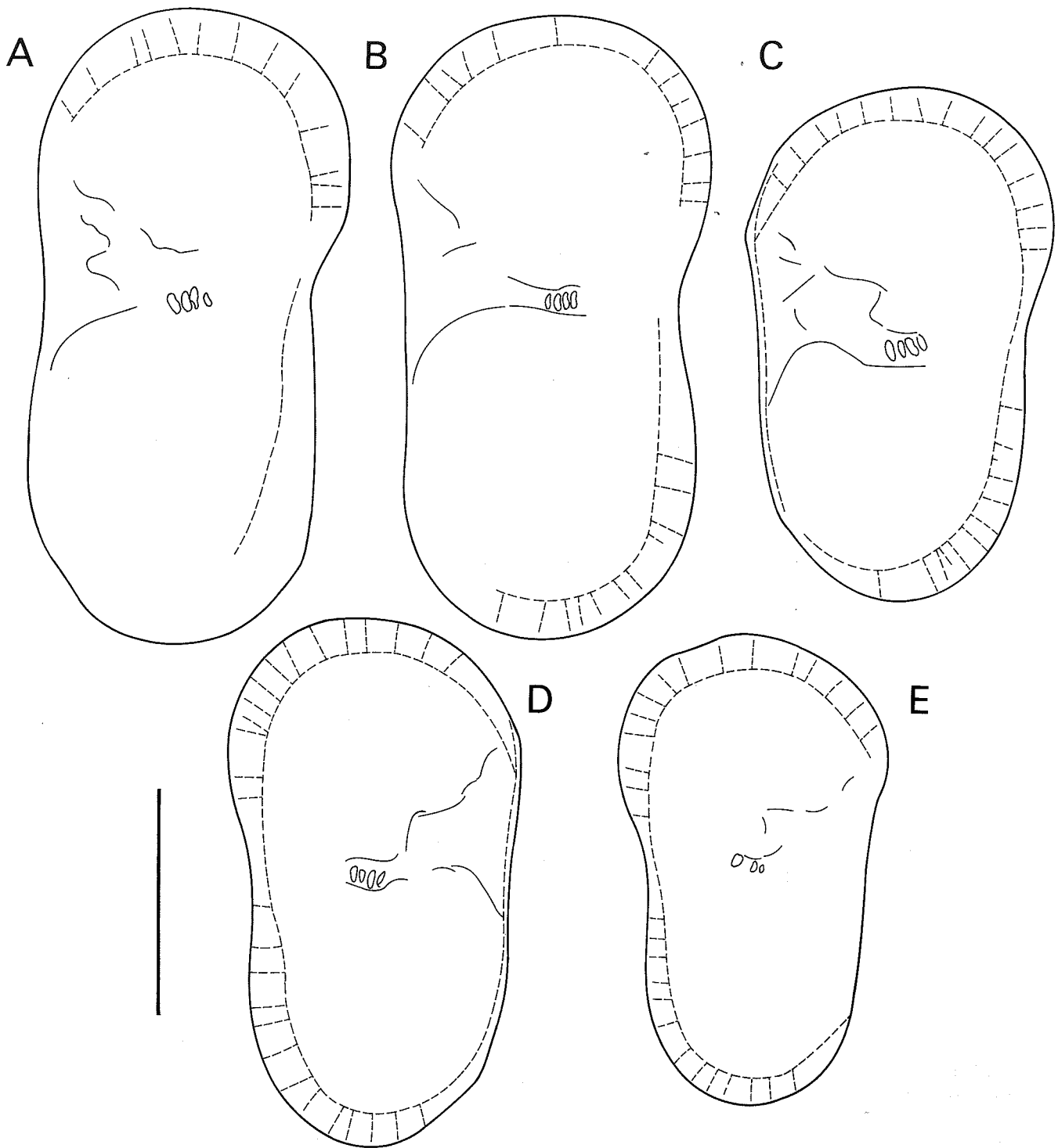
Figure 5. Leucocythere mirabilis KAUFMANN. External views of subfossil valves. A, B, E from site MO-7 at Mondsee, C, D, from site Weyregg at Attersee. A. ♂, RV. B. Idem. C. ♀, RV. D. ♀, LV. E. Last larval instar, LV, ♂. Scale = 333 \mu m for all figures.
