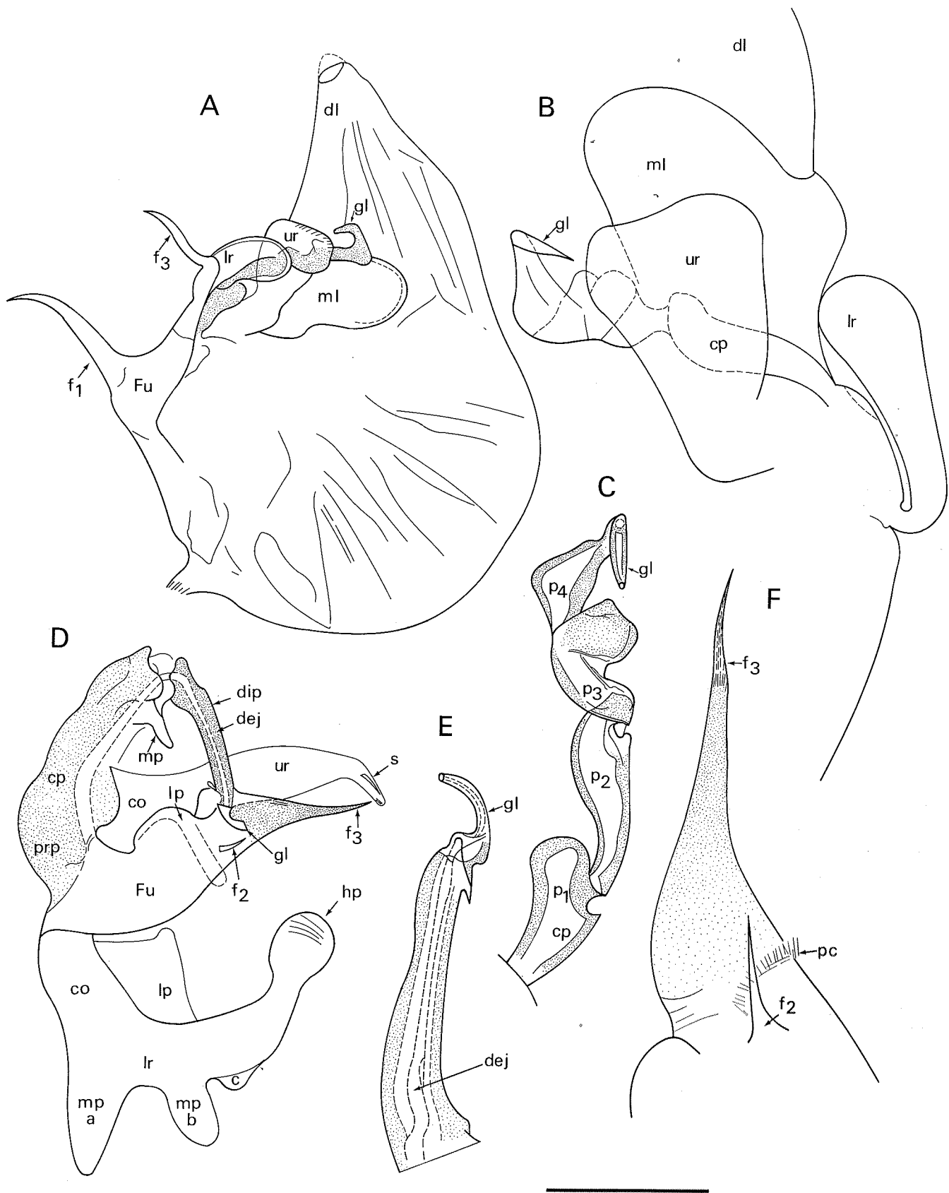
Figure 10. Leucocythere mirabilis KAUFMANN (A-C) and Limnocythere ( Limnocytherina ) sanctipatricii (BRADY & ROBERTSON) (D-F). Detail of hemipenis and male furcal anatomy. All specimens from Mondsee. L. mirabilis : A. Medial view of hemipenis. B. Details of co and copulatory process. C. Detail of copulatory process. L. (L.) sanctipatricii : D. Detail of copulatory complex, with co, copulatory process and furca. E. Detail of distal part of copulatory process. F. Detail of furca. Scale = 83 \mu m for A; 33 \mu m for B-E.
