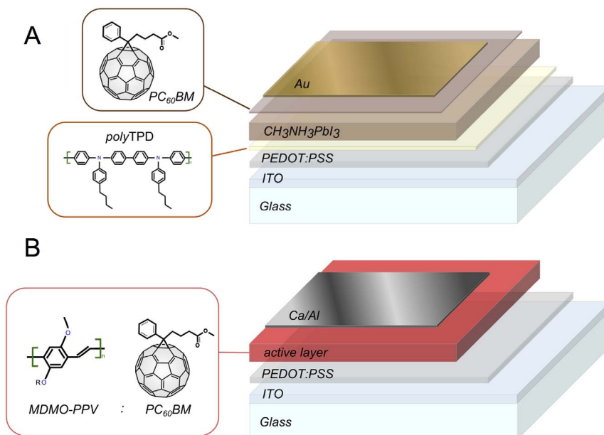
Figure 2 | Device layout of the studied solar cells. (A) Perovskite (MAPI) and (B) Organic (MDMO-PPV:PCBM) cells.
