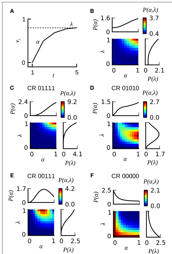
FIGURE 7 | The extended version of the Rescorla-Wagner model RW^{P(\alpha, \lambda)} . (A) The gradual increase of associative strength v_t across training trials in an individual animal is described by two parameters: the rate of learning \alpha and the asymptotic performance level \lambda . The probability for emitting a CR on a given trial is assumed to equal the associative strength. (B) Color-coded joint distribution P(\alpha, \lambda) of learning parameters of all animals from dataset 21. Most animals have high learning rates and high learning asymptotes. The inlets on the top and on the right side of the colored joint distribution depict the cumulative probability distributions P(\alpha) and P(\lambda) for which the joint distribution P(\alpha, \lambda) has been summed over lambda or alpha, respectively. (C-F) Color-coded likelihoods for observing a particular sequence of CRs given different combinations of \alpha and \lambda . The leftmost number of the CR sequence equals the CR in the first trial, and the rightmost number in the CR sequence equals the CR in the last trial.
