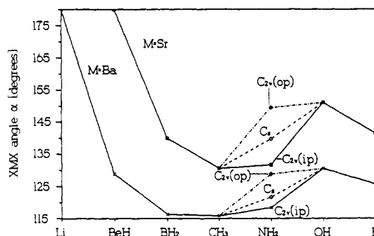
Figure 6. XMX angles for \text{SrX}_2 and \text{BaX}_2 compounds ( \text{X} = \text{Li}, \text{BeH}, \text{BH}_2, \text{CH}_3, \text{NH}_2, \text{OH}, \text{F} ). For \text{X} = \text{NH}_2 , points for structures with all hydrogen atoms in the NMN plane ( \text{C}_{2v}^p ), all hydrogens out-of-plane ( \text{C}_{2v}^o ), and two hydrogens out-of-plane ( \text{C}_2 ) are included (cf. Figure 1).
