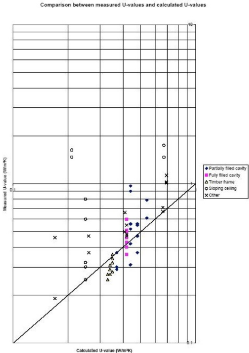
: A graph of measured U-value against calculated U-value shown for various construction types. Those points which lie above the diagonal line correspond to the measured U-value exceeding the calculated U-value whereas the points which lie below the line are cases where the measured U-value is less than predicted
