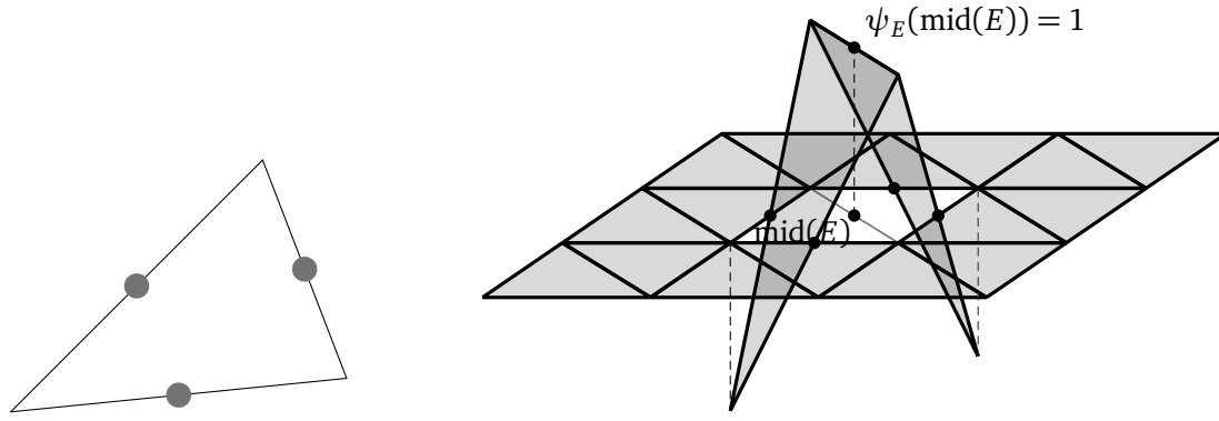
Figure 4.7: The CR_1 functions in \mathbb{R}^2 have three degrees of freedom. The values of the function can be chosen for the midpoints of the edges/faces (left). The figure on the right shows the CR_1 basis function \psi_E belonging to edge E (grey). The function is continuous in the midpoints of all edges.
