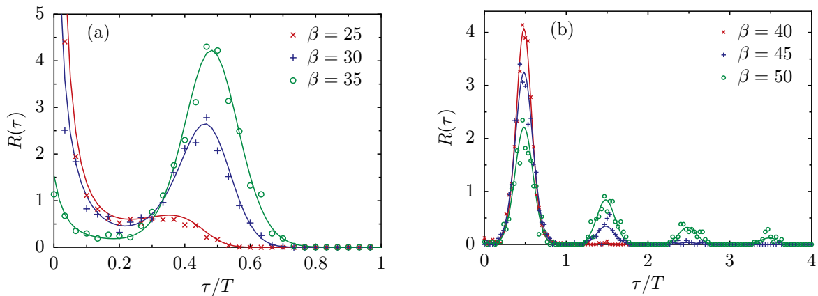
Figure 9. Residence time distributions for either of the two states are shown for \Omega = 10^{-4} and different values of the temperature. Theoretical results obtained from (eq. 31) are displayed as solid lines, estimates from the simulations as symbols. In panel (a) R(\tau) is shown for higher temperatures and in panel (b) for the optimal and lower than optimal temperatures. The peak structure and its temperature dependence is in complete agreement with previous findings, see Ref. [1].
