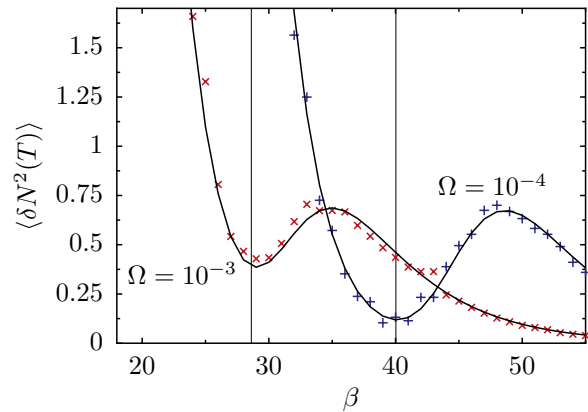
Figure 4. The variance of the number of transitions \langle \delta N^2(T) \rangle \equiv \langle \delta N^2(T, 0) \rangle in one period is shown as a function of the inverse temperature. The symbols are the same as in Fig. 2, the solid lines display equation (22). Note that \langle \delta N^2(T) \rangle is proportional to the diffusion constant of the Rice phase. The vertical thin black lines indicate the optimal inverse temperatures as found from the synchronization of the averaged phase (see Fig. 2). They coincide remarkably well with the positions of the minima of \langle \delta N^2(T) \rangle . So we find that at the optimal temperature also the fluctuations of the number of transitions and consequently of the generalized Rice phase are suppressed.
