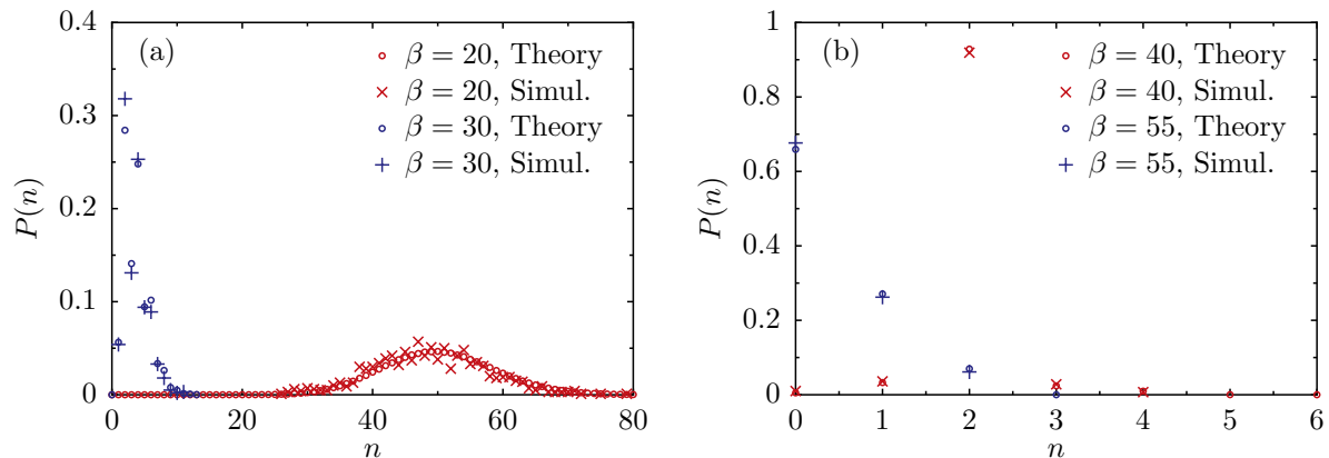
Figure 6. The probabilities P(n) = P(n; T, 0) are shown for the driving the driving strength A = 0.1 and the driving frequency \Omega = 10^{-4} ; for two temperatures that are higher than the optimal one corresponding to \beta \approx 40 in panel (a) and and for the optimal and a lower temperature in panel (b). As one expects for a good synchronization of the system with the driving force at the optimal temperature one finds two transitions per period with about 90% of the total weight. For high temperatures the distribution becomes rather broad with a maximum at some large number of transitions. On the contrary, for low temperatures the probability is largest at n = 0 and decreases with n . The agreement of the two-state theory resulting from equation (30) with the simulations is remarkably good.
