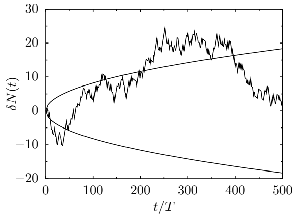
Figure 3. The fluctuations of the number of transitions \delta N(t) for A = 0.1 , \Omega = 10^{-3} and \beta = 35 (jagged line) appears as diffusive. The smooth curve depicts the root behavior of the diffusion law \langle \delta N^2(t) \rangle = 2D(0)t with the diffusion constant D(0) = \langle \delta N^2(T, 0) \rangle / (2T) = 5.36 \times 10^{-5} resulting from the two-state model, see eq. (25).
