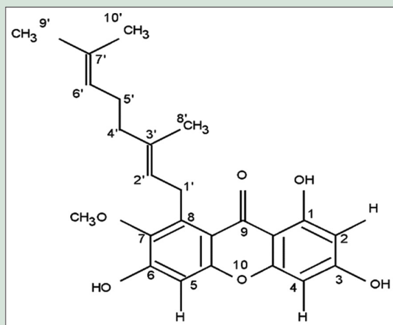
Figure 1: Rubraxanthone
