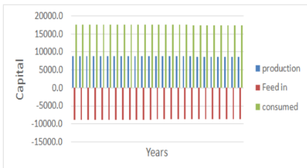
Figure 6: The PV production, the electricity consumption and the electricity feed-in with 50% capacity
