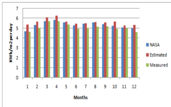
Figure 1: The Solar Radiation in Brunei
