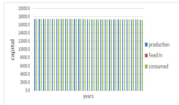
Figure 7: The PV production, the electricity consumption and the electricity feed-in with 100% capacity
