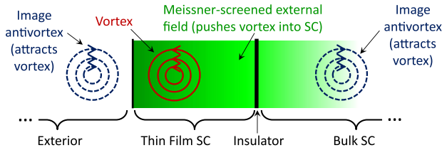
FIG. 3. Forces on a vortex in a homolaminate. As the film is made thinner, the image antivortex to the right of the film has a stronger pull on the vortex, lowering the barrier to vortex penetration.
