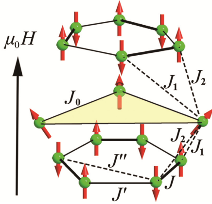
Fig. 1: Schematic view of the spin cluster V15 with \mu_0 \mathbf{H} being the external magnetic field. Exchange couplings between the spins are shown and reported in text. The central spin triangle is highlighted.
