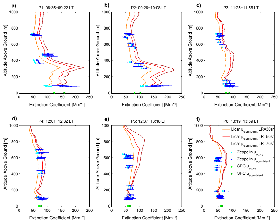
Figure 8. Extinction coefficients for profiles P1–P6 at different times of day. The lines reflect LIDAR results for assumed LRs of 30, 50 and 70 sr in orange, red and dark red, respectively. The dots describe in-situ results. In light and dark blue, dry and ambient airborne extinction coefficients are shown while the light and dark green dots represent the dry and ambient ground based results, respectively.
