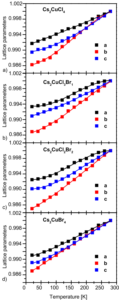
FIG. 3: (Color online) Normalized lattice parameters for a) \text{Cs}_2\text{CuCl}_4 , b) \text{Cs}_2\text{CuCl}_3\text{Br}_1 , c) \text{Cs}_2\text{CuCl}_2\text{Br}_2 , and d) \text{Cs}_2\text{CuBr}_4 , plotted as l_i(T)/l_i(280\text{ K}) . The size of each point exceeds the statistical error. The T -dependence was fitted with a third-order polynomial function (solid lines), which were used to calculate the coefficients of the thermal expansion.
