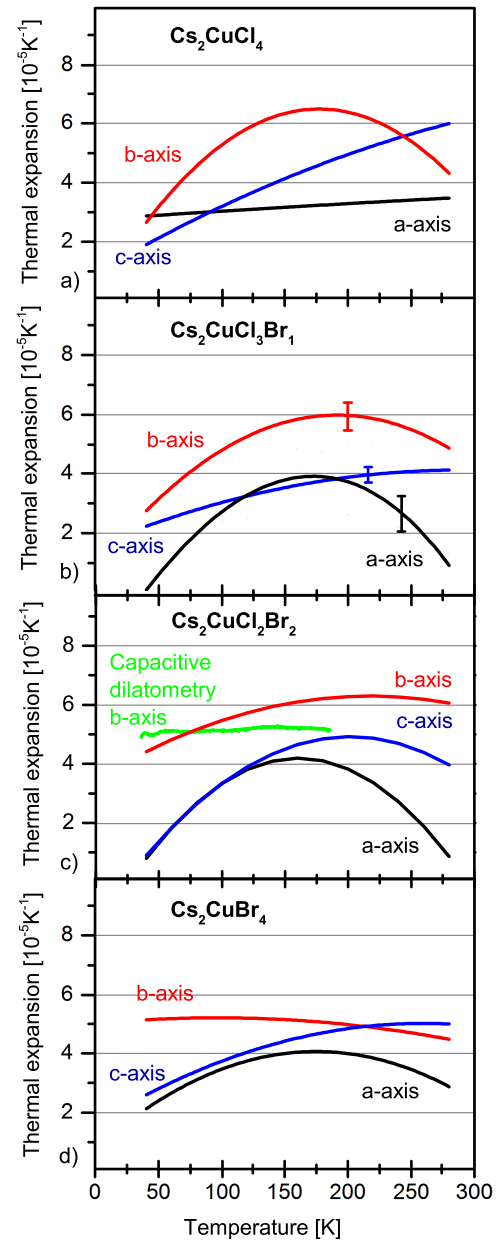
FIG. 4: (Color online) T -dependence of the linear thermal expansion coefficients for a) \text{Cs}_2\text{CuCl}_4 , b) \text{Cs}_2\text{CuCl}_3\text{Br}_1 , c) \text{Cs}_2\text{CuCl}_2\text{Br}_2 , and d) \text{Cs}_2\text{CuBr}_4 . Typical errors correspond to the error bars shown in b). The thermal expansion coefficients show a pronounced anisotropy for the three different crystal directions a, b, c and vary considerably with x . For x = 2 , we compare the data determined from the lattice parameters data with dilatometry data.
