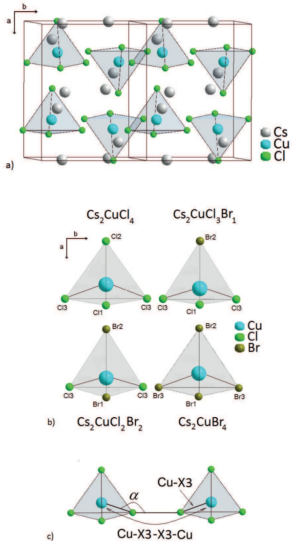
FIG. 5: (Color online) a) Crystal structure for x = 0 with the [\text{CuX}_4] -tetrahedra for two neighboring unit cells along the b -direction. b) [\text{CuX}_4] -tetrahedron for the four investigated compositions calculated from the PXRD data at 20 K. All tetrahedra are shown in the ab plane and are normalized to their height. b) Designation of the magnetic exchange path between two consecutive [\text{CuX}_4] -tetrahedra along the b -direction with the angle \alpha as well as the Cu-X3 and Cu-X3-X3-Cu distances used in Table III.
