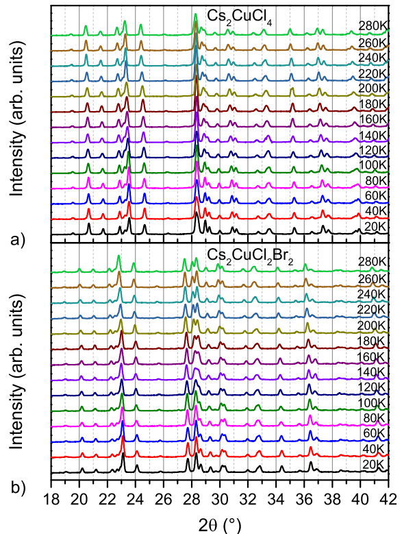
FIG. 2: (Color online) PXRD data from 280 to 20 K exemplarily shown for a) \text{Cs}_2\text{CuCl}_4 and b) \text{Cs}_2\text{CuCl}_2\text{Br}_2 . No structural phase transition for any of the materials was observed between 280 and 20 K. The high quality of these data allows for the determination of the thermal expansion coefficients.
