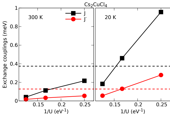
FIG. 6: (Color online) Spin exchange couplings for \text{Cs}_2\text{CuCl}_4 determined with density functional methods using two different sets of structural data, obtained at 300 and 20 K. Dashed lines denote the experimental findings for J and J' . 1
