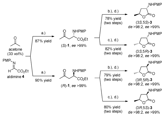
Scheme 2 Synthesis of all four diastereomers of PMP-protected \alpha -amino- \gamma -butyrolactone 3 through combination of organo- and biocatalysis. Reagents and conditions : (a) D- L -proline (0.25 eq.), DMSO, 3 h, rt; (b) ( R )-/ (S) - 1 (30 mM), ADH-A, NAD + , buffer (100 mM, pH 6.3), 2-PrOH (10 vol%), 30 °C, 24 h; (c) ( R )-/ (S) - 1 (50 mM), evo-1.1.200, NAD + , buffer (100 mM, pH 6.3), 2-PrOH (30 vol%), 30 °C, 24 h; (d) HCl-Et 2 O (2.0 eq.), MeOH, 16 h, rt. PMP = para -methoxyphenyl.
