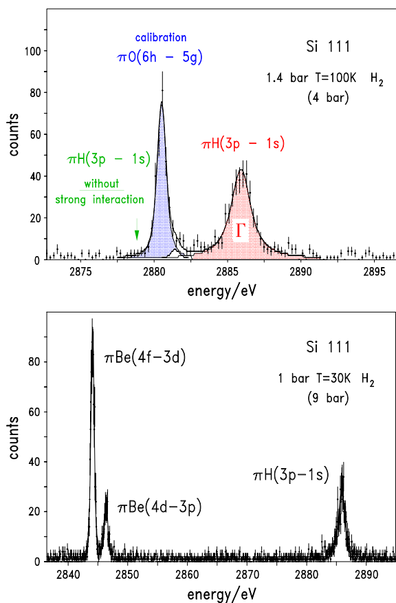
Fig. 4. Spectra from simultaneous measurements of the \pi H(3p-1s) transition and the \pi^{16}O(6h-5g) (top) and the \pi^{16}Be(4f-3d) calibration lines (bottom).
