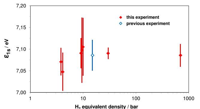
Fig. 6. Results for the hadronic ground-state shift \epsilon_{1s} in pionic hydrogen at various \text{H}_2 densities ( \blacklozenge ). The open diamond ( \diamond ) represents the weighed average of the previous precision experiment [67] when also using the new value for the electromagnetic transition energy. Note the logarithmic scale for the density.
