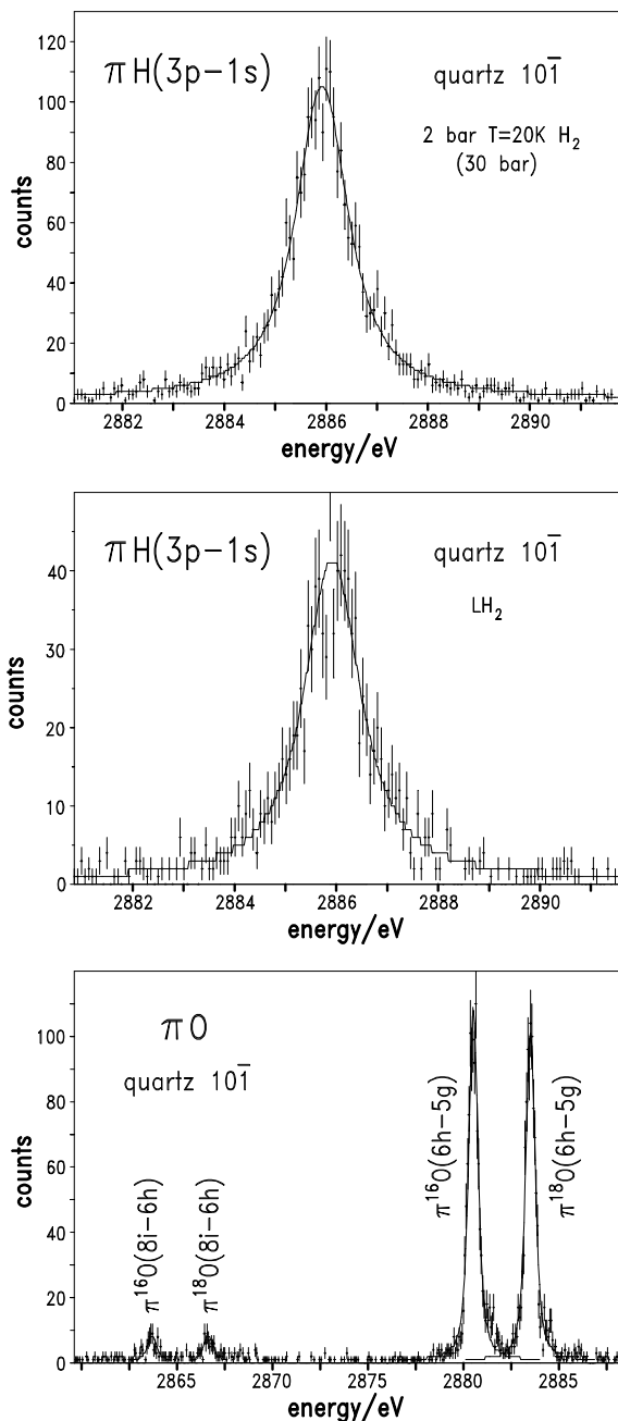
Fig. 5. High statistics measurement of the \pi H(3p-1s) transition (top), first crystal spectrometer measurement in liquid hydrogen (middle), and energy calibration with (6-5) transitions from an ^{16}O_2/^{18}O_2 mix target at 4 bar equivalent density with an 80% He admixture. Also visible are the inner transitions (8i-6h) of the oxygen isotopes having energies of 2863.689 and 2866.652 eV.
