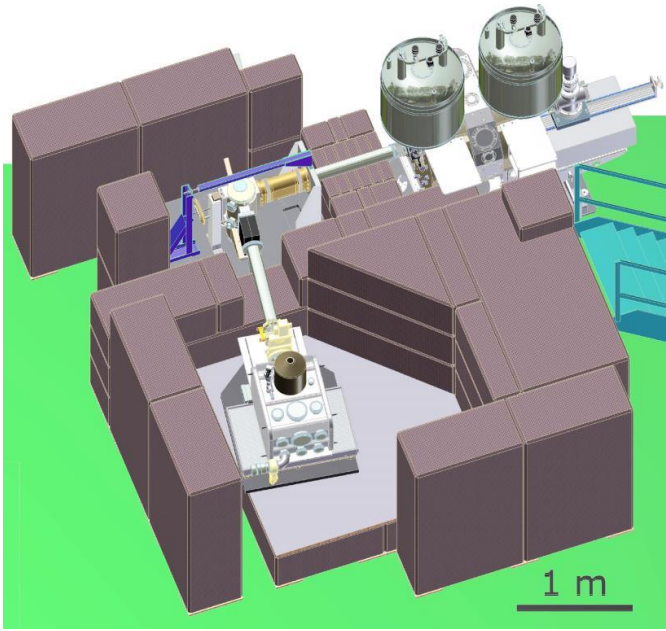
Fig. 2. Set-up of cyclotron trap (top right) and crystal spectrometer in the \pi E5 area at PSI for the \pi H(3p - 1s) (quartz 10\bar{1} ) and the \pi H(4p - 1s) transition (silicon 111). The roof of the concrete cave is not shown.
