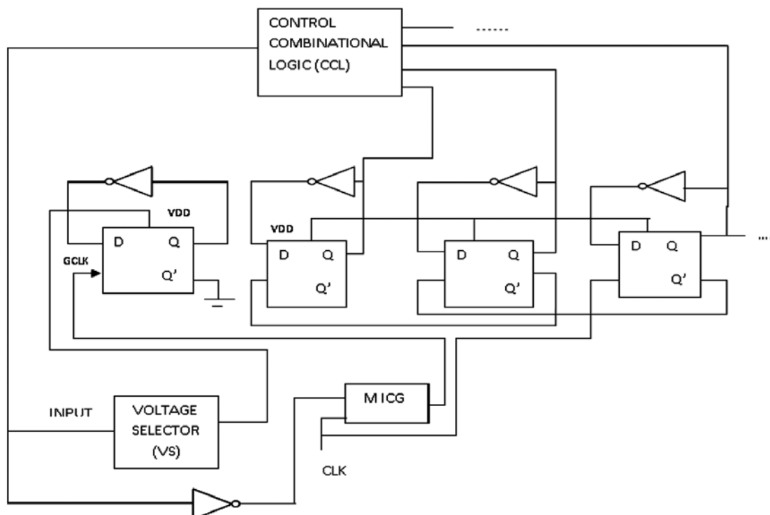
Fig. 1 — Modified Architecture.
