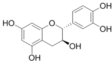
Fig. 1 — Structure of Catechin
