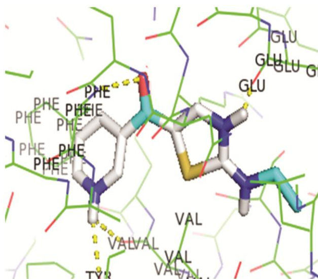
Fig. 4 — Docking image of 3-(2-ethylaminothiazol-5-yl)pyridine (6a)
