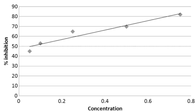
Fig. 5 — Plot of % inhibition vs concentration of 3-(2-ethylaminothiazol-5-yl)pyridine (6a)
