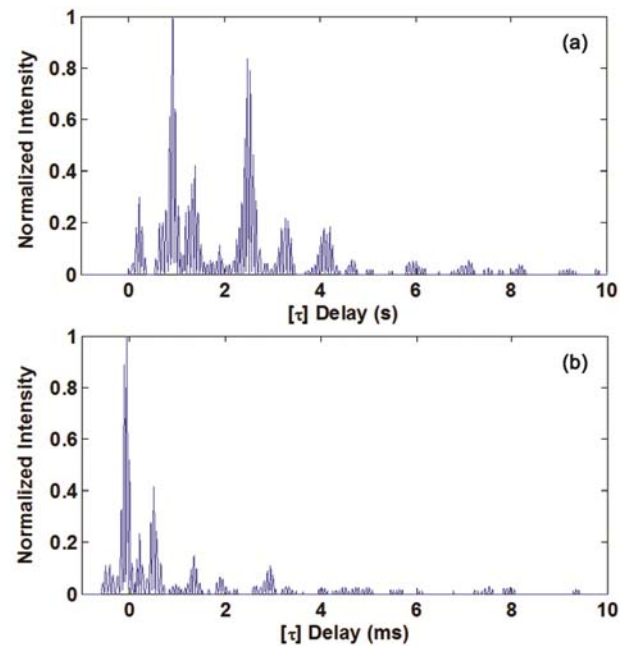
Fig. 5 — Multipath intensity profile for (a) channel 1 and (b) channel 2
