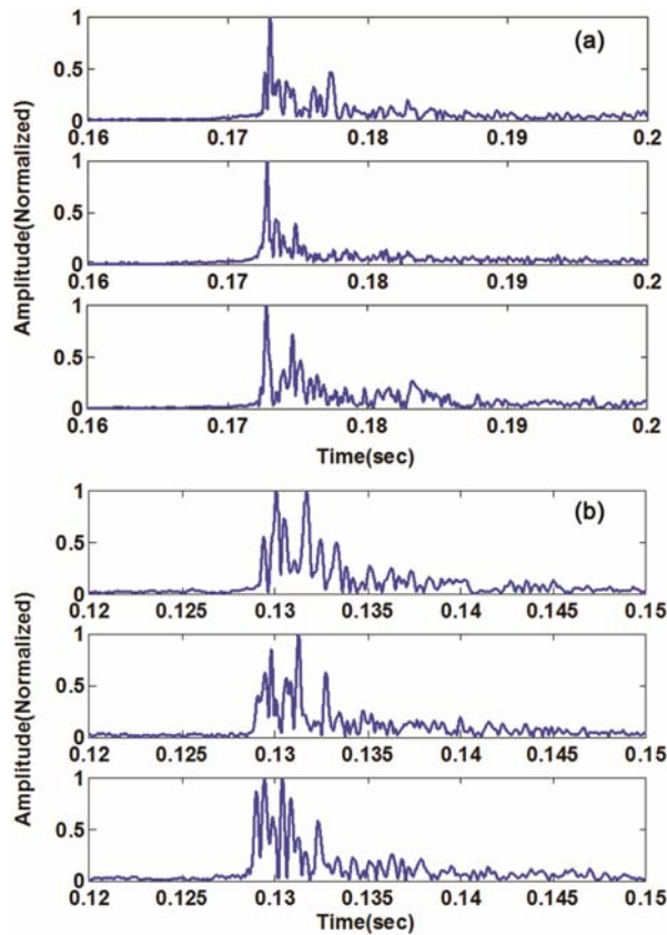
Fig. 4 — Channel response from hydrophone 1, 2 and 3 for channel 1 and 2
