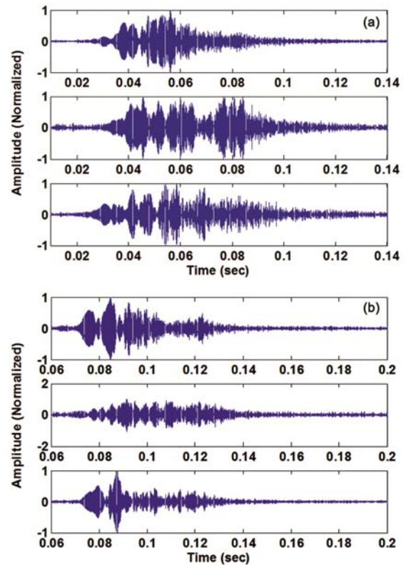
Fig. 3 — Received signals from hydrophone 1, 2 and 3 for (a) channel 1 and (b) channel 2
