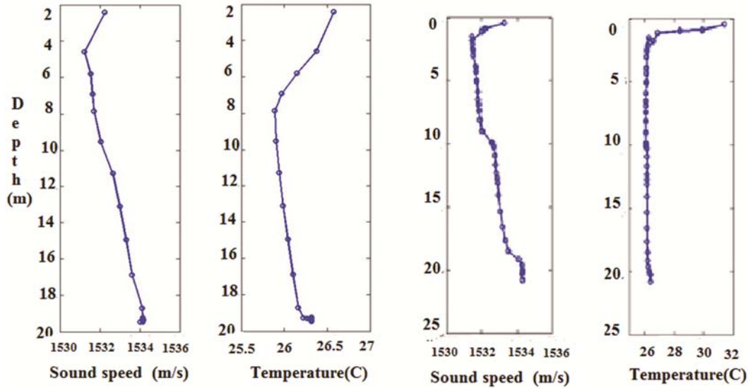
Fig. 2 — Sound speed and temperature variation at transmitter and receiver position (3 km) respectively
