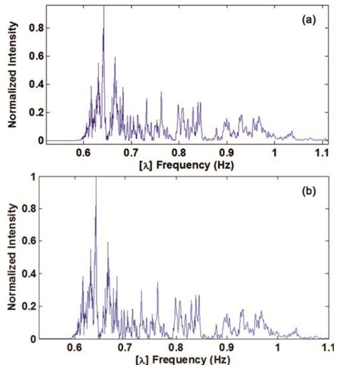
Fig. 6 — Doppler Power spectrum for (a) channel 1 and (b) channel 2
