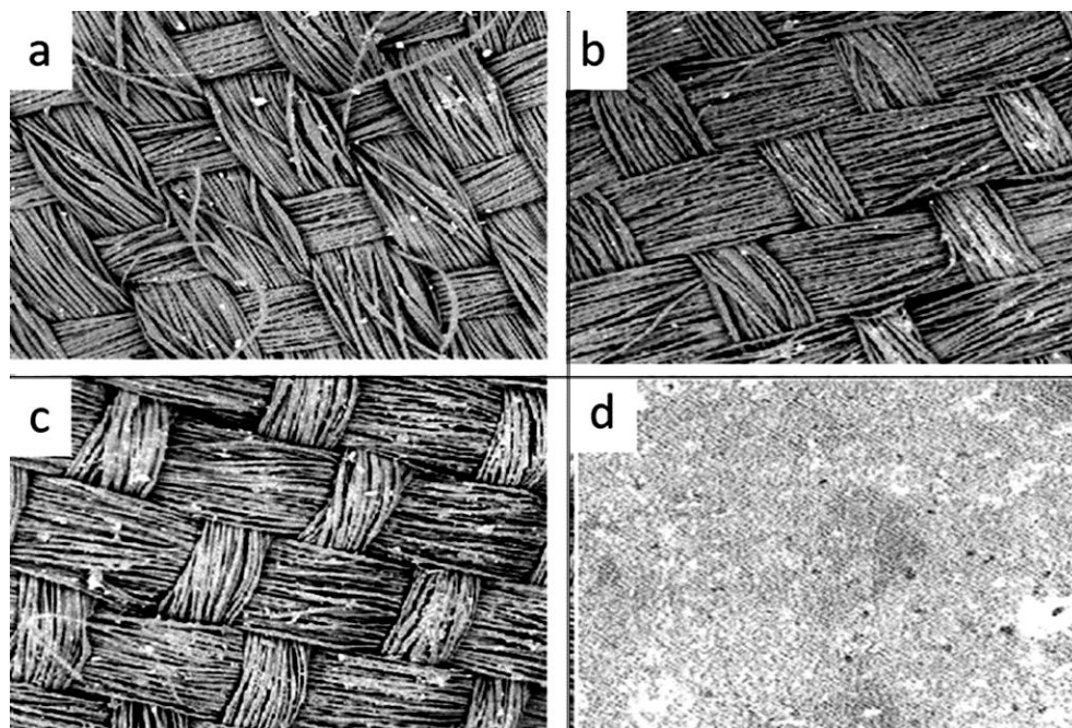
Fig. 2 — Scanning electron micrographs showing surface fibre pattern of silk based samples and leather (a) mulberry silk, (b) mulberry silk fused with non-woven fusing material, (c) mulberry silk quilted with foam and (d) leather
