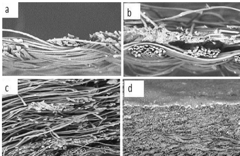
Fig. 3 — Scanning electron micrographs showing cross sectional view of silk based samples and leather (a) mulberry silk, (b) mulberry silk fused with non-woven fusing material, (c) mulberry silk quilted with foam and (d) leather
