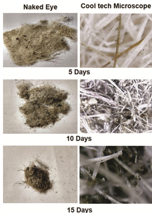
Fig. 4 — Biodegradation of raw nettle fibre after burial in soil
