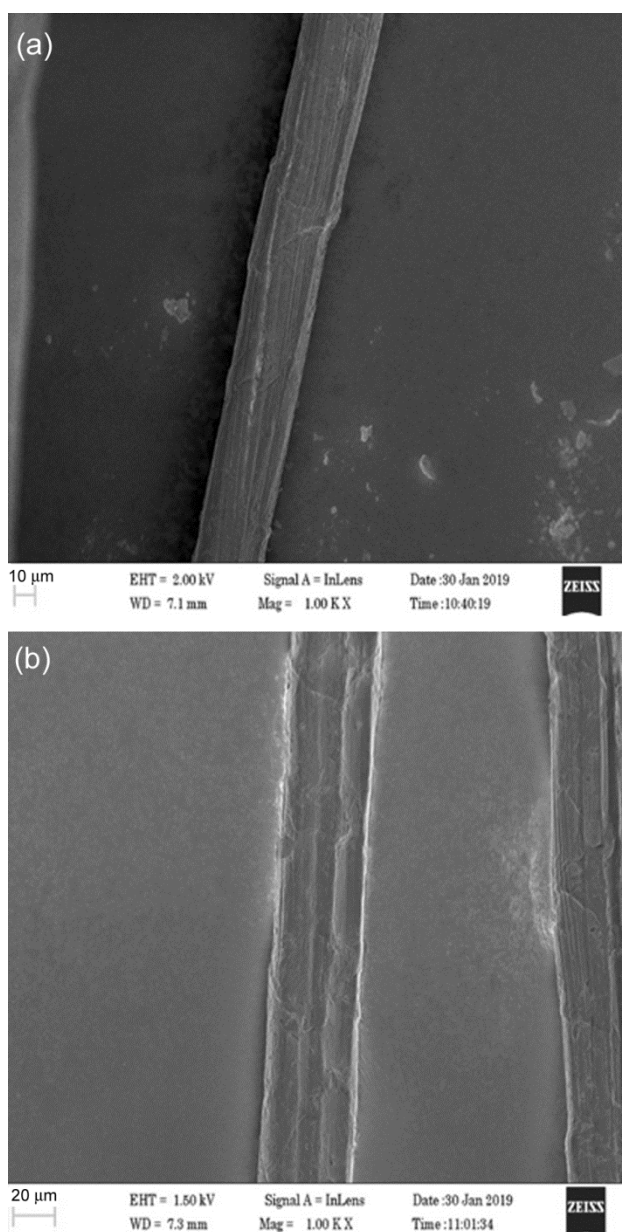
Fig. 2 — SEM Micrographs of (a) raw and (b) HCl treated nettle fibres
