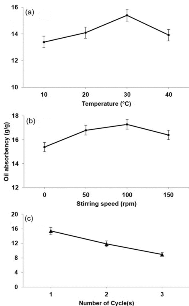
Fig. 3 — Effect of (a) temperature (b) stirring speed (c) no. of cycles (reusability) on oil absorbency
