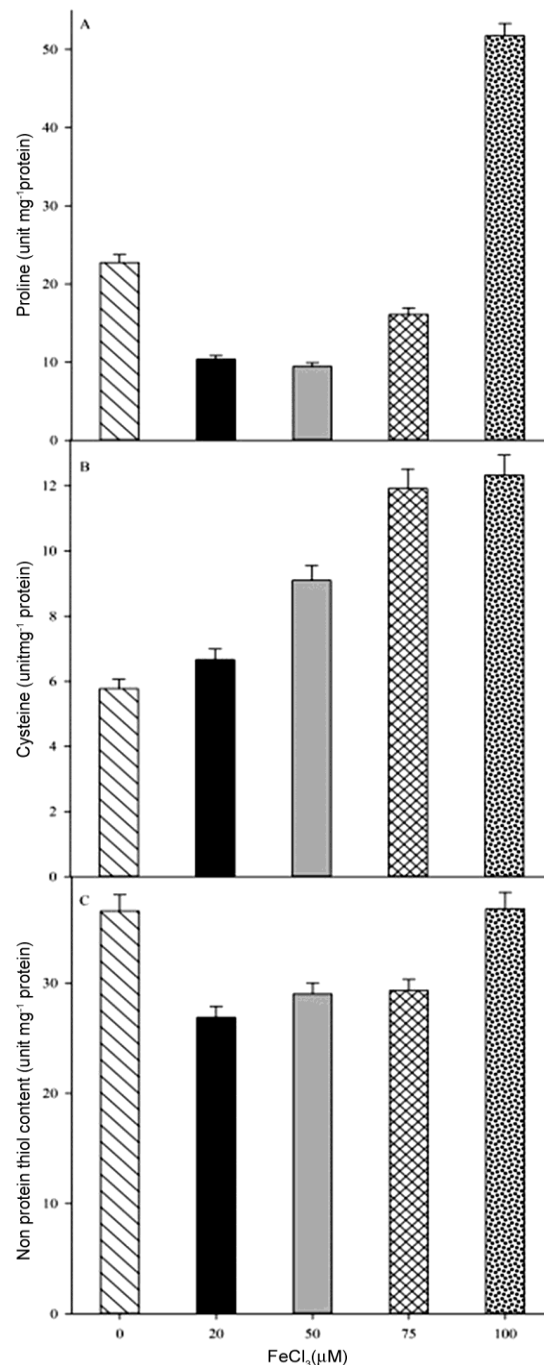
Fig. 7 — (A) Proline content; (B) cysteine; and (C) non protein thiol content of Anabaena sphaerica at different concentrations of \text{FeCl}_3 . [Data represents the mean \pm SD (n=6)]
