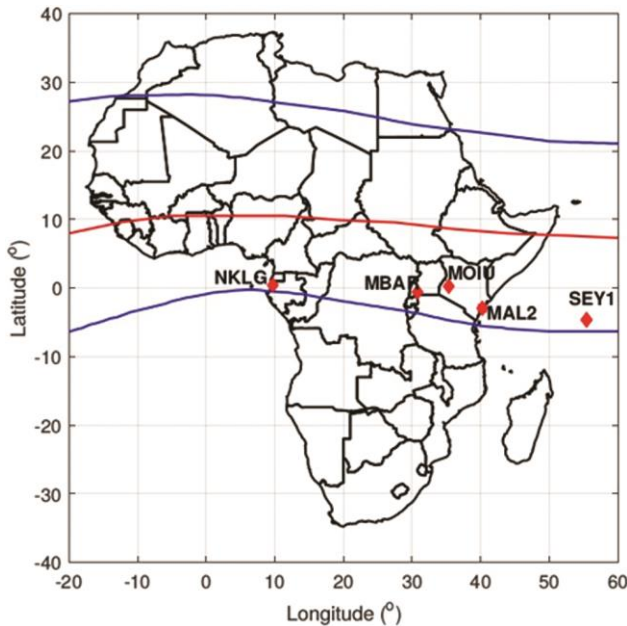
Fig. 1 — African map showing the geographic location of IGS receivers (red diamonds). The ionization anomaly region is represented by blue lines and the geomagnetic equator is represented by red line.
