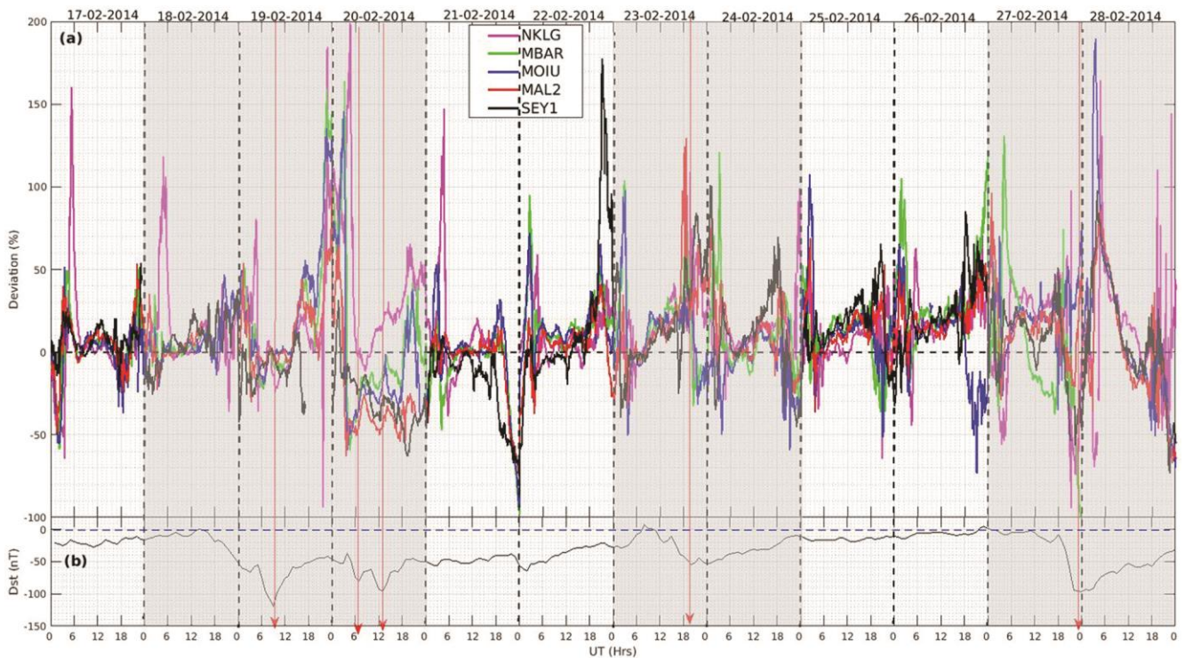
Fig. 5 — Percentage deviation of VTEC over NKLG, MBAR, MOIU, MAL2, and SEY1 for the geomagnetic storm period from 17 - 28 February, 2014. The Dst index is also plotted in panel (b).
