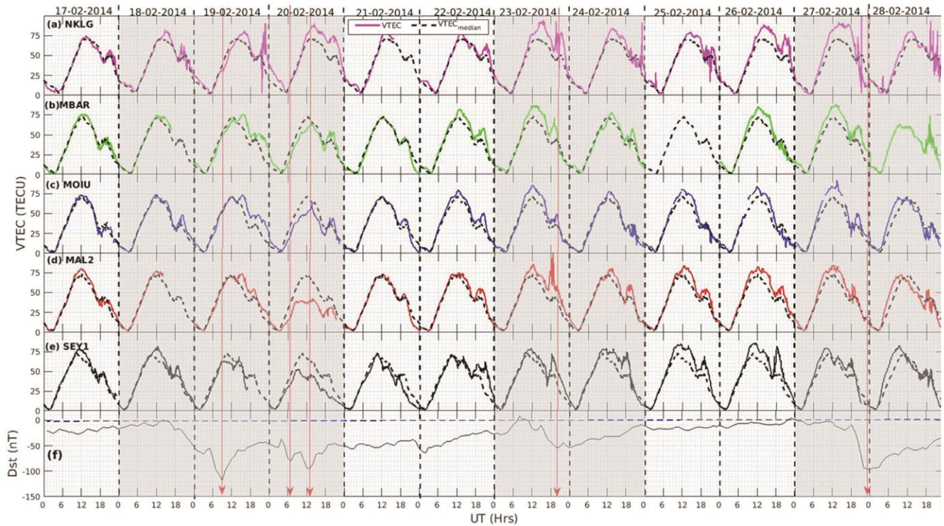
Fig. 4 — VTEC (solid curve) and monthly median VTEC (dotted curve) variations over (a) NKLG, (b) MBAR, (c) MOIU, (d) MAL2, and (e) SEY1 as a function of UT during 17 - 28 February 2014. The storm days are indicated by gray background.
