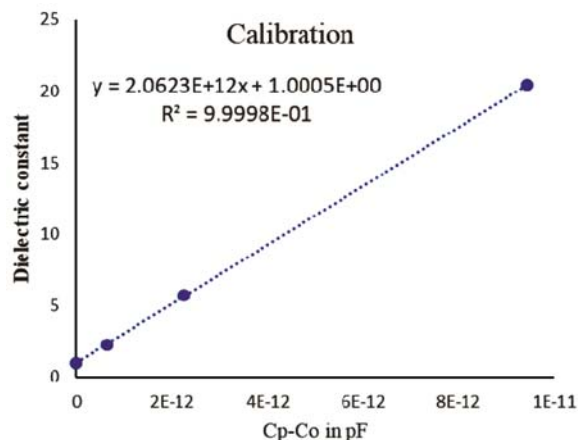
Fig. 1 – Calibration graph of the dielectric constant (ε) plotted against Cp-Co in pF.
