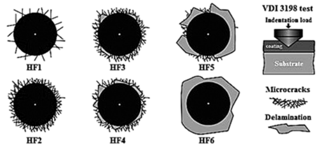
Fig. 2 — Principle of the VDI 3198 indentation test 53 .
