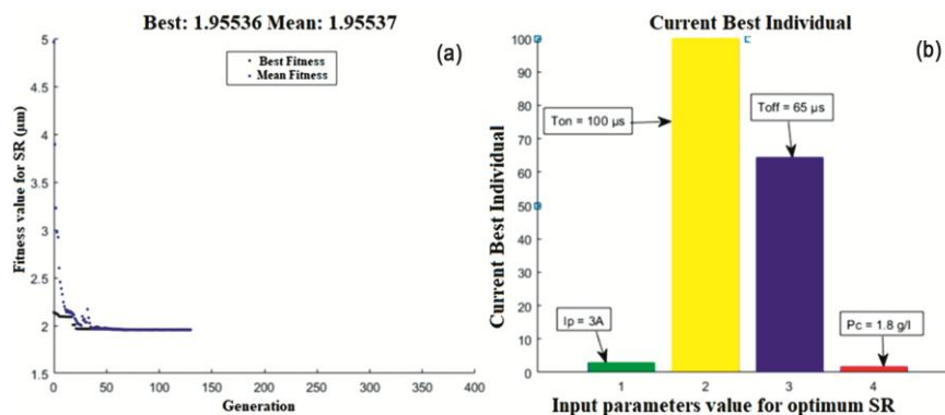
Fig.7 — MATLAB response for (a) SR fitness curve and (b) Optimum SR input setting.
