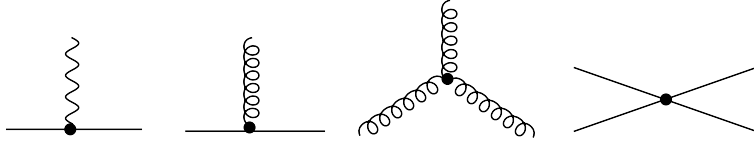
Figure 1. Schematic drawings of the \mathcal{PT} dimension-six operators in eq. (1.1). The QCD \bar{\theta} term is not shown. The solid, curly, and wavy lines denote external quark, gluon, and photon states respectively. The first and second diagram depict the quark EDM and chromo-EDM, respectively, the third diagram the Weinberg operator, and the fourth diagram a four-quark operator. Vertices with two or more gluon fields associated with the quark CEDM and the Weinberg operator are not shown.
