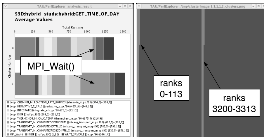
Figure 3. S3D cluster analysis. The figure on the left shows the difference in (averaged mean) execution behaviour between the two clusters of processes. The figure on the right shows a virtual topology of the MPI processes, showing the locations of the clustered processes. The lighter processes ran on XT3 nodes, and the darker processes ran on XT4 nodes.
