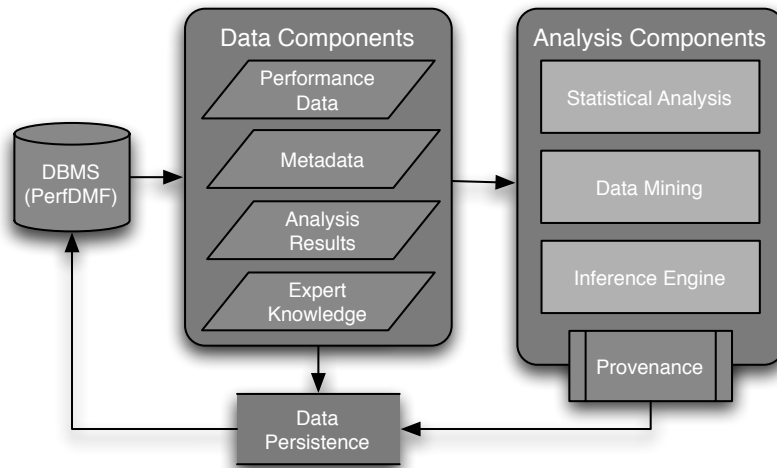
Figure 2. PerfExplorer components and their interactions.
