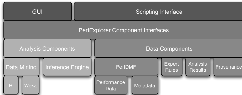
Figure 1. The redesigned PerfExplorer components.
