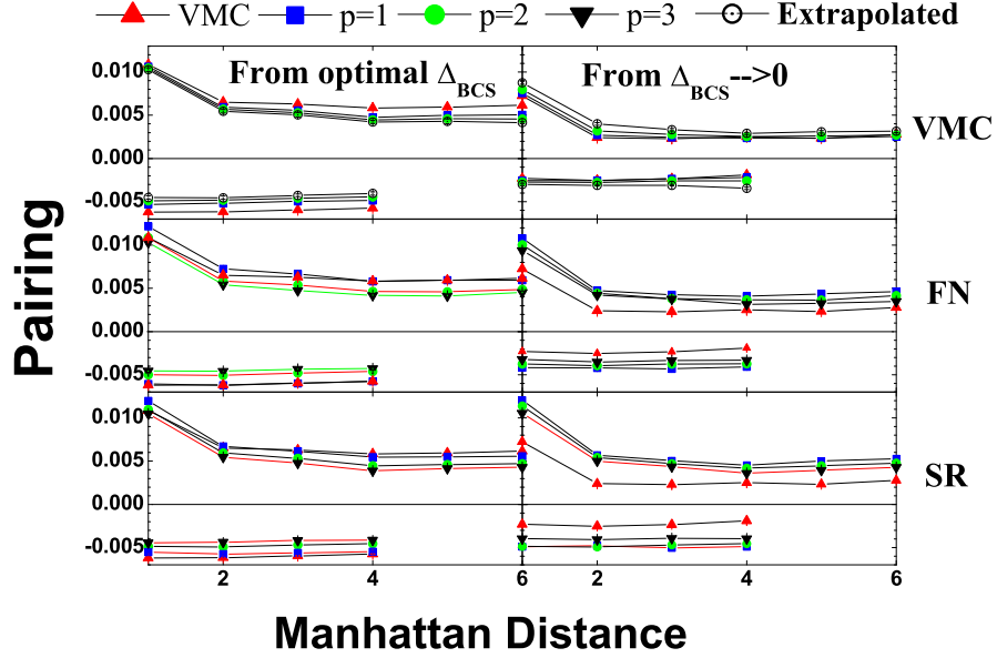
Figure 4. Pairing correlations in the 6 \times 6 lattice for 4 holes in the J/t = 0.5 t - J model. Left panels and right panels refer to two different initial guiding functions with or with vanishing small d-wave order parameter respectively. The latter is used in order to remove the degeneracy of the free electron Slater-determinant. The panels at different rows refer to different methods, as a function p of the hamiltonian powers used to evaluate the local energy e_L , required by all the methods: the larger is p , the more ( L^p for p \geq 2 ) computationally demanding is the calculation. The VMC values (red triangles) are plotted in all panels for comparison.
