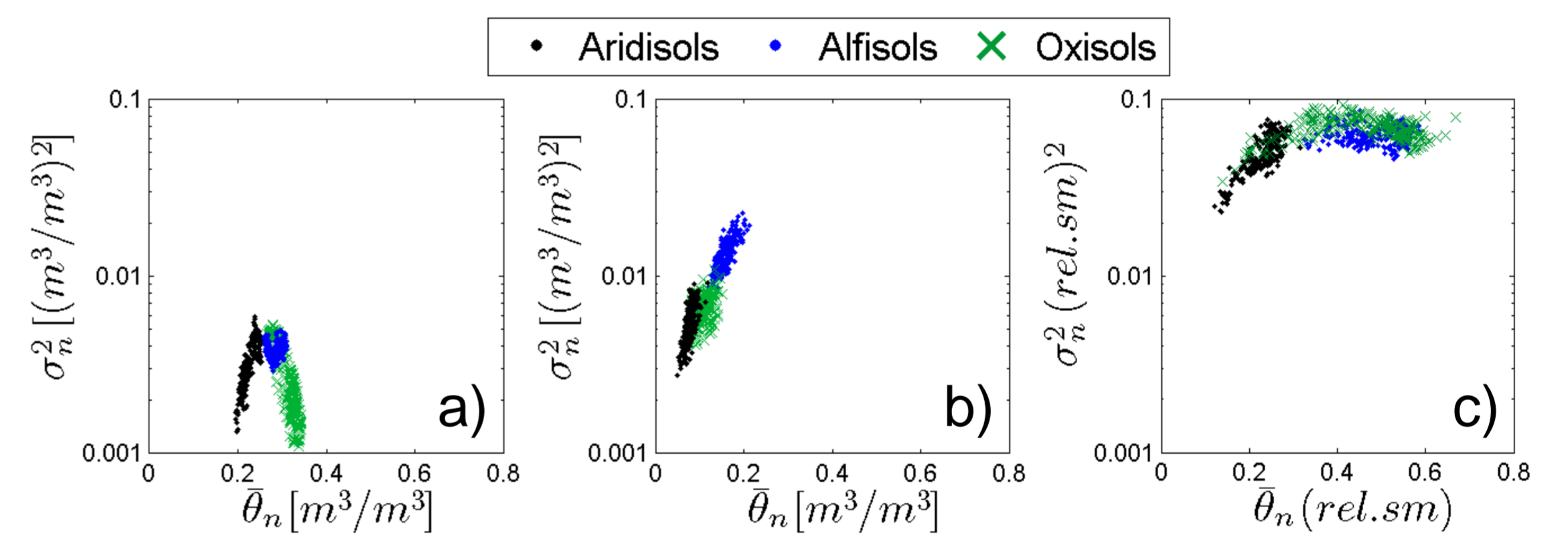
Fig. 4: Relation between spatial mean and spatial variance of soil moisture for a) ERA, b) SMOS and c) ASCAT soil moisture for selected soil orders. Different relationships of the products reflect characteristics of the products, while the same relationships (e.g. Aridisols) indicate characteristics of the respective region.
