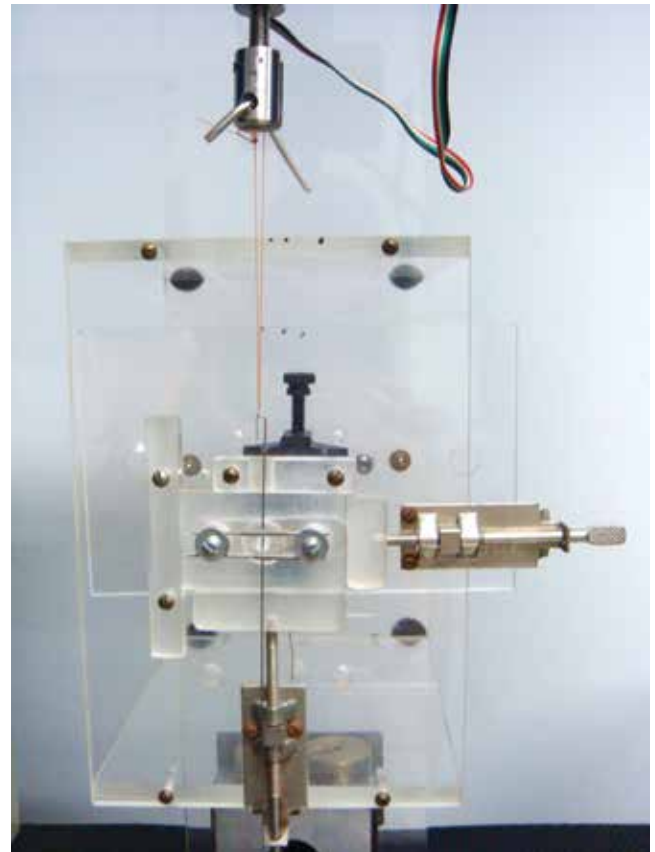
Figure 2 - Completely assembled test system.
