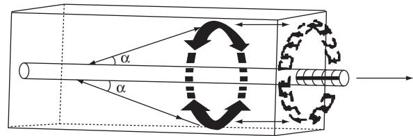
Figure 1. Representation of the radial component of by strength bond in the anchorage zone (Tepfers, 1979).
