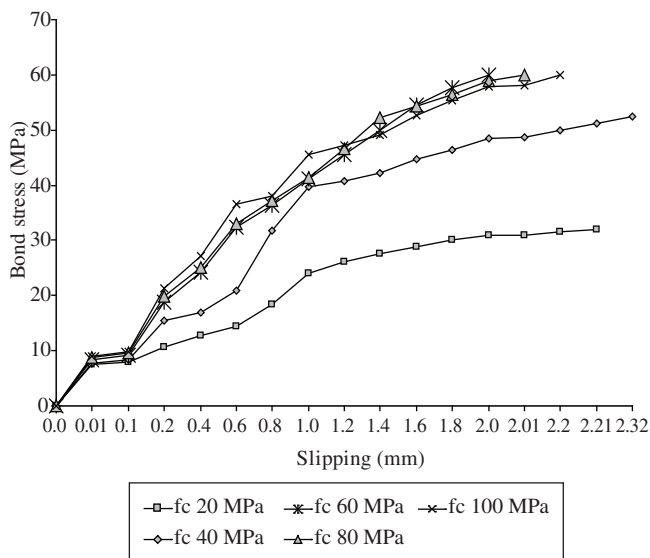
Figure 5. Bond Stress vs. Slipping ( \phi = 25.0 mm).
