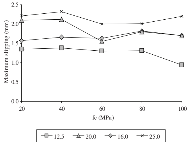
Figure 6. Maximum slipping vs. strength of concrete.
