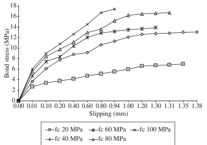
Figure 2. Bond Stress vs. Slipping (ϕ = 12.5 mm).
