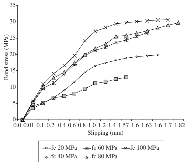
Figure 3. Bond Stress vs. Slipping (ϕ = 16.0 mm).
