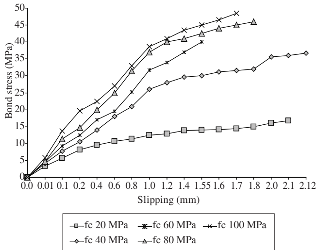
Figure 4. Bond Stress vs. Slipping ( \phi = 20.0 mm).
