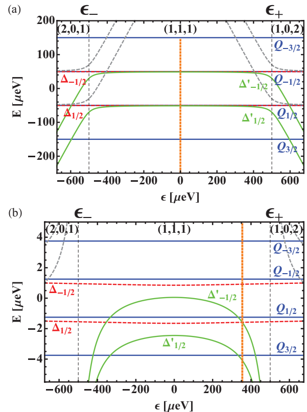
FIG. 2. (Color online) Diagram of the eigenenergies of the exchange Hamiltonian of Eq. (1) as a function of the bias parameter \epsilon with E_z > 0 . The dashed gray lines are the higher energy states that are not treated by the \mathcal{H} in Eq. (1). They are removed from the \mathcal{H}_{\text{Hubbard}} by adiabatic elimination. (a) The case of large external magnetic fields: E_z = 100 \mu\text{eV} ( \approx 7 T in GaAs). In (b) the external magnetic fields are small ( E_z = 2.5 \mu\text{eV} , corresponding to 200 mT in GaAs). The dashed orange lines mark regimes analyzed in the analysis of Sec. IV.
