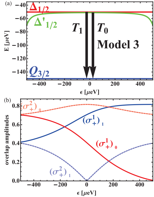
FIG. 13. (Color online) Description of local spin relaxation for the subspace qubit at large external magnetic fields ( E_z = 100 \mu\text{eV} ). Only local spin relaxations from the interaction with phonons are significant. (a) Sketch of energy diagram of the subspace qubit to describe the time evolution under local spin relaxation. T_1 and T_0 are the dominant transition rates from the qubit levels to the s_z = \frac{3}{2} quadruplet state. (b) Transition amplitudes for the qubit state i through the noise operator \sigma_+ acting on dot j : (\sigma_+^i)_j = |\langle Q_{\frac{3}{2}} | \sigma_+^i | W_j \rangle| ( W_1 = \Delta_{\frac{1}{2}} , W_0 = \Delta'_{\frac{1}{2}} ).
