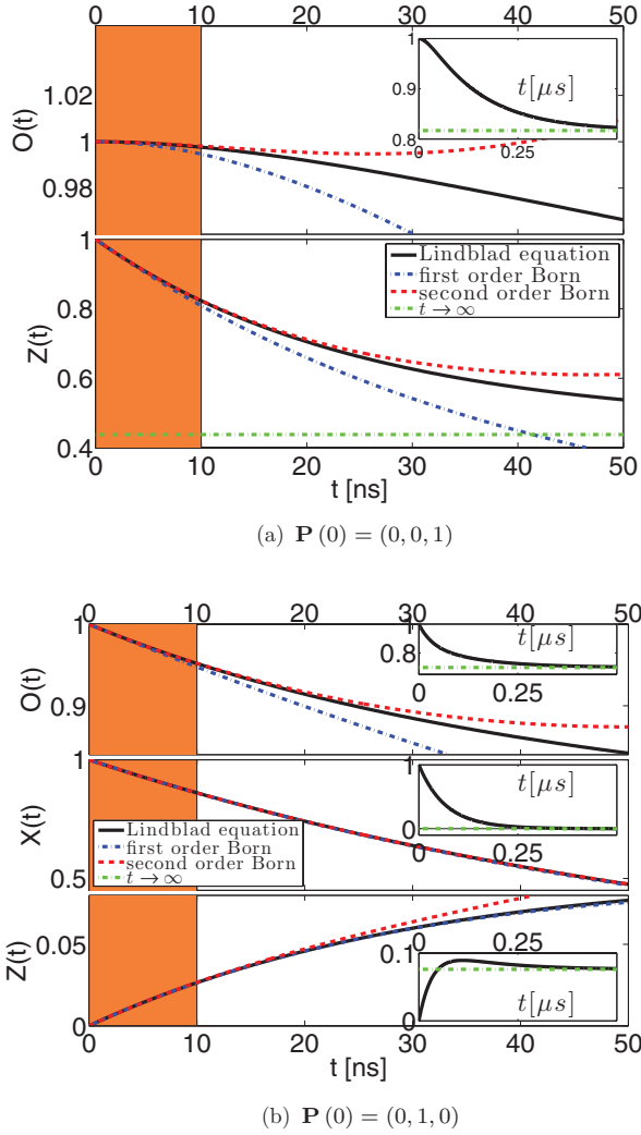
FIG. 9. (Color online) Time evolution of the subsystem qubit at E_z = 2.5 \mu\text{eV} through local spin relaxations at \epsilon = 354.6 \mu\text{eV} [compare energy diagram in Fig. 2(b)]. The major influence is from local spin relaxation, generated from hyperfine interactions. We use \Upsilon_1^x = (20 \text{ ns}^{-1}) , \Upsilon_2^x = (30 \text{ ns}^{-1}) , and \Upsilon_3^x = (40 \text{ ns}^{-1}) . The orange region marks a typical time scale of qubit experiments. Here the second-order Born approximation and the results from the full master equation match very closely. The insets show the long time evolution of the qubit. We see thermalization occurring within microseconds.
