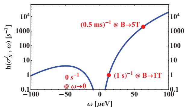
FIG. 5. (Color online) Relaxation rates h(\sigma_x^i, \omega) generated by piezoelectric phonons according to Eq. (27). Experimentally observed time scales from qubit experiments (Ref. 33) are included in this picture.
