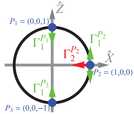
FIG. 17. (Color online) Sketch of transition rates, extracted from the initial time evolution of the qubit on the Bloch sphere at three special points. The Bloch sphere parameters are renormalized by the trace evolution of relevant part of the density matrix, which describes the qubit: \hat{P}_{x,z}(t) \equiv P_{x,z}(t) / \text{Tr}(\rho^{\text{rel}}) .
