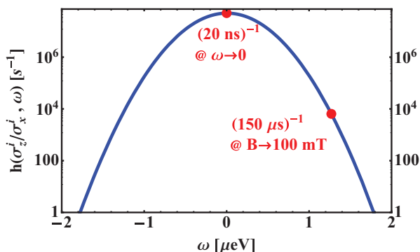
FIG. 4. (Color online) Hyperfine interaction causes dephasing and relaxation through local magnetic field fluctuations on each quantum dot. Dephasing and relaxation is generated by the transition rates h(\sigma_z^i/\sigma_x^i, \omega) according to Eq. (21). The marked points refer to results from two qubit experiments, described in the main text.
