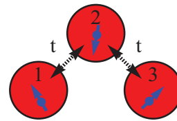
FIG. 1. (Color online) Layout of the triple quantum dot setup. Each quantum dot is occupied with one electron. Neighboring dot pairs are tunnel coupled with the coupling strength t . An external electric bias is used to occupy either the left (dot 1) or the right (dot 3) quantum dot with two electrons.
