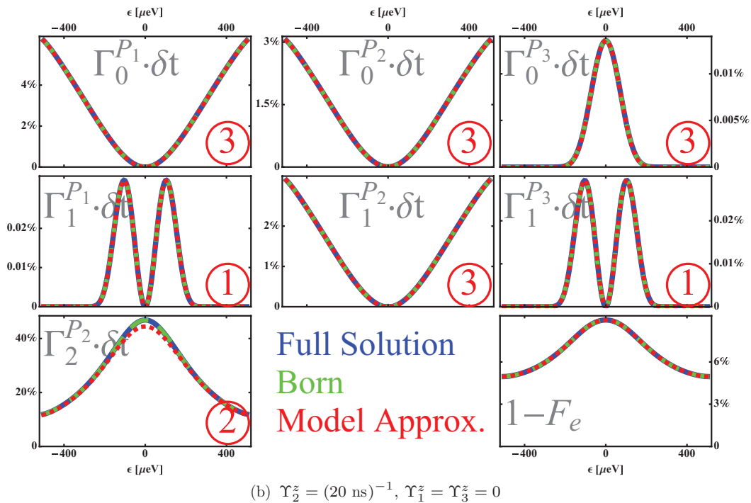
FIG. 10. (Color online) Errors from local phase noise on the subspace qubit at E_z = 100 \mu\text{eV} . We take into account the influence of fluctuating hyperfine fields through the transition rates from Eq. (21). The effective error rates are extracted from the numerical simulation of the full master equation (blue lines) and of the second-order Born approximation (green lines). Red lines describe effective errors from simple toy models, as described in the text. For each extracted error rate we add with a red number the specific model system under consideration from Appendix E.
