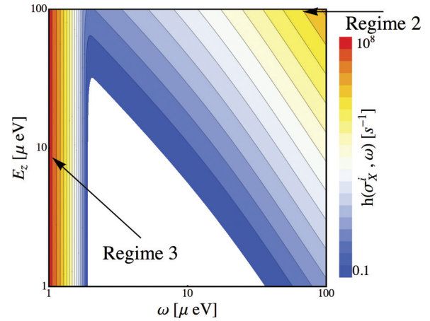
FIG. 6. (Color online) Density plot of the transition rates for local spin relaxation h(\sigma_x^i, \omega) as a function of the energy difference \omega and the external magnetic field E_z . The influence of hyperfine interaction (Regime 2) and phonon interaction (Regime 3) can be separated due to the different parameter ranges when the effects are dominant. The hyperfine mechanism is independent of E_z .
