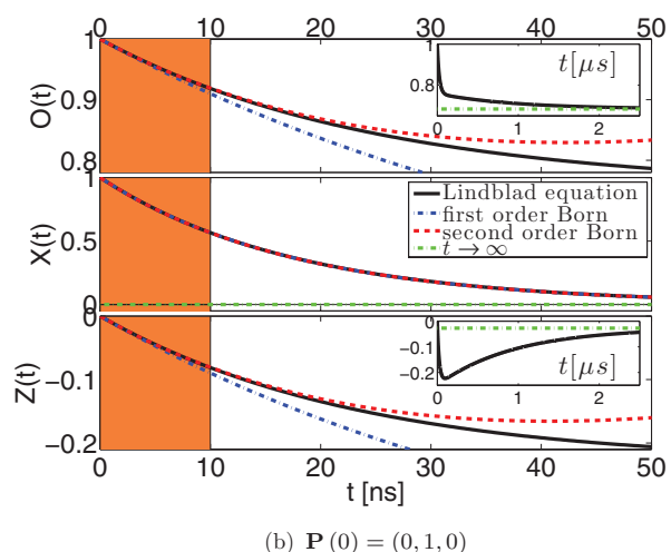
FIG. 7. (Color online) Time evolution of the subspace qubit without electric bias ( \epsilon = 0 \mu\text{eV} ) at E_z = 100 \mu\text{eV} . The qubit is subjected to local phase noise generated by fluctuating hyperfine fields [ \Upsilon_1^z = (20 \text{ ns}^{-1}) , \Upsilon_2^z = (30 \text{ ns}^{-1}) , \Upsilon_3^z = (40 \text{ ns}^{-1}) ]. The orange region marks a typical time interval for qubit experiments: [0, 10] \text{ ns} . Blue lines represent the results from the first-order Born approximation, while red lines are calculated in the second-order Born approximation. The insets show the evolution on a longer time scale. Green lines represent the long time limit of the evolution as discussed in the text.
