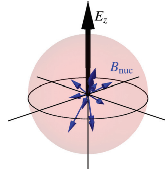
FIG. 3. (Color online) Semiclassical picture used for the time evolution of a single electron spin in a distribution of hyperfine configurations. For every experiment the hyperfine field acts like a static magnetic field, which is randomly varying between every run of the experiment. A constant external magnetic field E_z is applied in the z direction.
