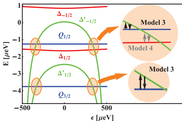
FIG. 16. (Color online) Transition diagram for subsystem qubit when hyperfine interactions generate local spin flips. Large error rates are observed only at the region of level crossings. They can be described by leakage transitions to a quadruplet state (model 3 from Appendix E 3) or internal transitions between two states of the subsystem qubit (model 4 from Appendix E 4).
