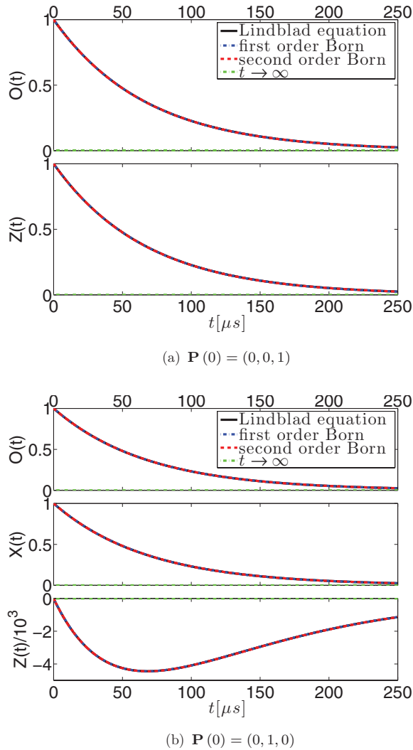
FIG. 8. (Color online) Time evolution from local spin relaxation for the unbiased subspace qubit generated by the interaction with piezoelectric phonons for \epsilon = 0 and E_z = 100 \mu\text{eV} . The transition parameters are chosen to \Xi^x = 2 \times 10^{-6} \frac{1}{s \mu\text{eV}^5} , \Xi^y = 1.5 \times 10^{-6} \frac{1}{s \mu\text{eV}^5} , and \Xi^z = 1 \times 10^{-6} \frac{1}{s \mu\text{eV}^5} . The numerical solution of the full master equation (black lines) and the first-order (blue lines) and second-order (red lines) Born approximations are identical. The qubit depopulates completely in the long time limit.
