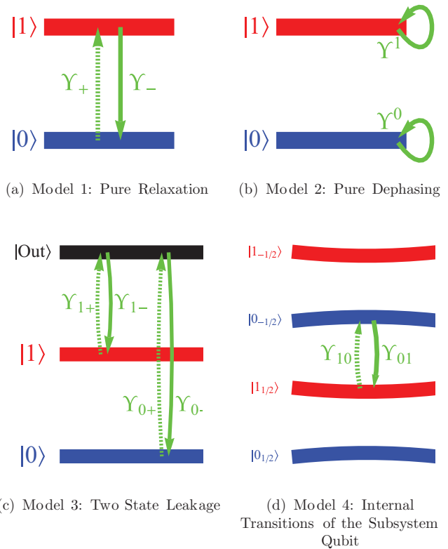
FIG. 18. (Color online) The time evolution of the qubit in triple quantum dots can be described by four toy models (a)–(d).
