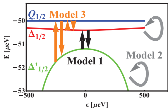
FIG. 11. (Color online) Energy diagram of the subspace qubit with major transition rates generated from local phase noise. The energy diagram shows only the relevant energy levels for this description [cf. Fig. 2(a)]. The transition rates can be grouped into three sets, which are described by the toy models analyzed in Appendix E. Model 1 describes pure relaxation of the qubit states (black arrows; see Appendix E 1), model 2 describes pure dephasing of the qubit states (gray arrows; see Appendix E 2). Model 3 characterizes leakage of the qubit states to one state in the surroundings (orange arrows; see Appendix E 3).
