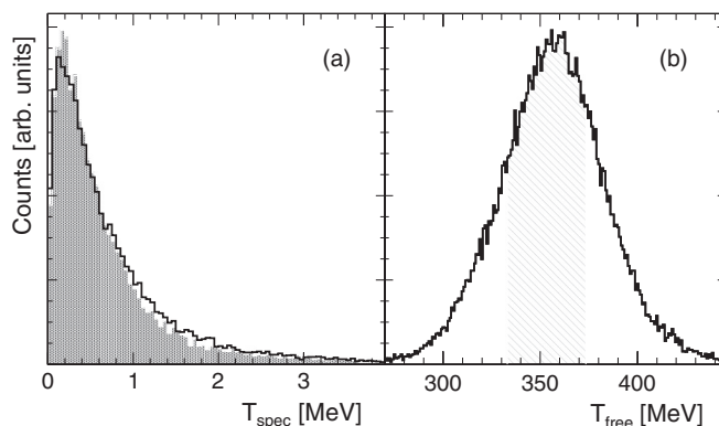
FIG. 2. (a) Experimental (histogram) and simulated (shaded area) distribution in the deuteron rest frame of spectator proton energies from the dp \rightarrow \{pp\}_s \pi^- p_{\text{spec}} reaction for the selected T_{\text{free}} range. (b) Experimental distribution of effective beam energies; the region selected for analysis is shown by the shading.
