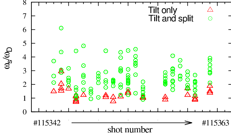
Figure 2: The ratio of the E_r \times B flow shear rate ( \omega_s ) to the natural diffusive scattering rate of ambient turbulence ( \omega_D ) in a number of discharges at TEXTOR for the eddy "tilt only" and "tilt and split" events. The x-axis corresponds to different shot numbers.
