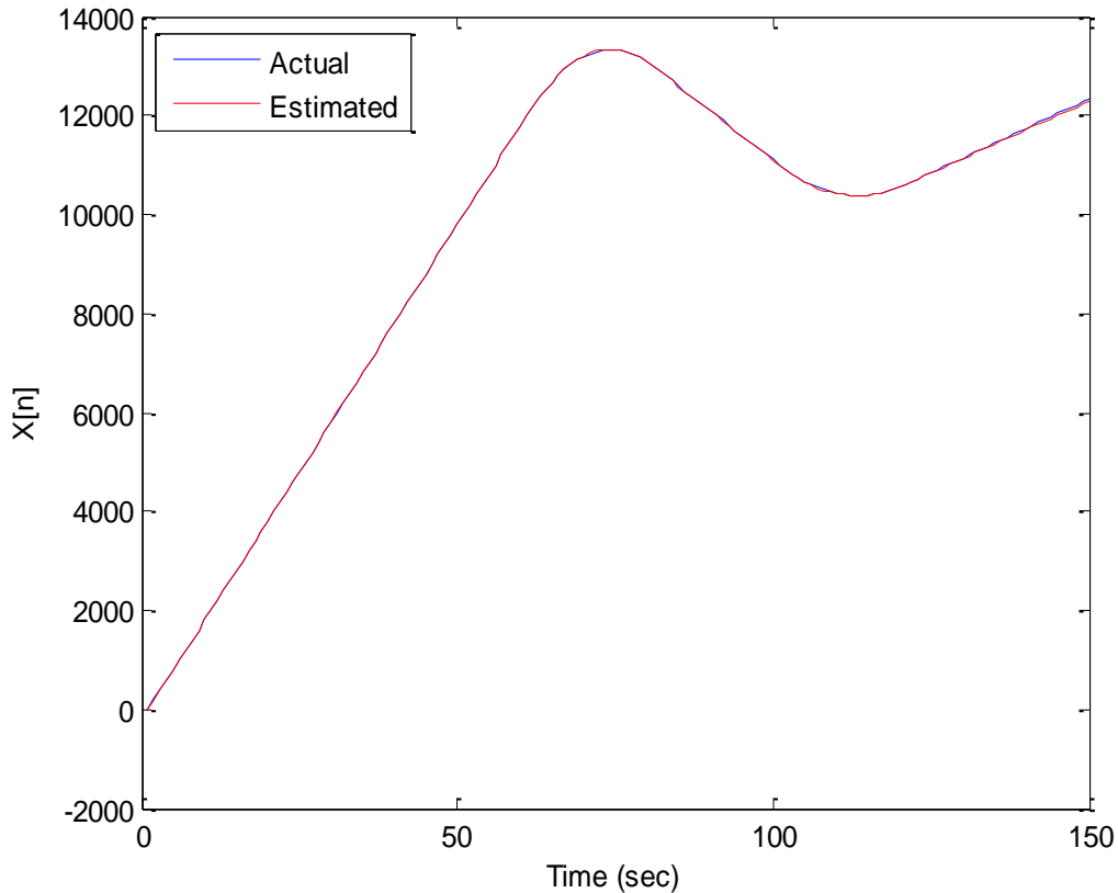
Fig. 2-13: Kalman filter performance in x plane
