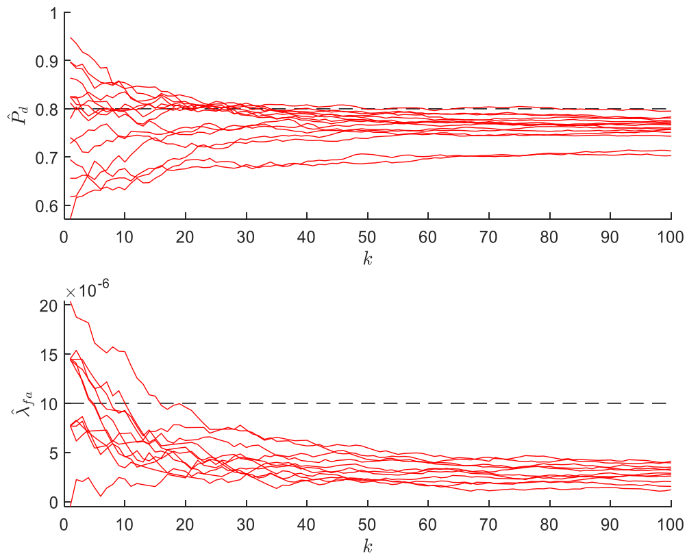
Fig. 4-38: Estimation results for the probability of detection and density of false alarms when the measurement noise matrix is unknown
