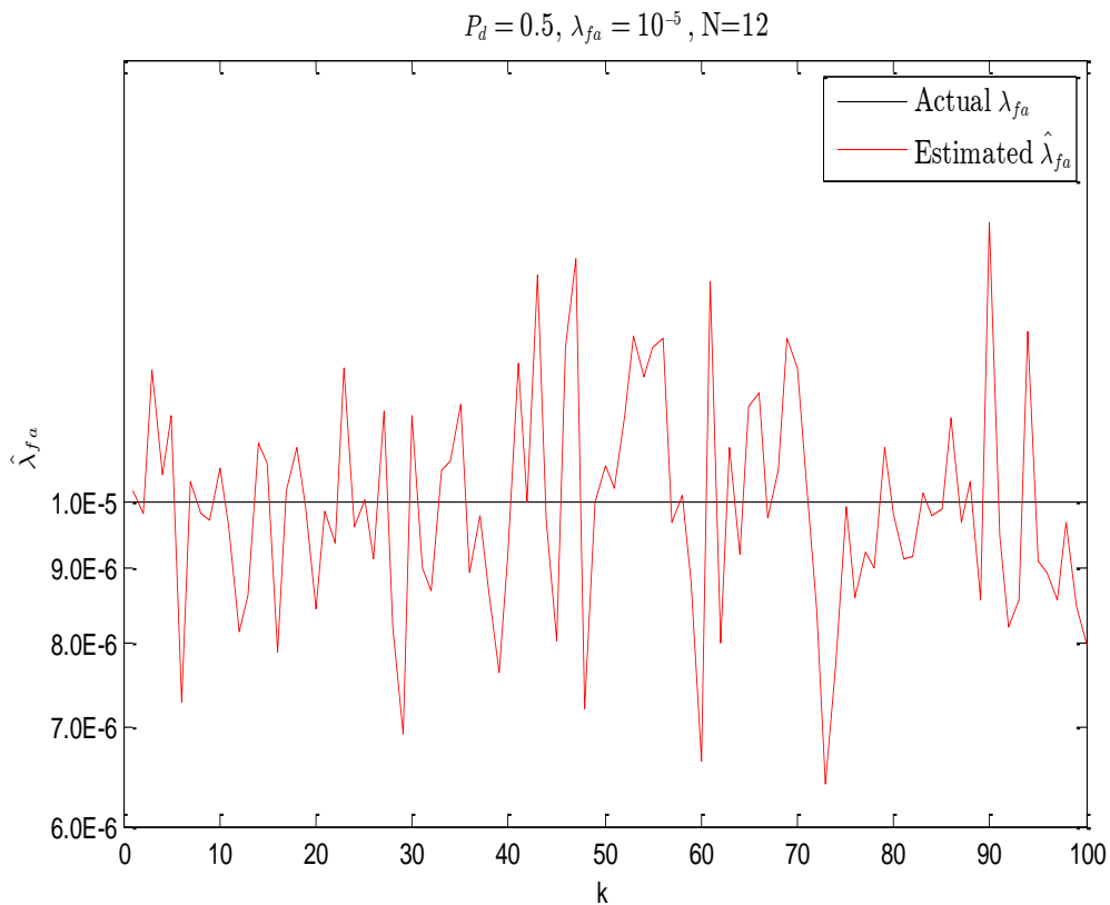
Fig. 4-16: Estimation of the density of false alarm
