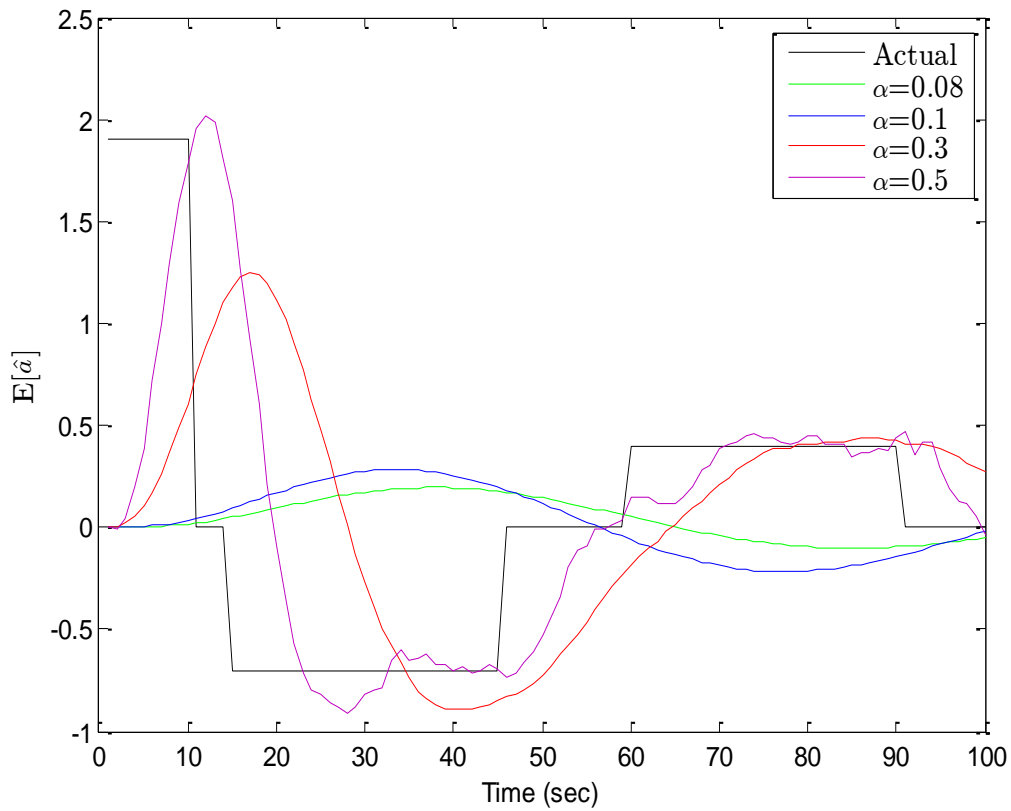
Fig. 2-10: Estimation of acceleration ( \alpha - \beta - \gamma filter)
