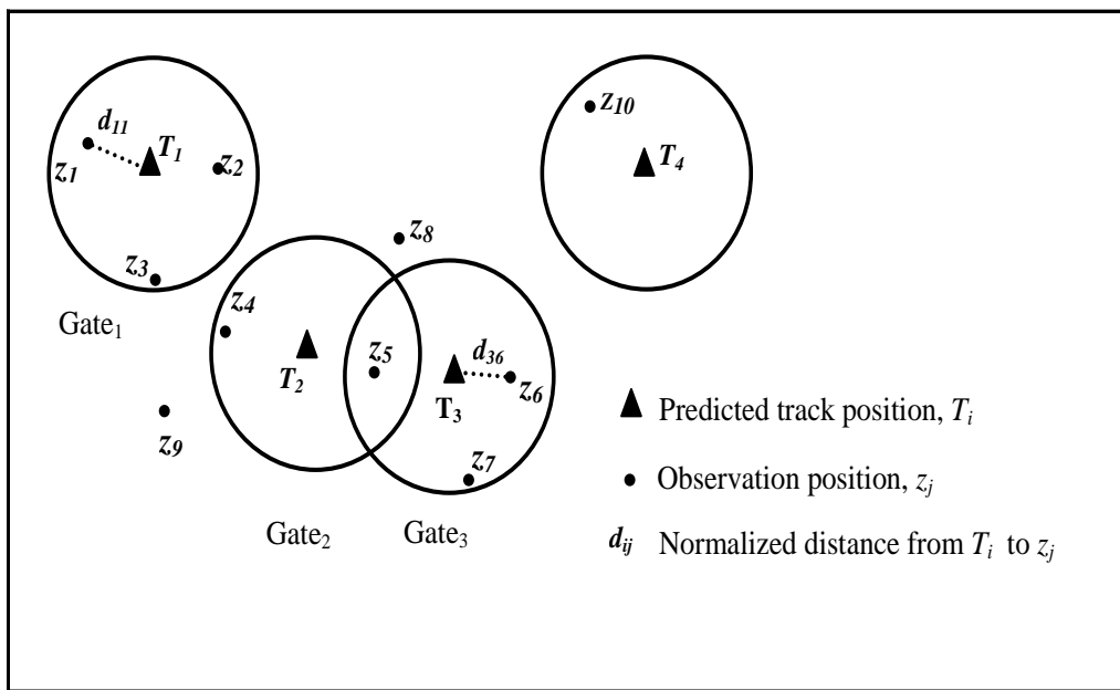
Fig. 2-2: The gating process
