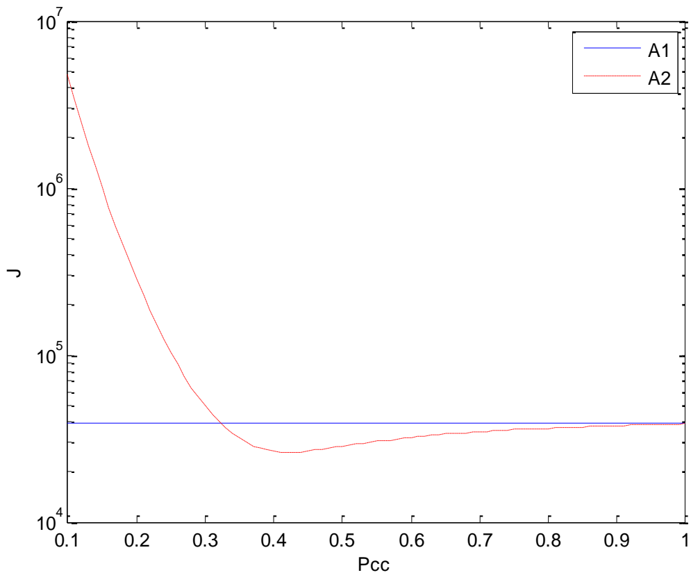
Fig. 2-21: Mean squared errors for \lambda_{fa} = 1.3 \times 10^{-4}
