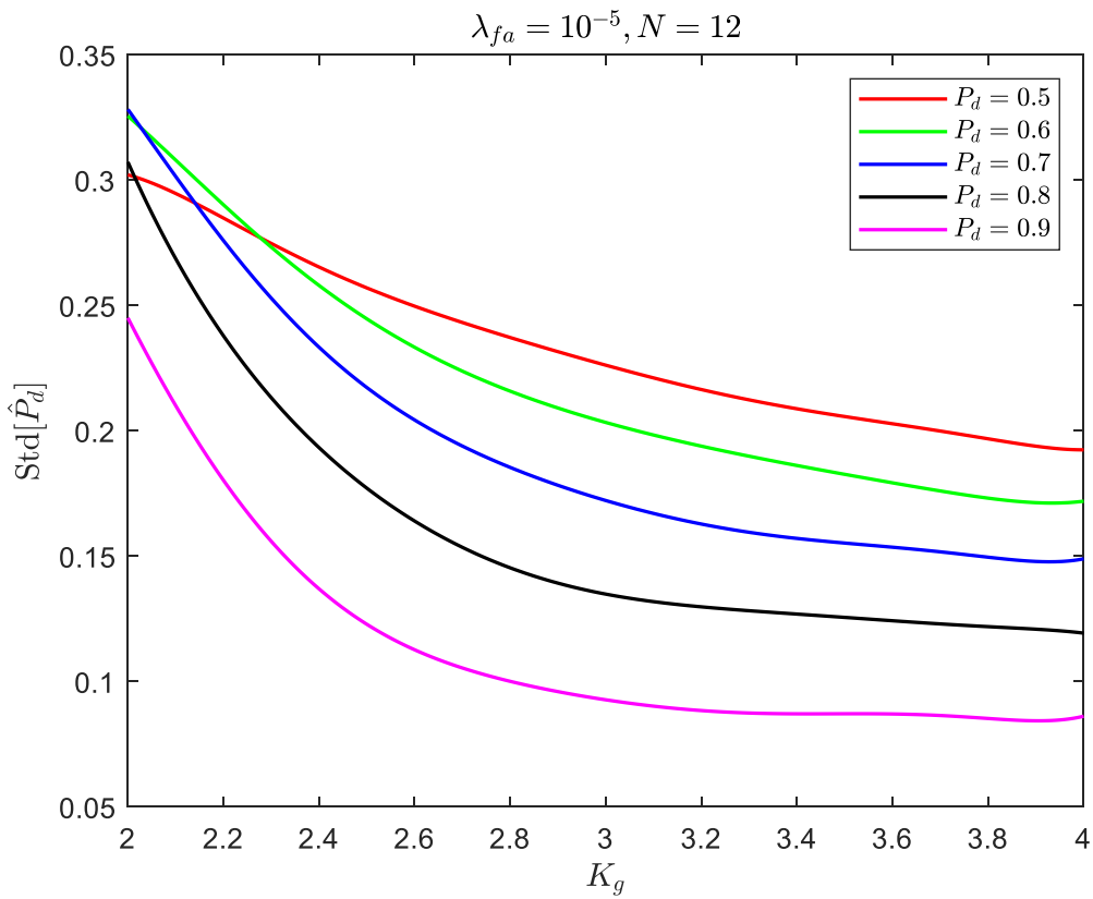
Fig. 4-3: Standard deviation of the estimated probability of detection
