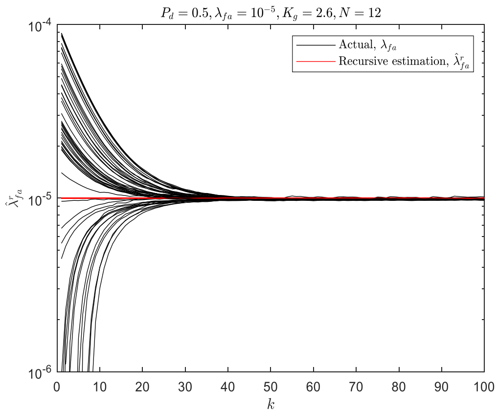
Fig. 4-33: Recursive estimation of density of false alarms at fixed actual P_d = 0.5 and \lambda_{fa} = 10^{-5} for different initial conditions
