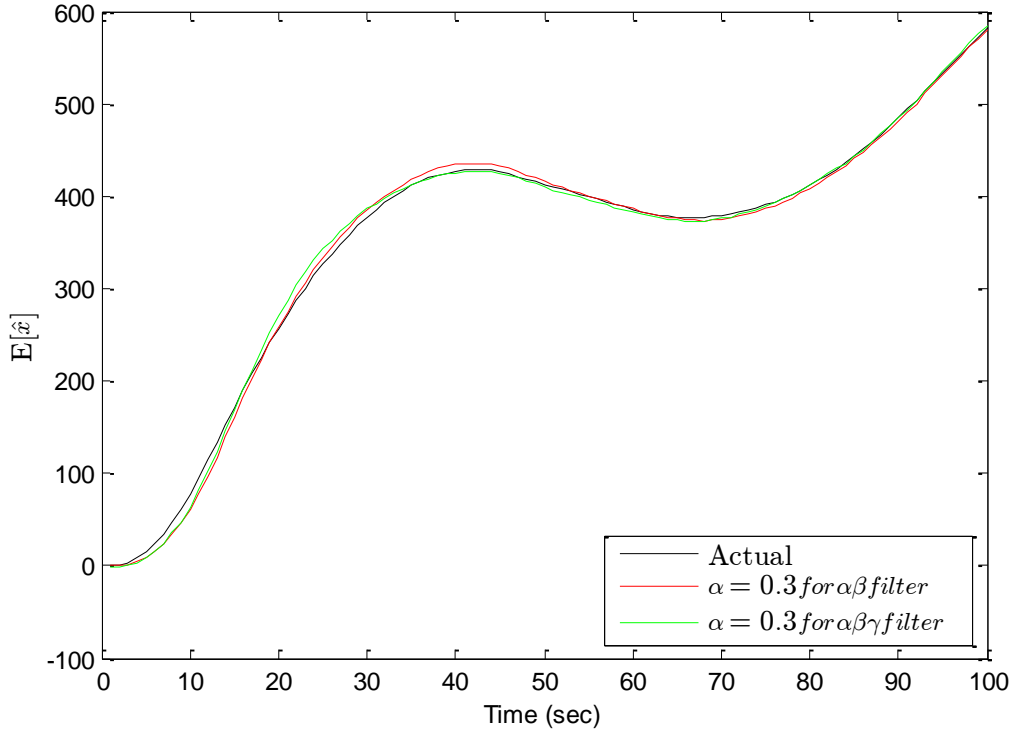
Fig. 2-11: Comparison in the estimation of the position between ( \alpha\beta and \alpha\beta\gamma ) filters
