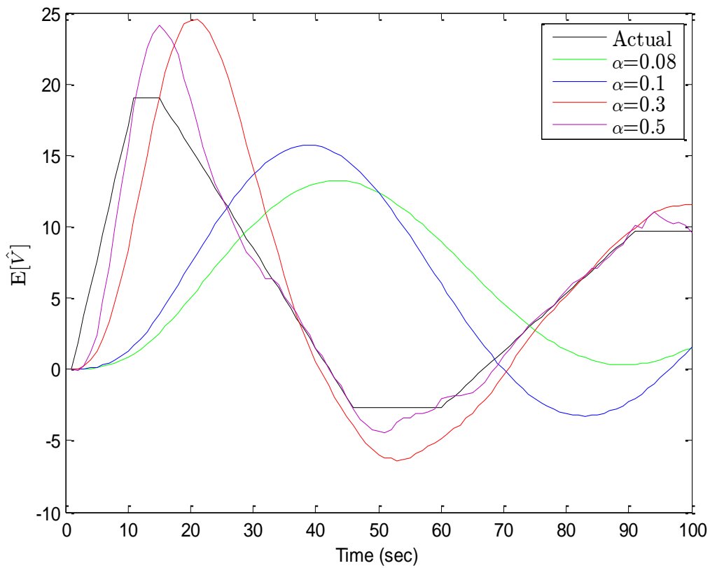
Fig. 2-9: Estimation of velocity ( \alpha - \beta - \gamma filter)
