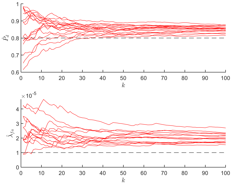
Fig. 4-39: Estimation results for the probability of detection and density of false alarms when the measurement noise matrix is unknown
