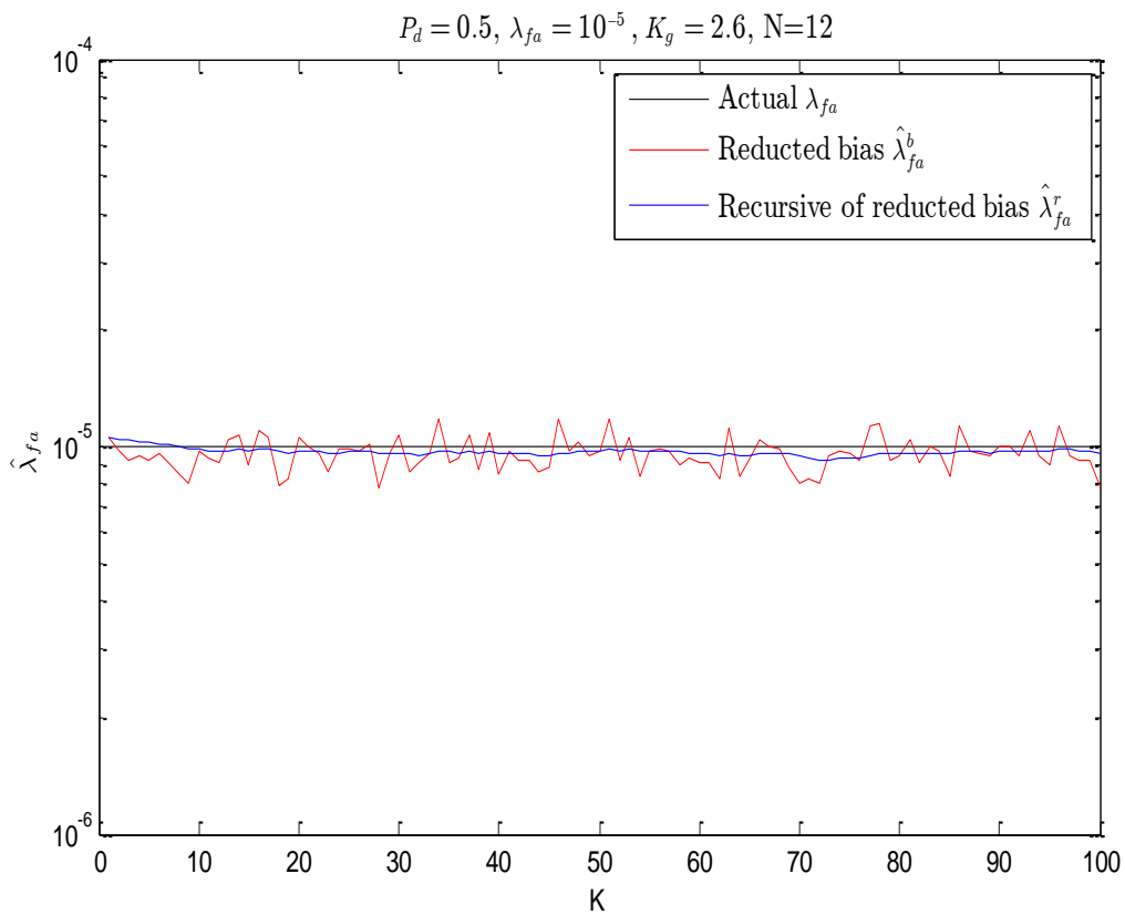
Fig. 4-31: Recursive estimation of density of false alarms at fixed actual P_d = 0.5 and \lambda_{fa} = 10^{-5}
