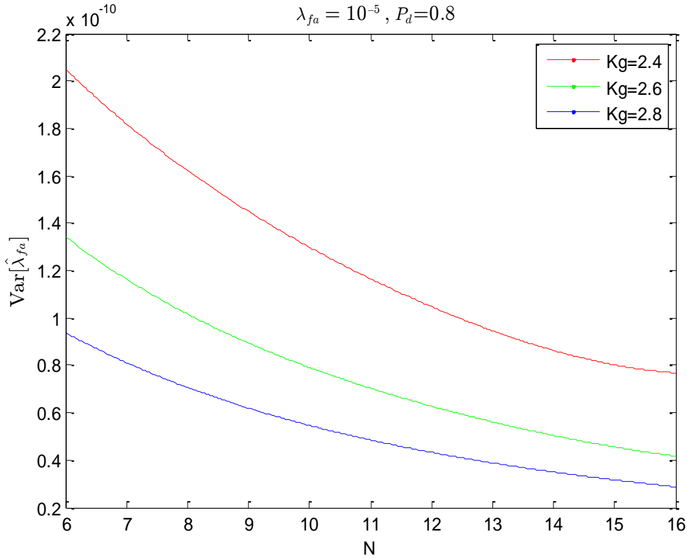
Fig. 4-14: Variance of the estimated density of false alarm as a function of length of sequence N for different values of gate size K_g
