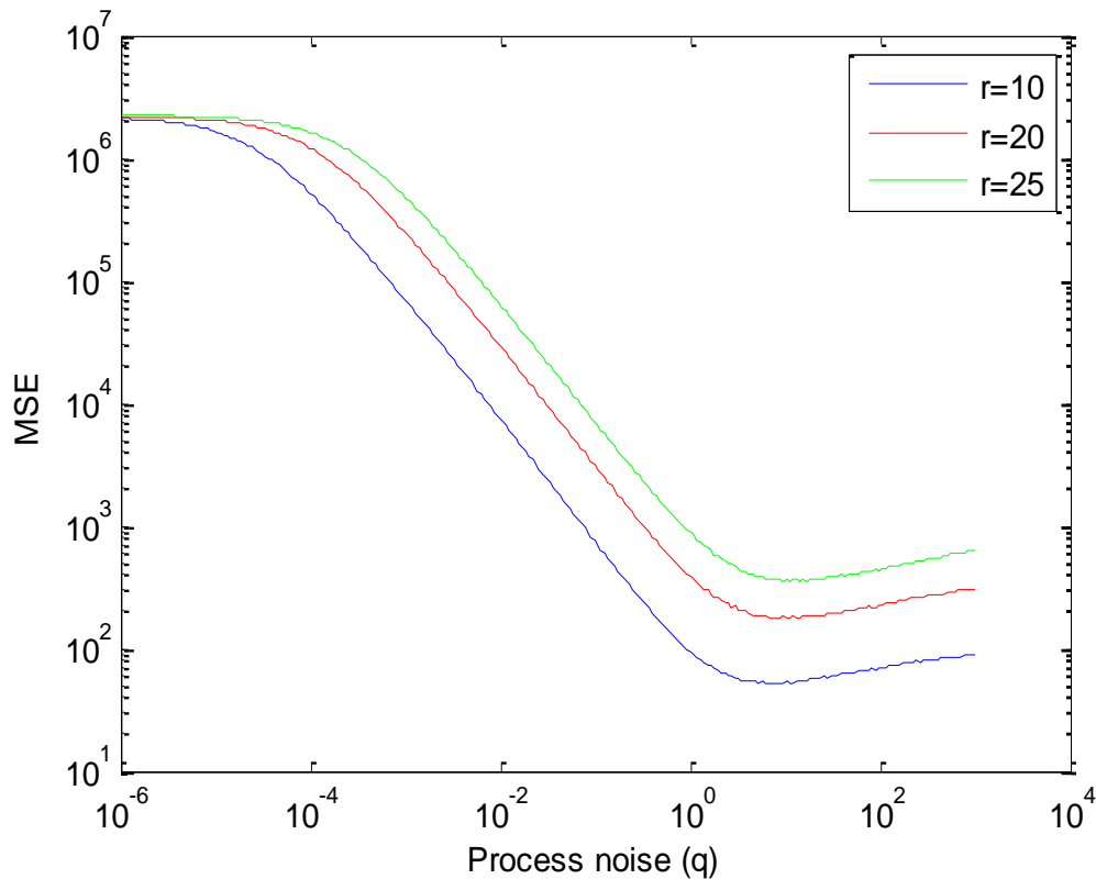
Fig. 2-23: Influence of process noise on the performance of the tracking system.
