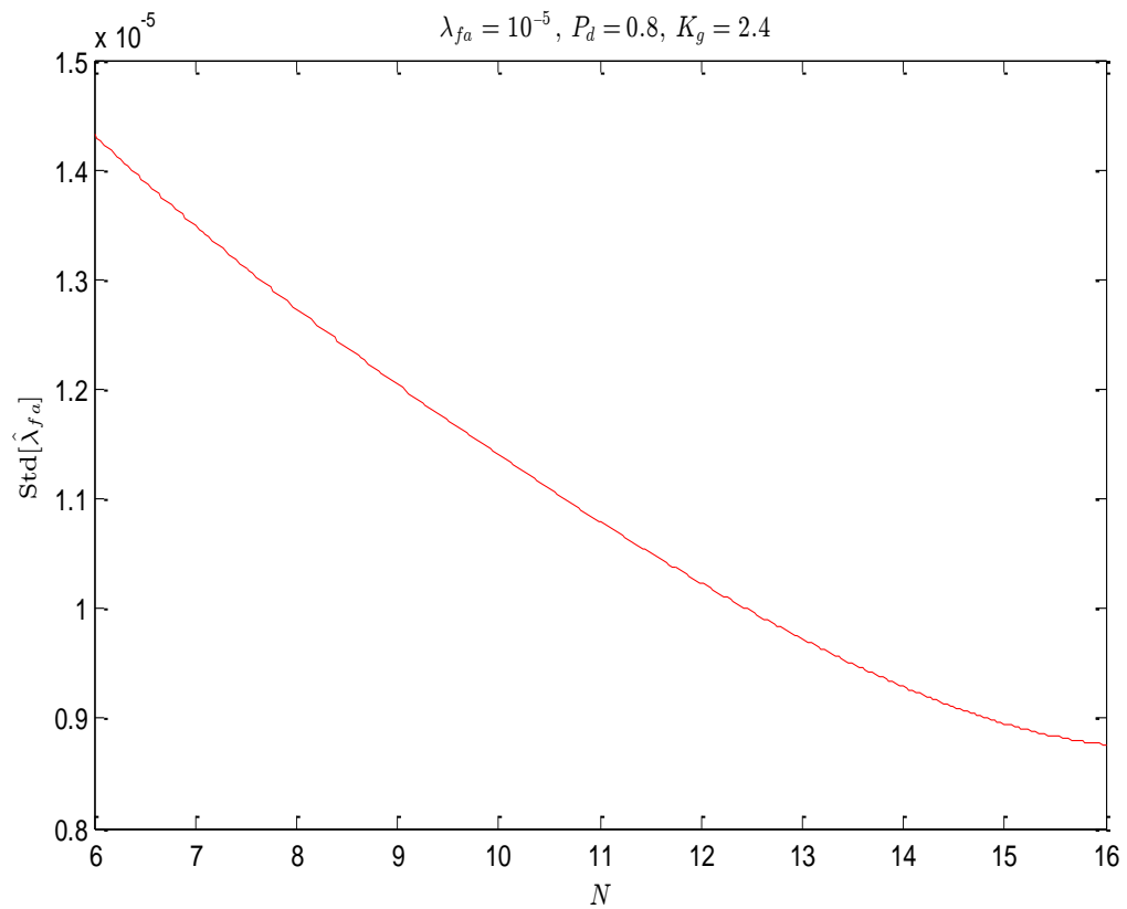
Fig. 4-10: Standard deviation of the estimated density of false alarm as a function of length of sequence N
