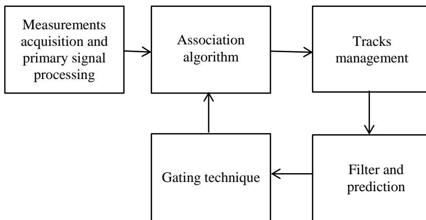
Fig. 2-1: Basic elements of the simple recursive MTT system
