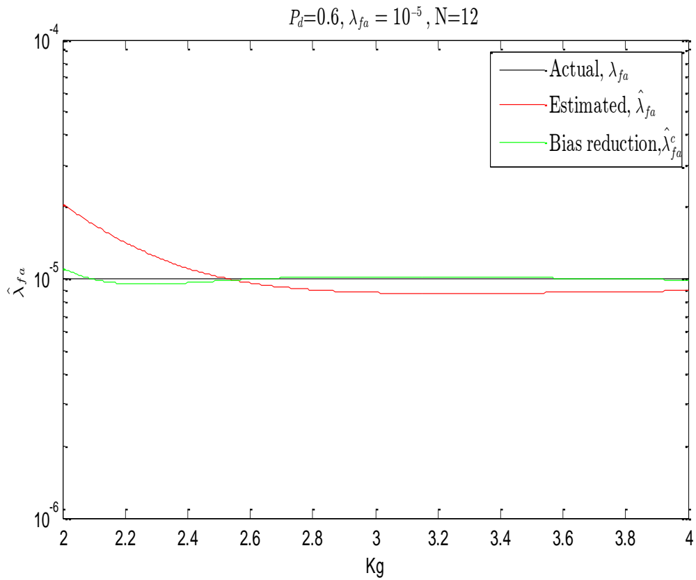
Fig. 4-22: Improvement of the averaged estimated density of false alarm when the actual \lambda_{fa} = 10^{-5} and P_d = 0.6
