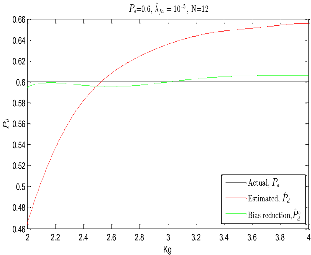
Fig. 4-21: Improvement of the averaged estimated low probability of detection, actual P_d = 0.6
