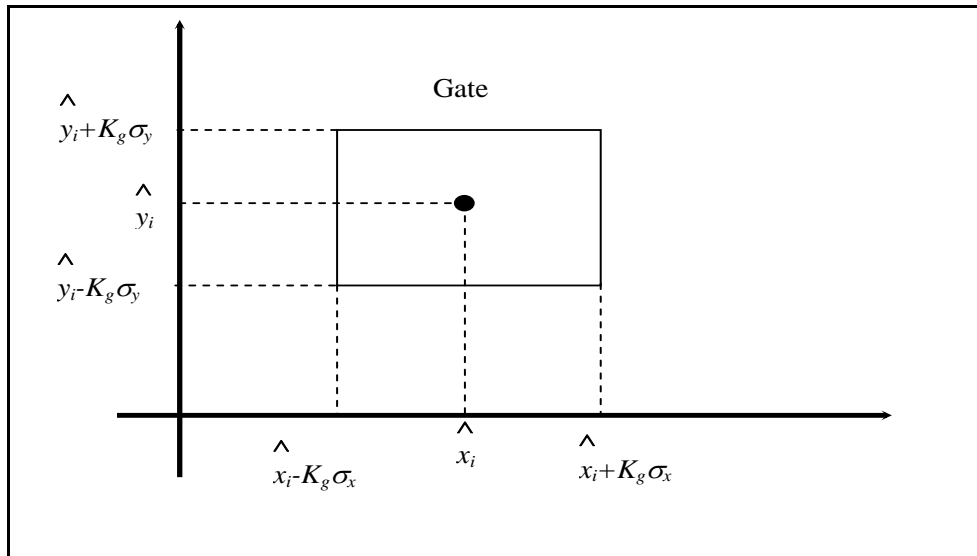
Fig. 2-3: Rectangular gate
