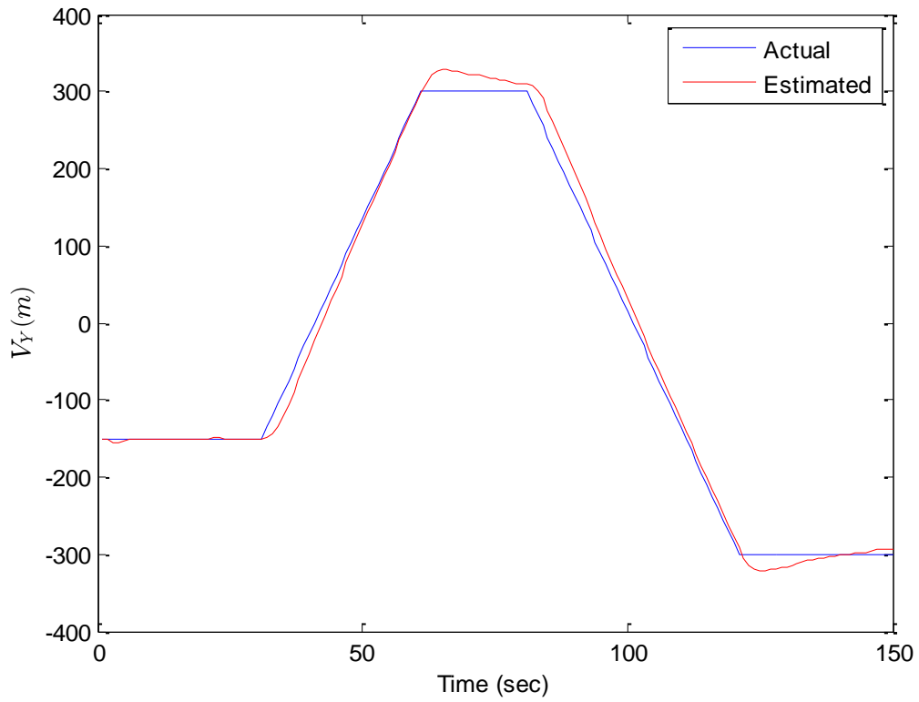
Fig. 2-17: Estimation of velocity along the y-axis
