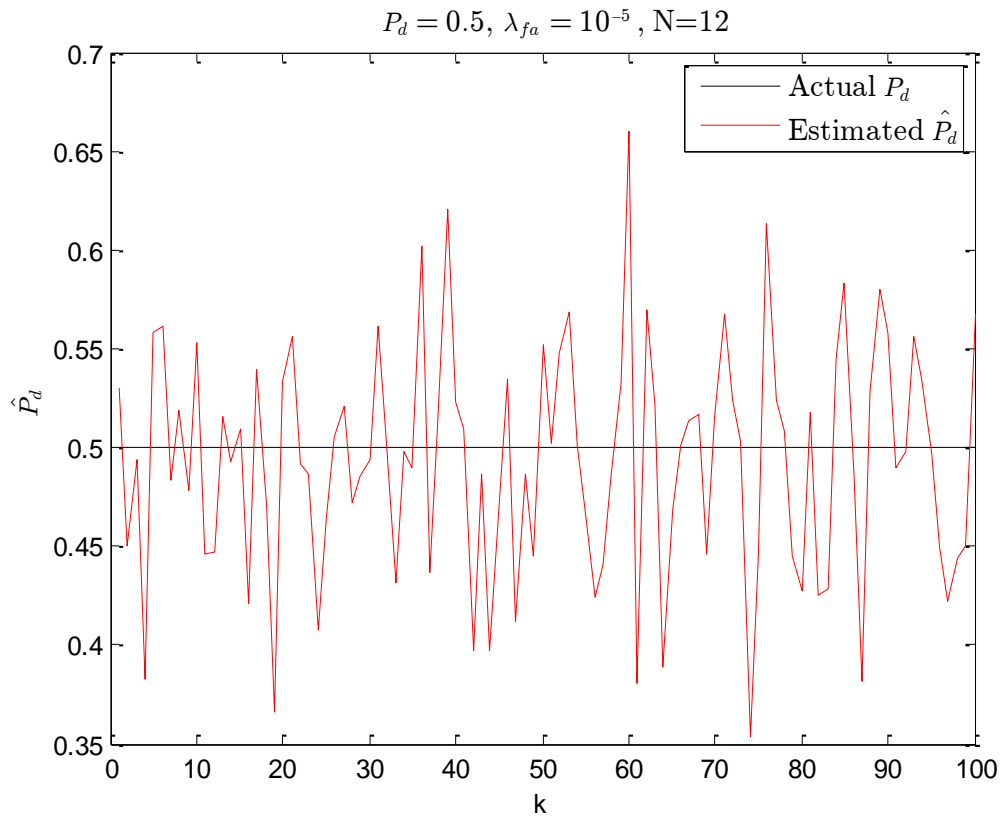
Fig. 4-15: Estimation of the probability of detection
