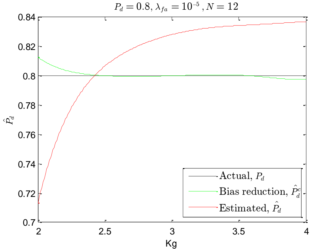
Fig. 4-23: Improvement of the averaged estimated probability of detection, actual P_d = 0.8
