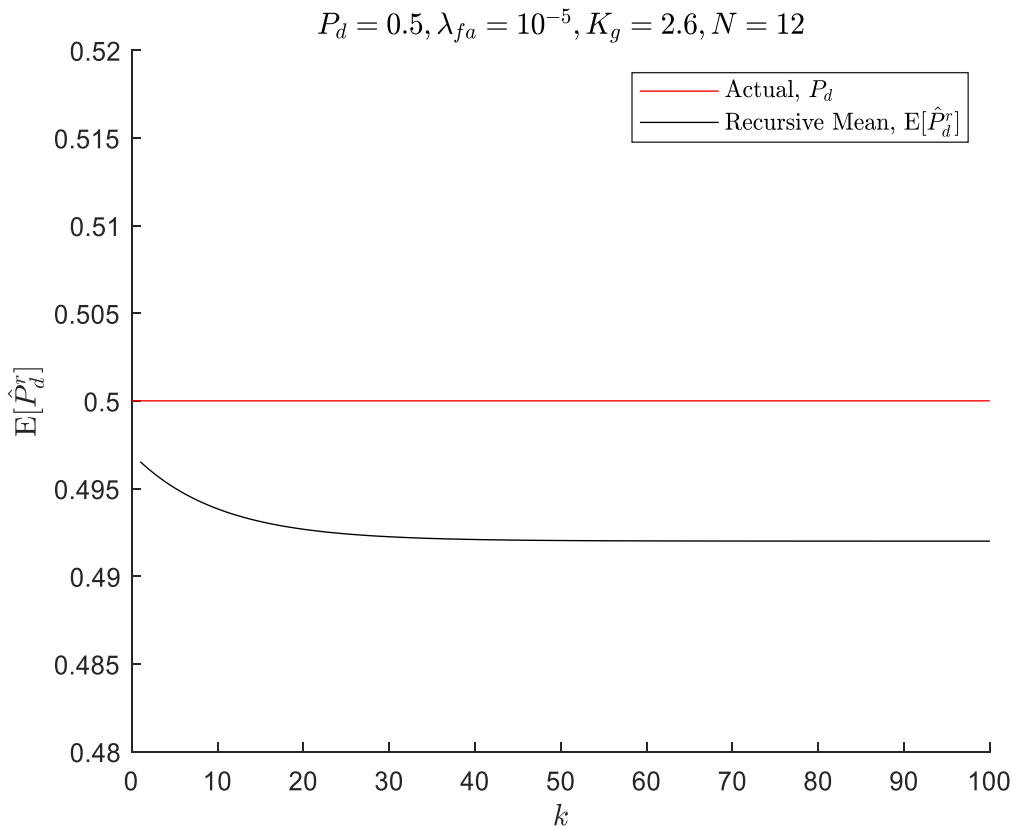
Fig. 4-34: Mean value of recursive estimates of the probability of target detection
