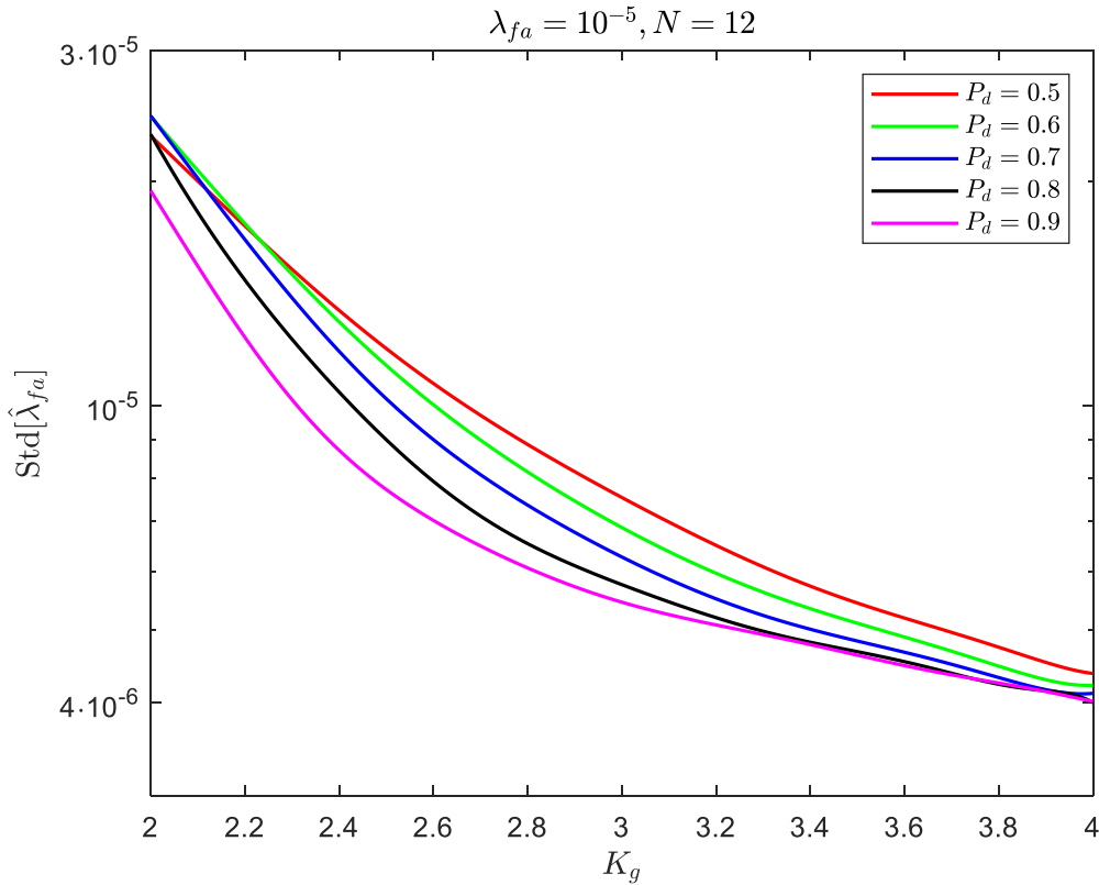
Fig. 4-5: Standard deviation of the estimated density of false alarms
