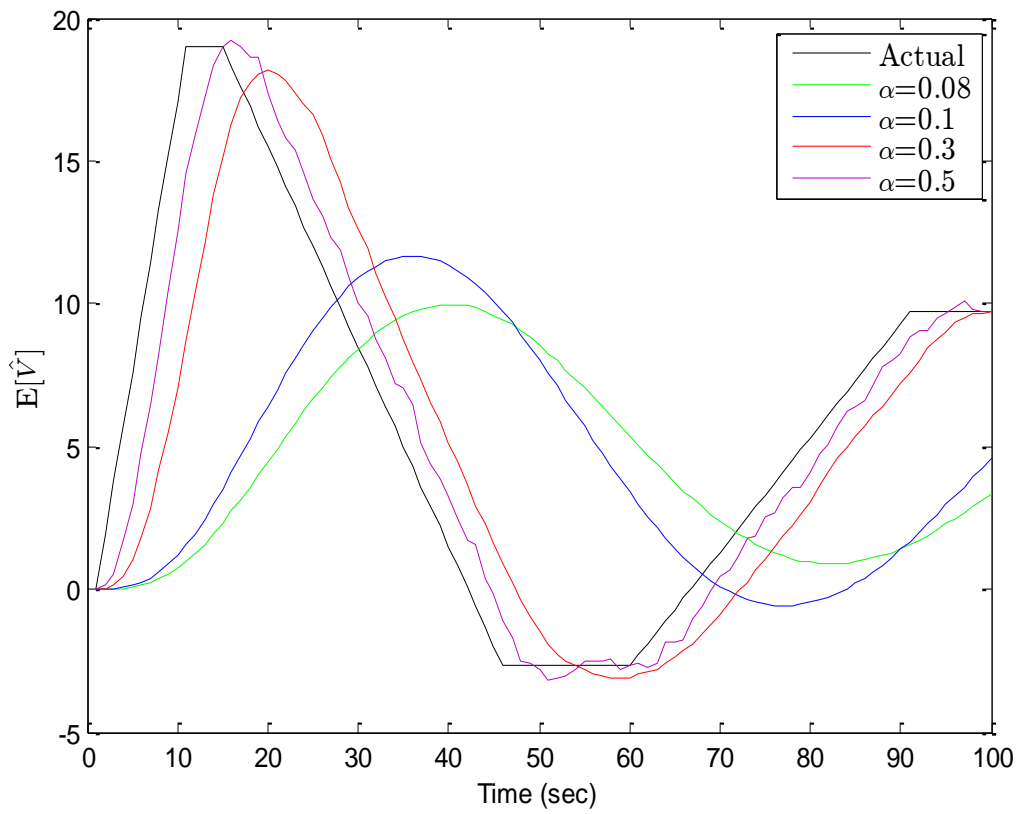
Fig. 2-7: Estimation of velocity ( \alpha - \beta filter)
