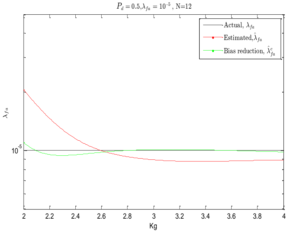
Fig. 4-20: Improvement of the averaged estimated density of false alarm when actual \lambda_{fa} = 10^{-5} and P_d = 0.5
