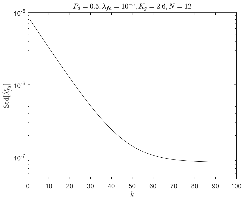
Fig. 4-37: Standard deviation of recursive estimates of the density of false alarm
