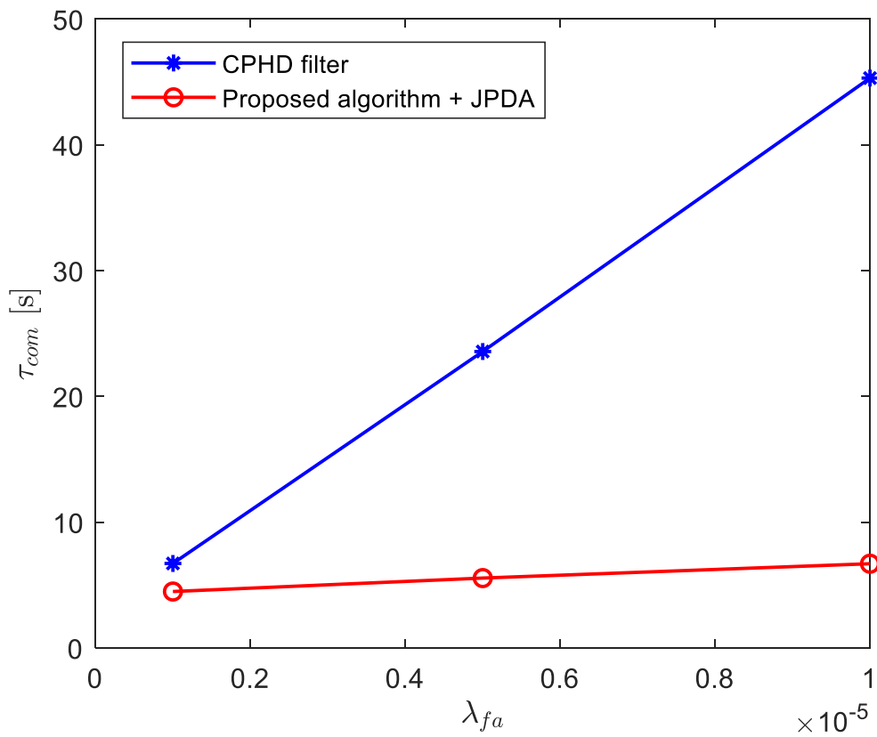
Fig. 4-44: Processing time of the algorithms depending on the density of false alarms with a constant probability of detection ( P_d = 0.8 )
