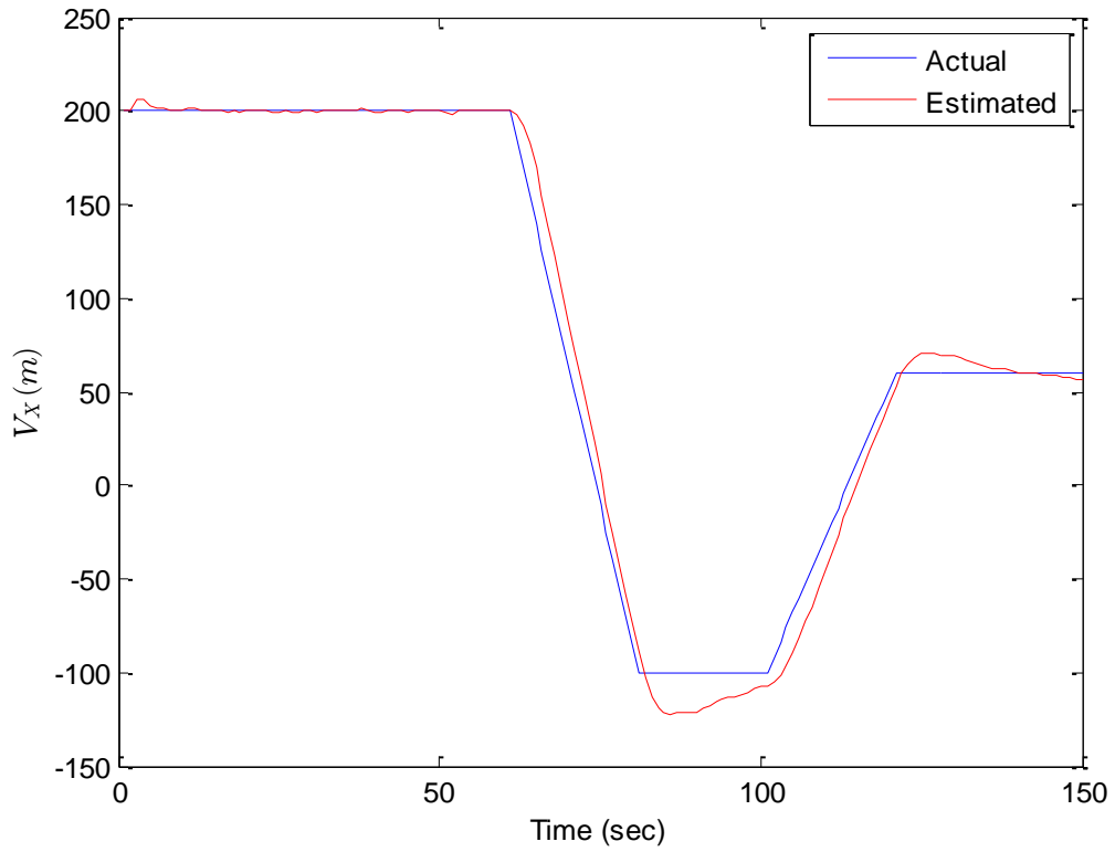
Fig. 2-16: Estimation of velocity along x-axis
