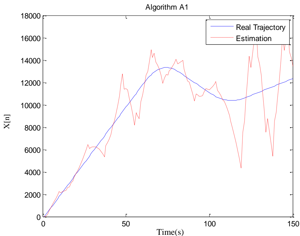
Fig. 2-19: Performance of the standard Kalman filter
