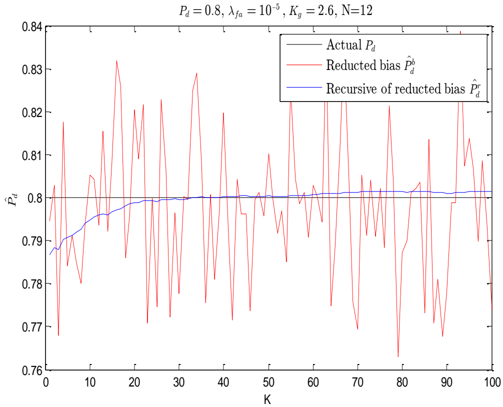
Fig. 4-25: Recursive estimation of probability of detection at fixed actual P_d = 0.8 and \lambda_{fa} = 10^{-5}
