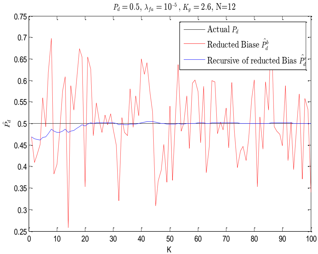
Fig. 4-30: Recursive estimation of probability of detection at fixed actual P_d = 0.5 and \lambda_{fa} = 10^{-5}
