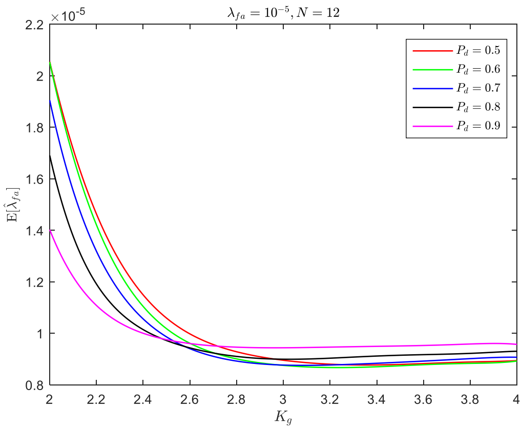
Fig. 4-4: Averaged estimation of the density of false alarms
