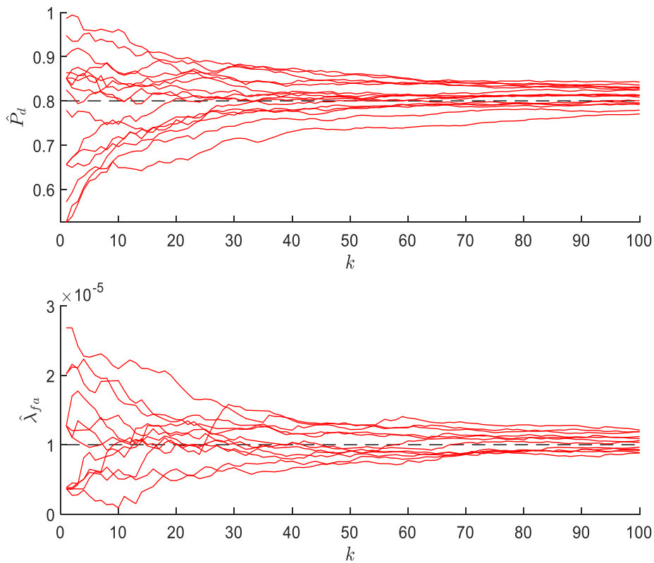
Fig. 4-40: Estimation of the probability of detection and density of false alarms after estimating the measurement noise covariance matrix ( \hat{R} ).
