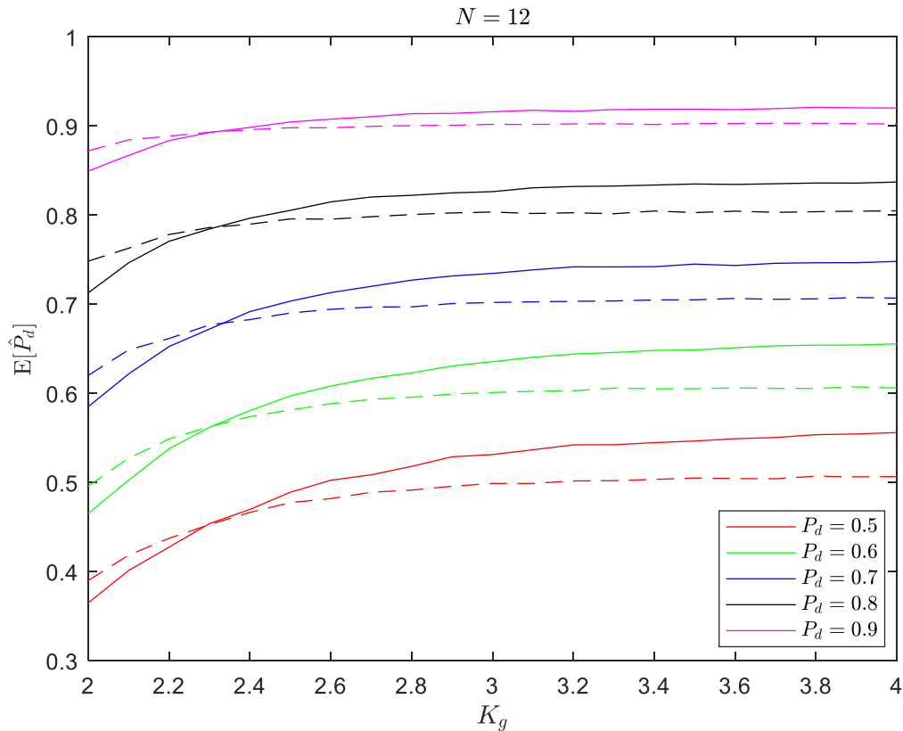
Fig. 4-6: Quality of Estimation of probability of detection as a function of density of false alarms
