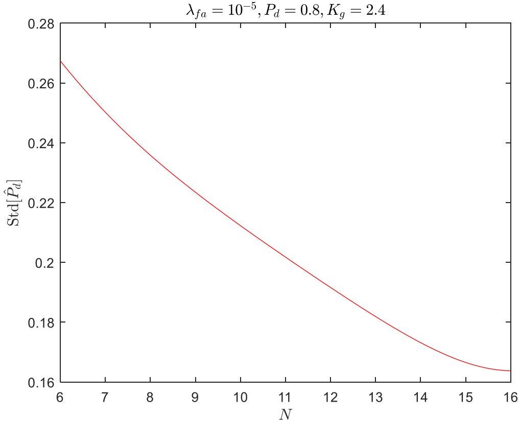
Fig. 4-8: Standard deviation of the estimated probability of detection as a function of length of sequence N
