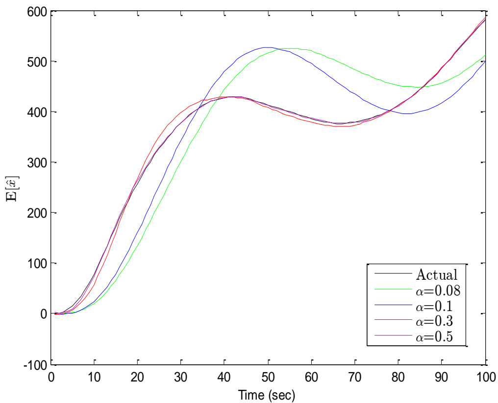
Fig. 2-8: Estimation of position ( \alpha\text{-}\beta\text{-}\gamma filter)
