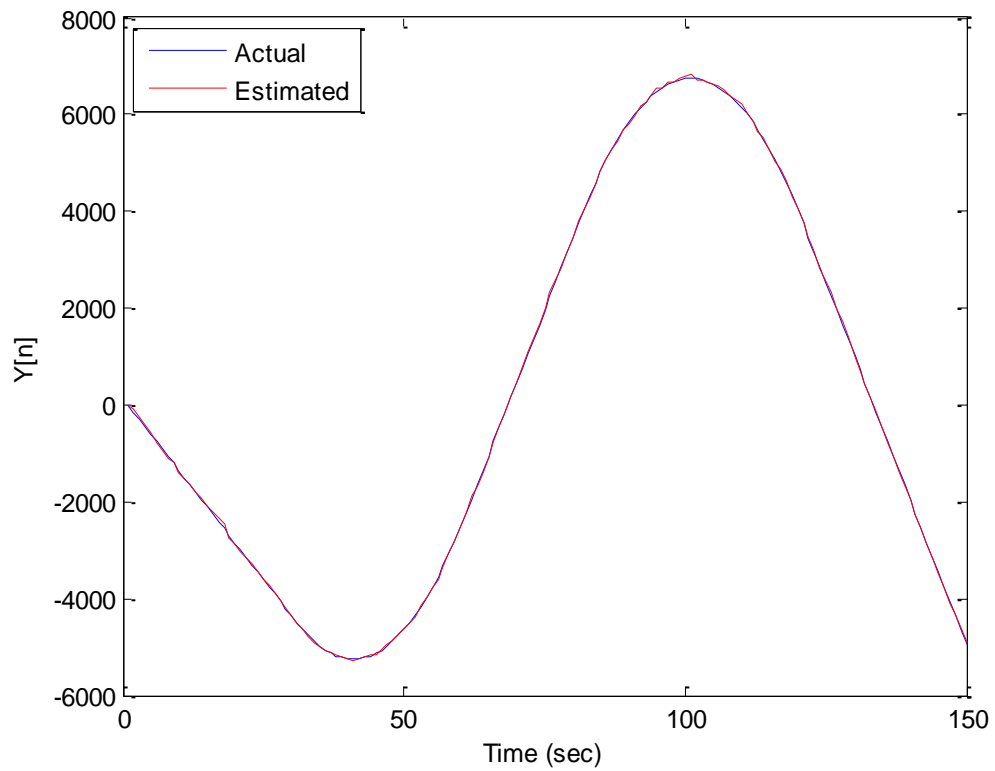
Fig. 2-15: Kalman filter performance in Y plane
