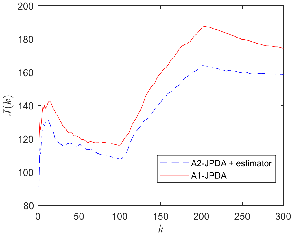
Fig. 4-42: Cumulative RMSE measure for algorithms A1 (with constant parameters) and A2 (with adaptive parameters)
