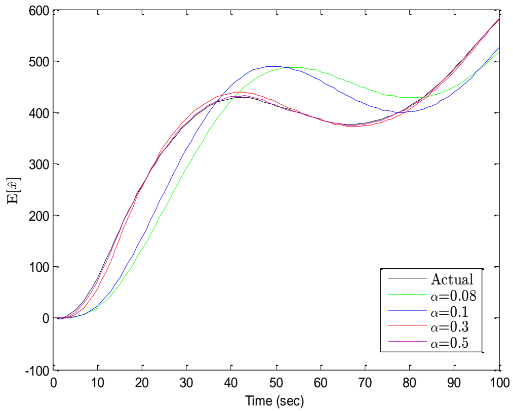
Fig. 2-6: Estimation of position ( \alpha - \beta filter)
