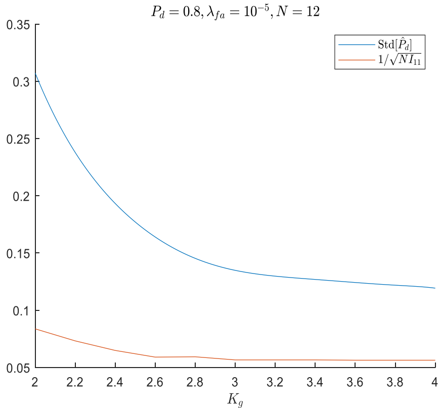
Fig. 4-41: Comparison of Cramer-Rao lower bound and experimentally determined standard deviation of \hat{P}_d
