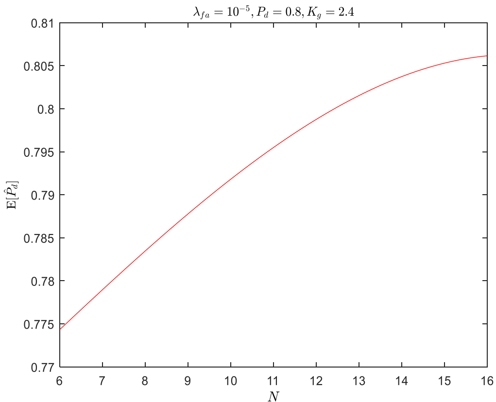
Fig. 4-7: Average estimations of probability of detection as a function of length of sequence N
