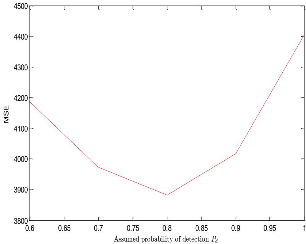
Fig. 3-4: Influence of applying inaccurate values of probability of detection on the performance of the target tracking system
