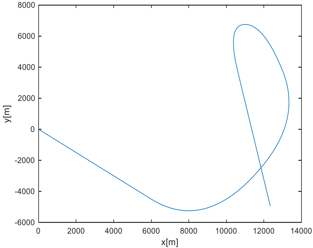
Fig. 2-18: The true trajectory of the tracked target
