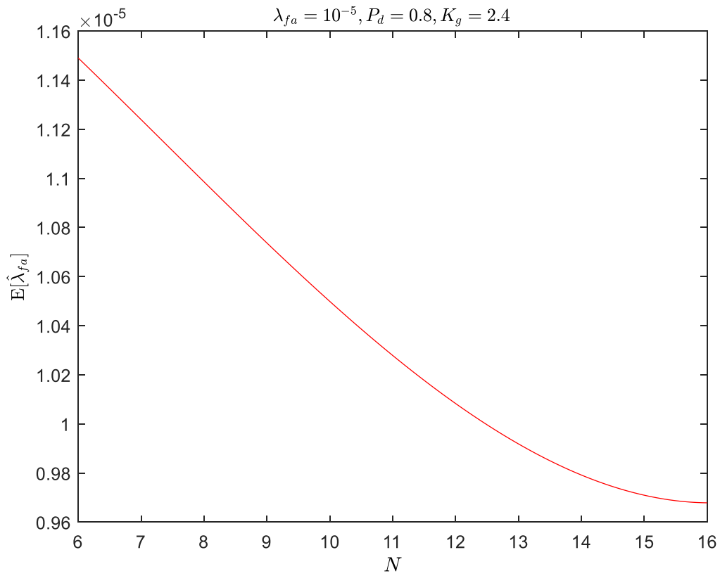
Fig. 4-9: Average estimations of the density of false alarm as a function of length of sequence N
