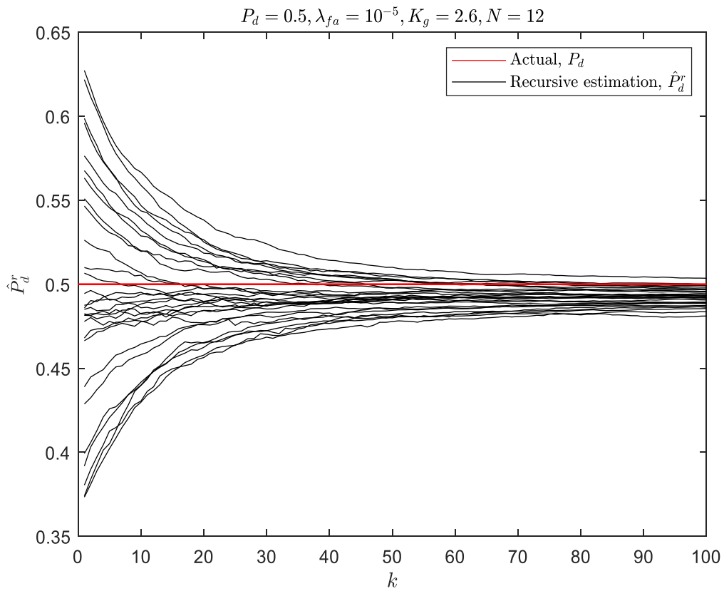
Fig. 4-32: Recursive estimation of probability of detection at fixed actual P_d = 0.5 and \lambda_{fa} = 10^{-5} for different initial conditions
