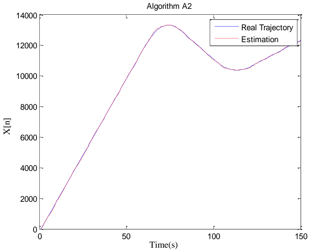
Fig. 2-20: Performance of the modified Kalman filter
