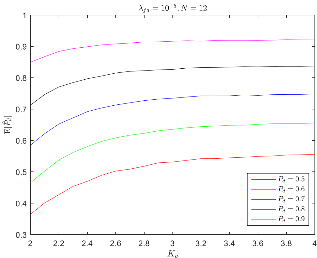
Fig. 4-2: Averaged estimation of the probability of detection
