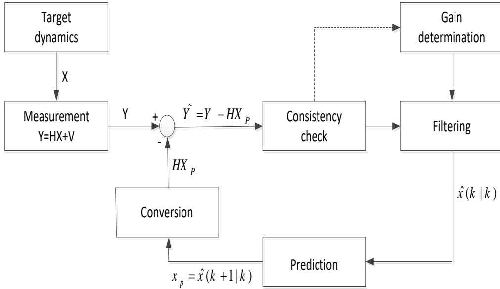
Fig. 2-5: Flow diagram of the filtering and the prediction process
