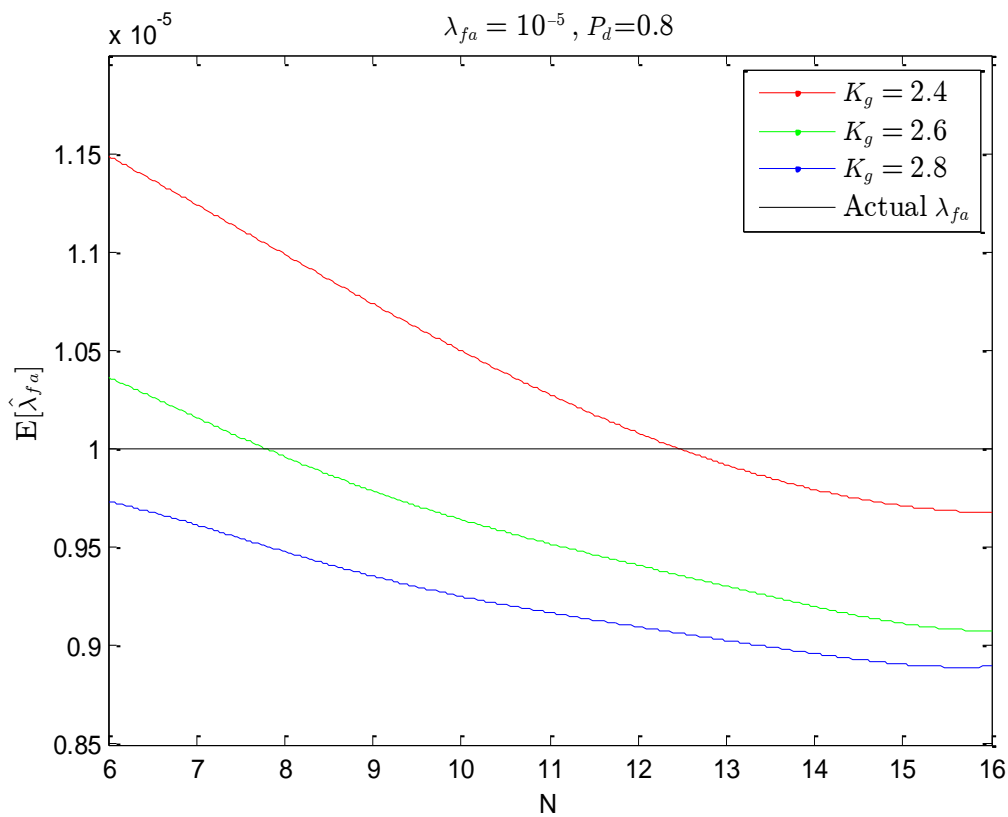
Fig. 4-13: Average of the estimated density of false alarm as a function of length of sequence N for different values of gate size K_g
