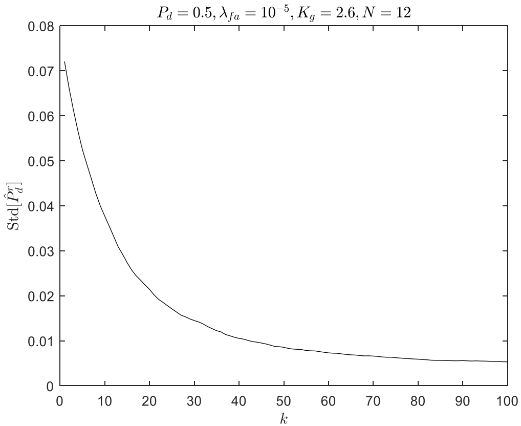
Fig. 4-35: Standard deviation of recursive estimates of the probability of detection.
