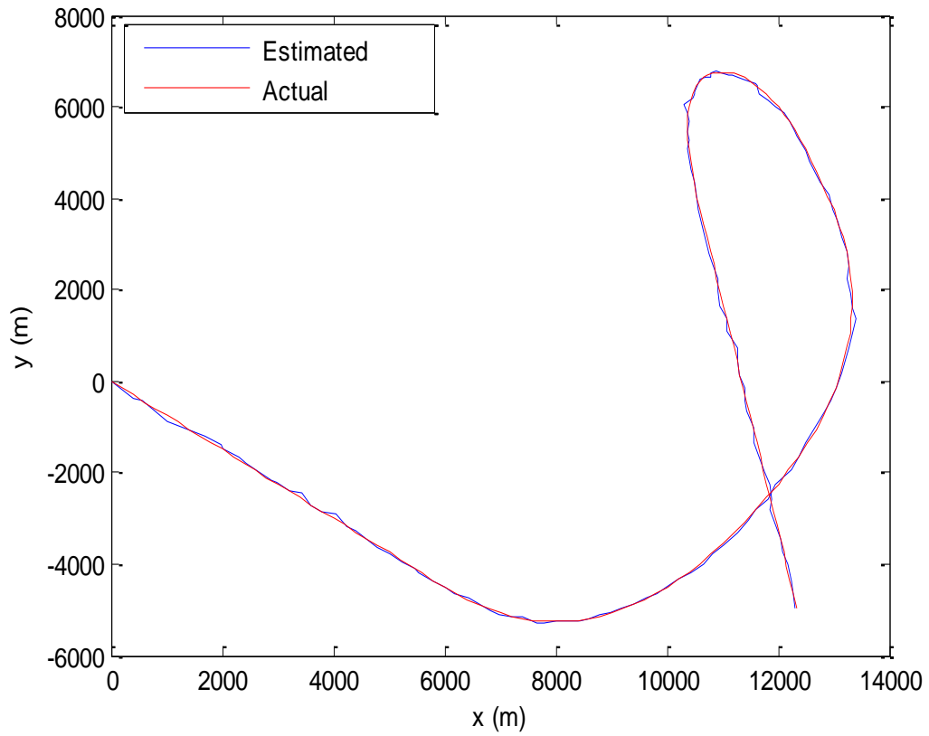
Fig. 2-14: Kalman filter performance in two planes
