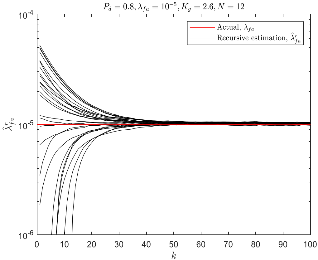
Fig. 4-29 Recursive estimation of density of false alarms at fixed
