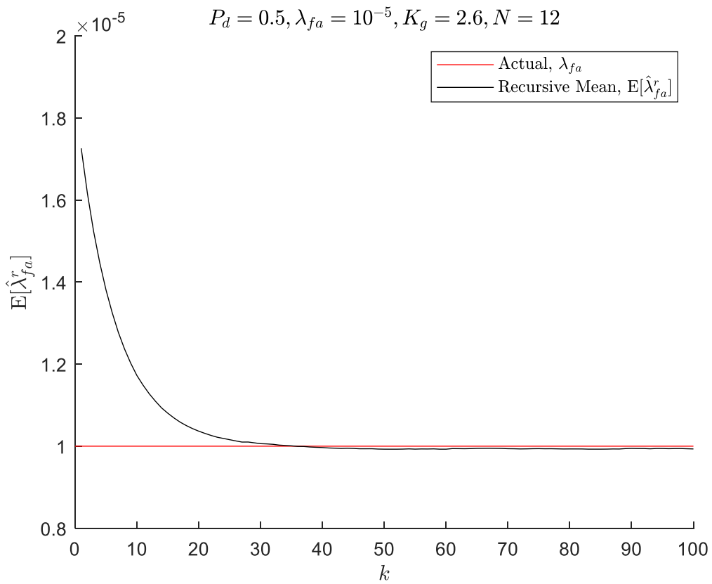
Fig. 4-36: Mean value of recursive estimates of the density of false alarm.
