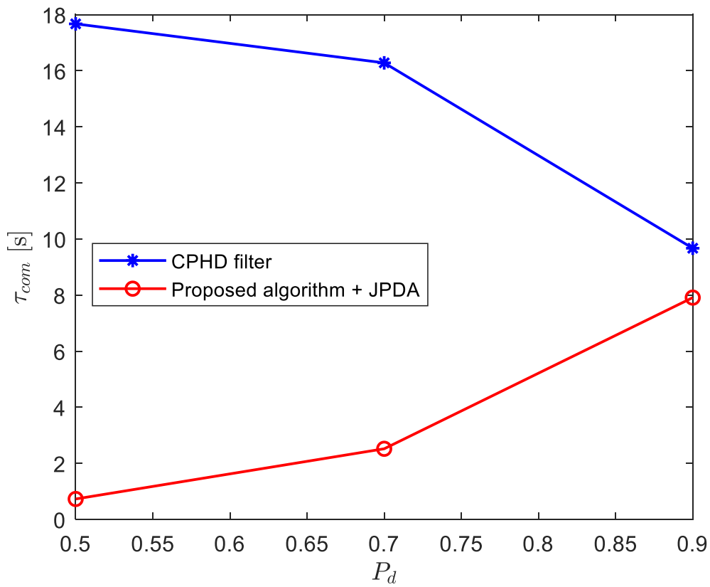
Fig. 4-43: Processing time of the algorithms depending on the probability of detection with a constant density of false alarms ( \lambda_{fa} = 2.5 \times 10^{-6} )
