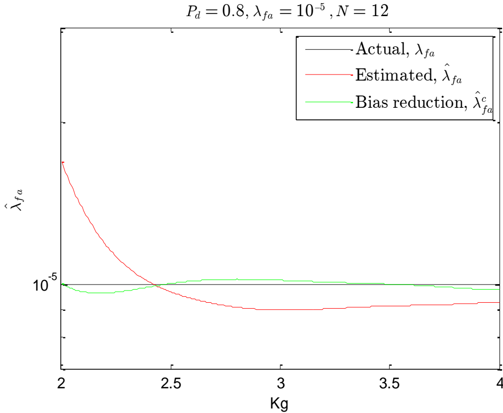
Fig. 4-24 Improvement of the averaged estimated density of false alarm when the actual \lambda_{fa} = 10^{-5} and P_d = 0.8
