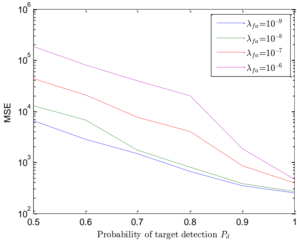
Fig. 3-1: Influence of the probability of detection on the performance of the target tracking system
