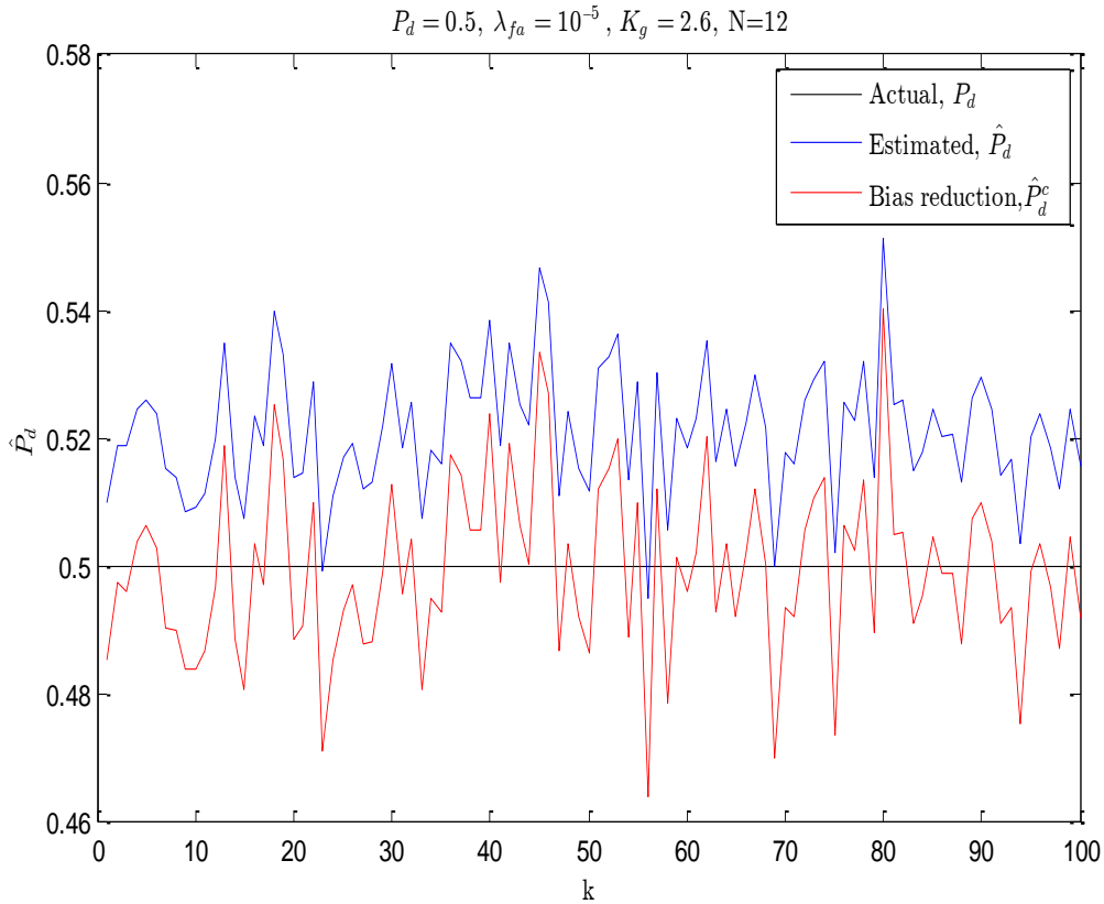
Fig. 4-17: Estimated probability of detection \hat{P}_d and bias reduced \hat{P}_d^c
