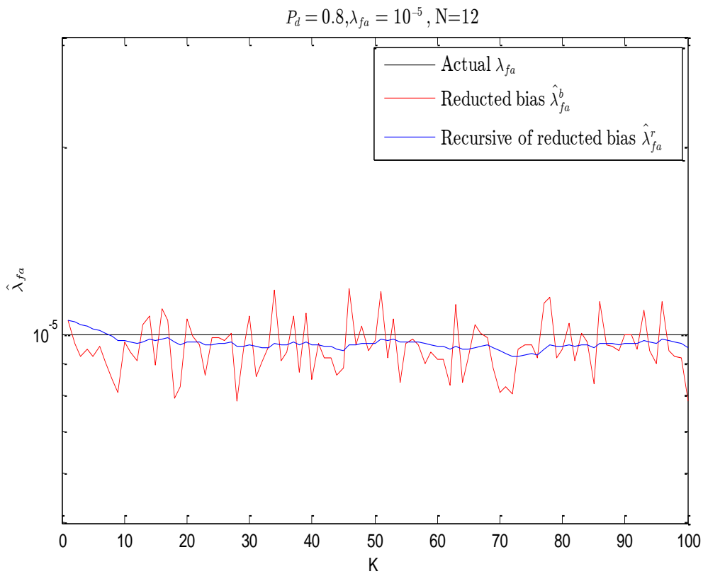
Fig. 4-26: Recursive estimation of density of false alarms at fixed actual P_d = 0.8 and \lambda_{fa} = 10^{-5}
