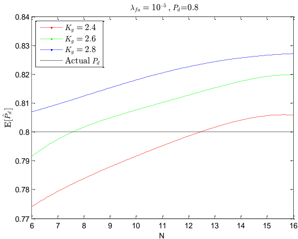
Fig. 4-11: Average of the estimated probability of detection as a function of length of sequence N for different values of gate size K_g
