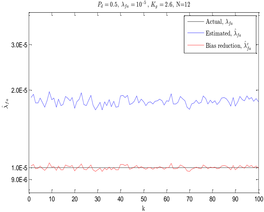
Fig. 4-18: Estimated density of false alarms \hat{\lambda}_{fa} and bias reduced \hat{\lambda}_{fa}^c
