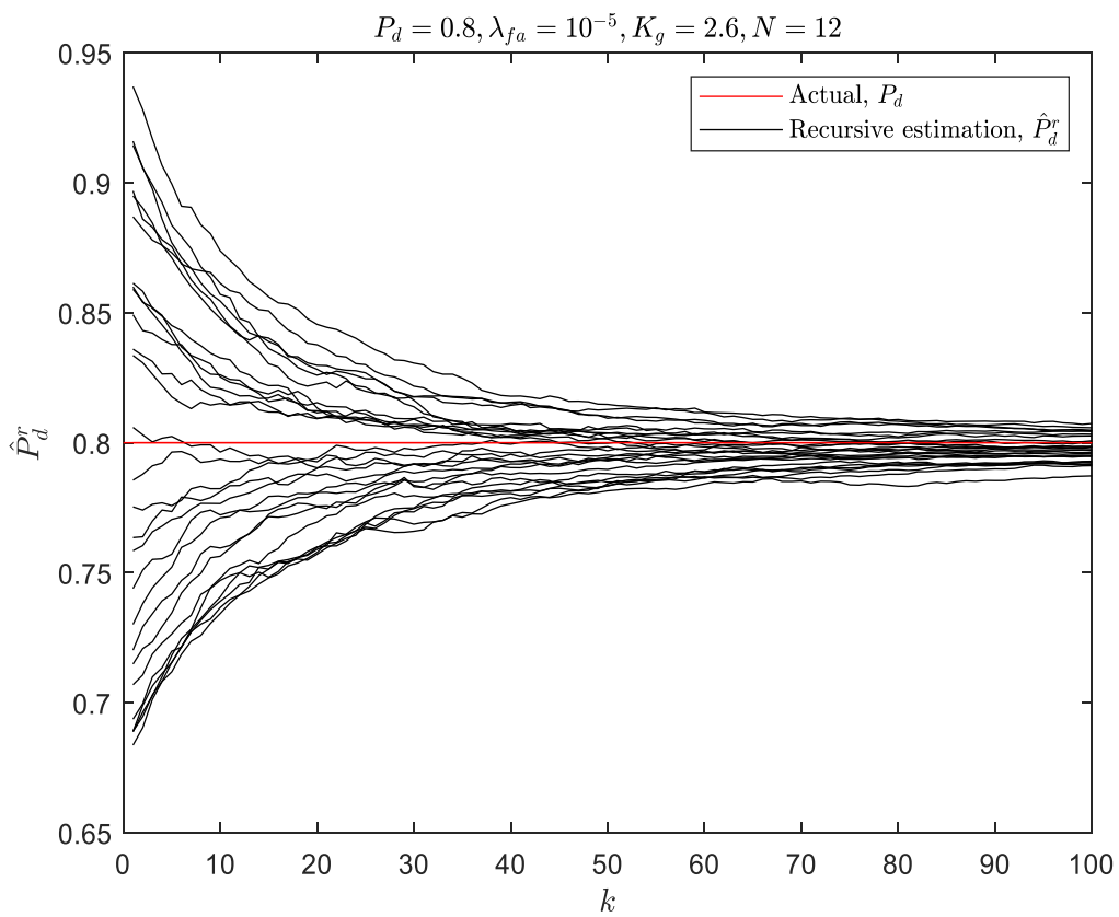
Fig. 4-28: Recursive estimation of probability of detection at fixed actual
