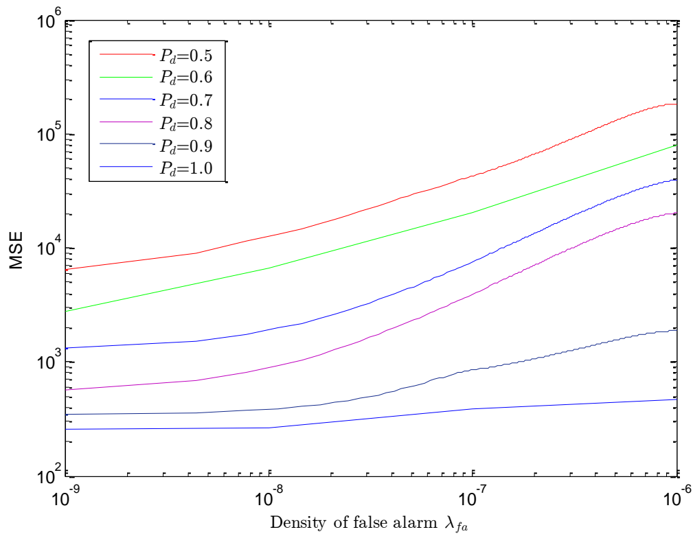
Fig. 3-2: Influence of the density of false alarm on the performance of the target tracking system
