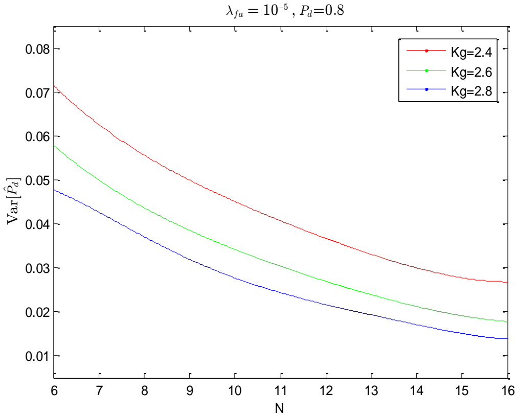
Fig. 4-12: Variance of the estimated probability of detection as a function of length of sequence N for different values of gate size K_g
