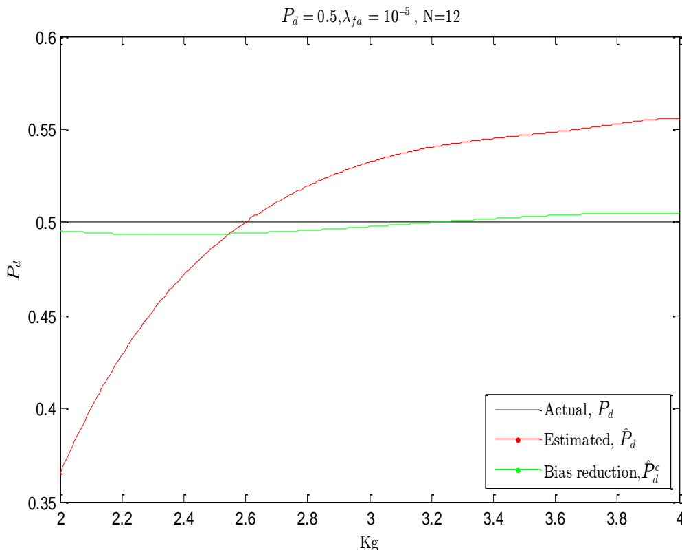
Fig. 4-19: Improvement of the averaged estimated low probability of detection, actual P_d = 0.5
