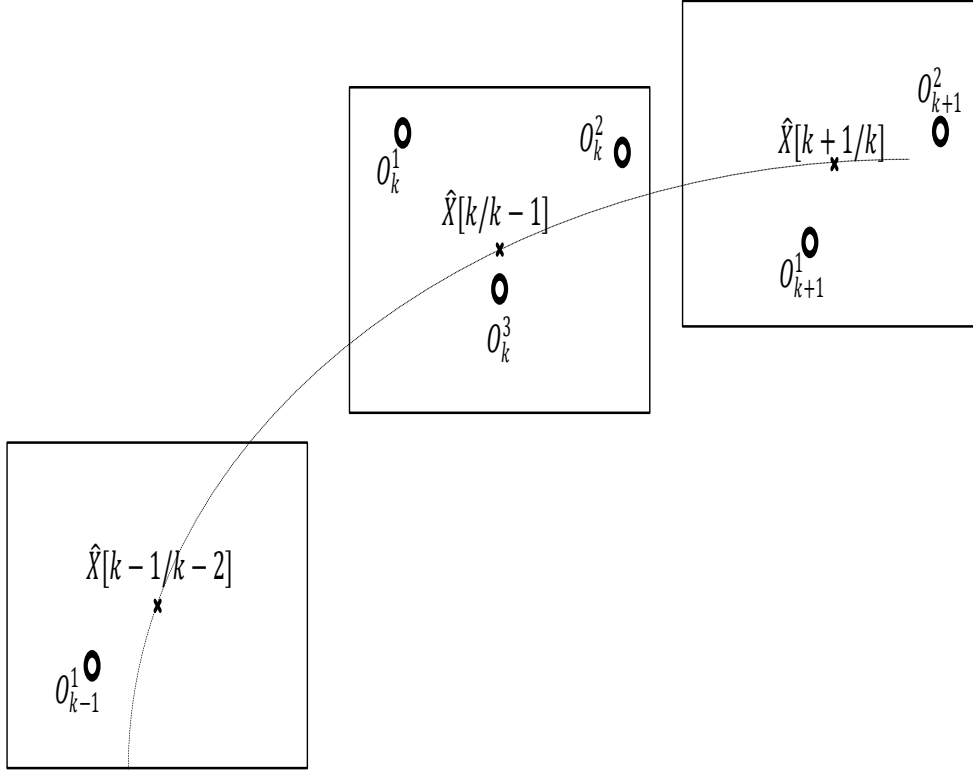
Fig. 4-1: Gate function and observations for three consecutive scans
