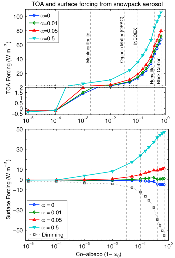
Figure 28. Daily-mean (top) top-of-atmosphere and (bottom) surface changes in net solar power (radiative forcing) as a function of single-scattering co-albedo ( 1-\omega_0 ) for all aerosol at 500 nm. Extinction optical depth of the atmospheric aerosol is fixed at 0.2, and the environment represents a clear-sky atmosphere overlying a snowpack with effective grain radius of 200 \mu\text{m} on 1 April at 45°N. Curves are shown for different values of \alpha , which is the ratio of particle mixing ratio in snow to atmospheric column burden ( (\text{kg kg}^{-1})(\text{kg m}^{-2})^{-1} ). Radiative forcings represent the combined influence of particles in the atmosphere and snow. For reference, the change in downwelling surface insolation (“dimming”) is also depicted. Vertical lines depict common co-albedo values of BC and organic matter, and that measured during the Indian Ocean Experiment (INDOEX) [ Ramanathan et al. , 2001b]. Also shown are co-albedo values of strongly and weakly absorbing components of dust aerosols. The plot illustrates that (1) any mixture of atmospheric BC and organic matter exerts a positive ToA radiative forcing over snowpack and (2) a small amount of aerosol mixed within the underlying snowpack exerts a darkening effect that exceeds the loss of absorbed energy from surface dimming caused by the atmospheric constituents. Figure from Flanner et al. [2009].
