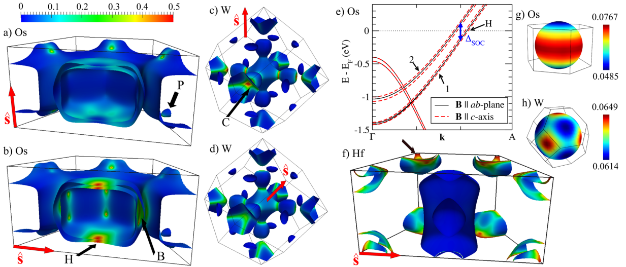
FIG. 1 (color online). Fermi surfaces of Os (a), (b), W (c), (d), and Hf (f). For an illustration of the nested sheets of Os and Hf, only half of the Fermi surface is shown. The spin-mixing b_{k_s}^2 is shown in terms of a color code with the SQA \hat{s} (red arrows at the lower left corners) along the c axis (a) and the ab plane (b). The splitting introduced by SOC and by a Zeeman-like field is shown in the band structure of Os (e) along the \Gamma -A direction (BZ center to hexagonal-face center). For W, the cases \hat{s} \parallel [001] and [111] are shown in (c) and (d), respectively. In (g) and (h), the Elliott-Yafet parameter b_{\xi}^2 is shown as a function of the SQA direction for Os and W, respectively [in (g) and (h) the color scale is different than in the Fermi-surface plots]. The average of b_{\xi}^2 over all directions of \hat{s} , corresponding to polycrystalline samples, are 0.0666 for Os and 0.0627 for W. (f) Hf Fermi surface with \hat{s} parallel to the ab plane. An arrow indicates one of the spin-flip hot loops, clearly visible in red on the hexagonal face of the BZ. The hot loops vanish when \hat{s} is rotated to the c axis, resulting in an anisotropy of 830% of the Elliott-Yafet parameter.
