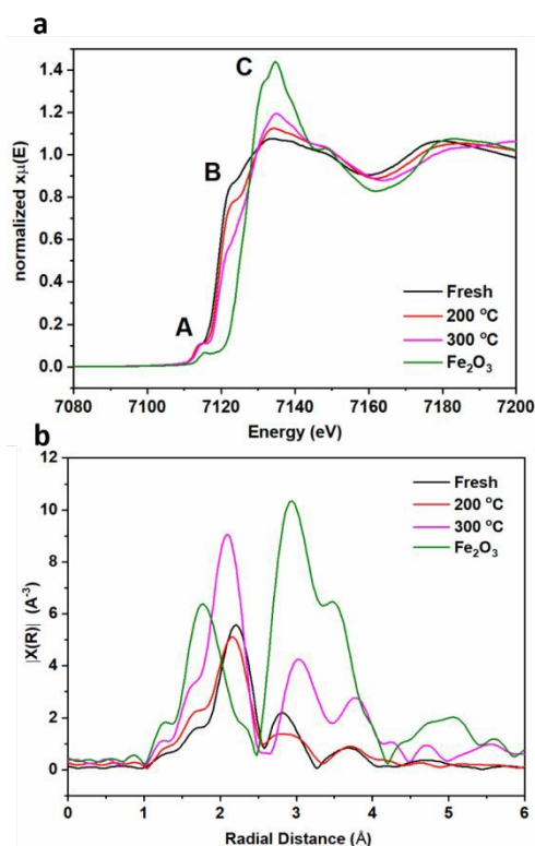
Figure 5: XAS data of Fe K-edge including (a) XANES and (b) Fourier Transform EXAFS for pyrrhotite samples; fresh (black), 200^\circ\text{C} calcination (red), 300^\circ\text{C} calcination (pink) and \text{Fe}_2\text{O}_3 reference sample (green). Blue arrows indicate direction of increasing oxygen ligands.
