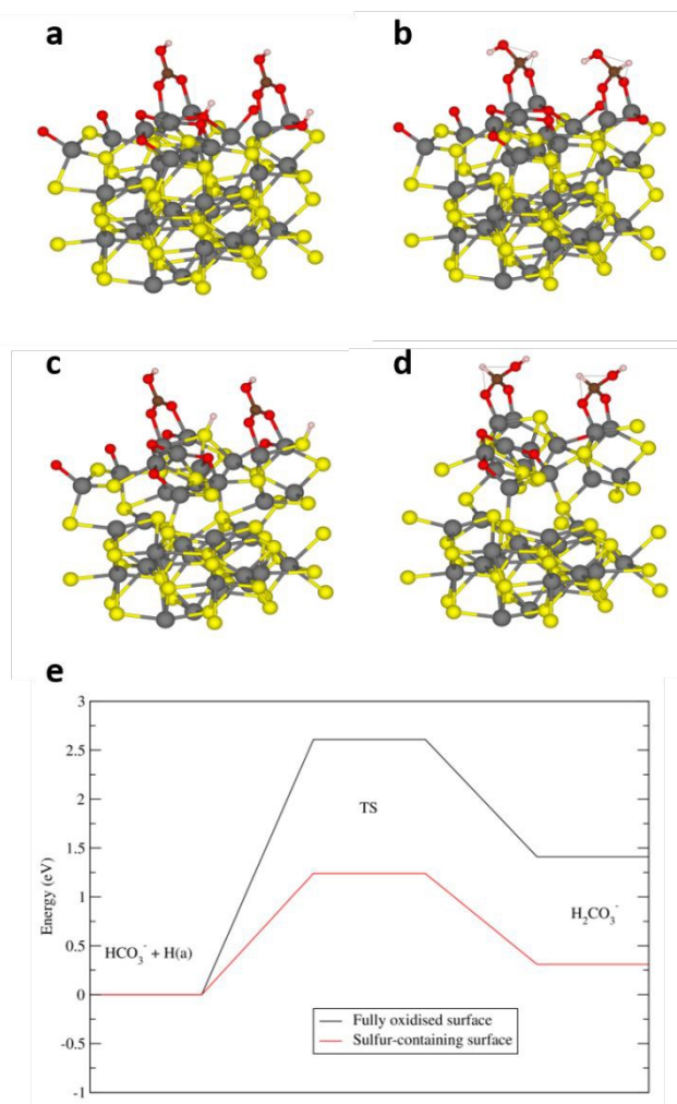
Figure 4: Adsorption (a & c) and hydrogenation (b & d) structures of \text{HCO}_3^- on the fully oxidised termination A (a & b) and sulfur-containing termination B (c & d) of FeS stoichiometric pyrrhotite. Colour code: Fe-grey, S-yellow, O-red, C-brown, H-white. (e) Energetics of the carbon hydrogenation step on the fully oxidised termination A and sulfur-containing termination B surface showing the position of reactants ( \text{HCO}_3^- ), products ( \text{H}_2\text{CO}_3^- ) and transition states (TS). The hydrogen species on the surface of the reactant configurations is indicated with H(a).
