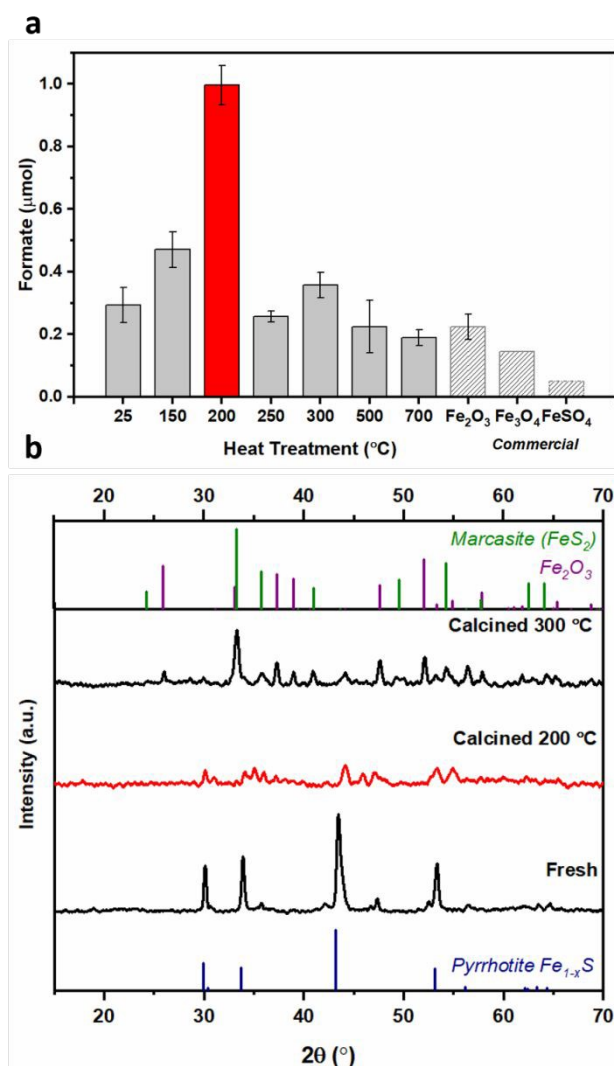
Figure 2: (a) Comparison of the effect of different calcination temperatures pyrrhotite catalyst for the hydrogenation of CO 2 to produce formate, Reaction conditions: catalyst: 20mg; 1M NaOH solution: 4 ml; pCO 2 :H 2 : (1:1) 20 bar; 125 °C for 3 days. (b) XRD spectra of pyrrhotite fresh, calcined at 200 °C, and calcined at 300 °C, compared to corresponding XRD patterns sourced PDF cards. (blue) – pyrrhotite, 01-079-5974; (green) – Marcasite, FeS 2 , 01-074-1051; (purple) – Fe 2 O 3 , 01-085-0987.
