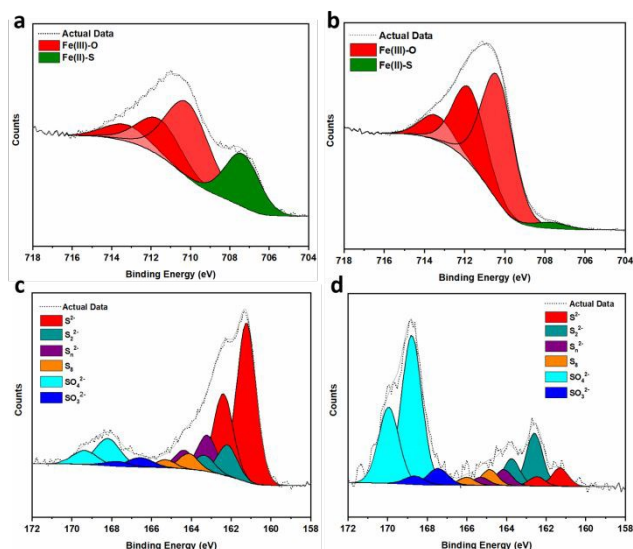
Figure 3: (a-d) XPS spectra of fresh and calcined samples (a) Fe2p, Fresh (b) Fe2p, Calcined 200 °C (c) S2p, Fresh (d) S2p, Calcined 200 °C. Plot details in (Table S2).
