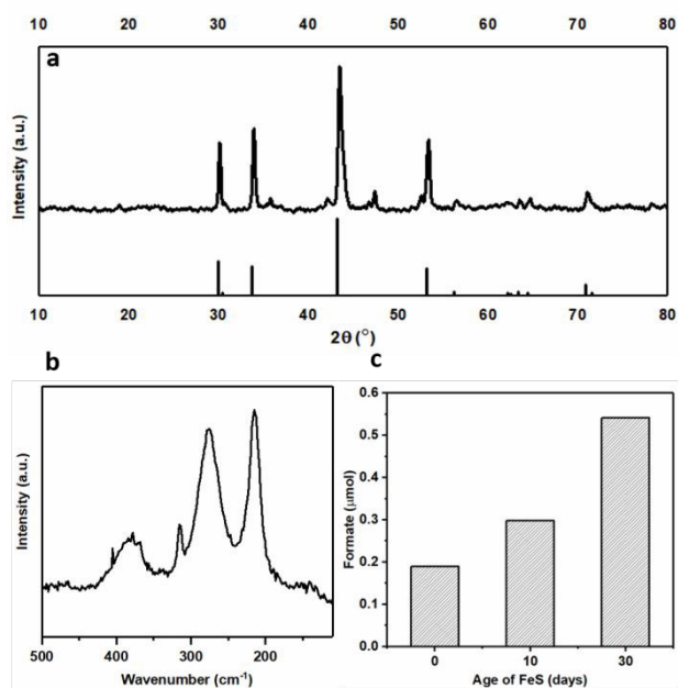
Figure 1: Freshly synthesised pyrrhotite analysed by (a) XRD with pyrrhotite reference peaks (JCPDS 01-079-5974 PDF file) and (b) Raman spectroscopy. (c) Effect of aging the pyrrhotite catalyst in air on formate production
