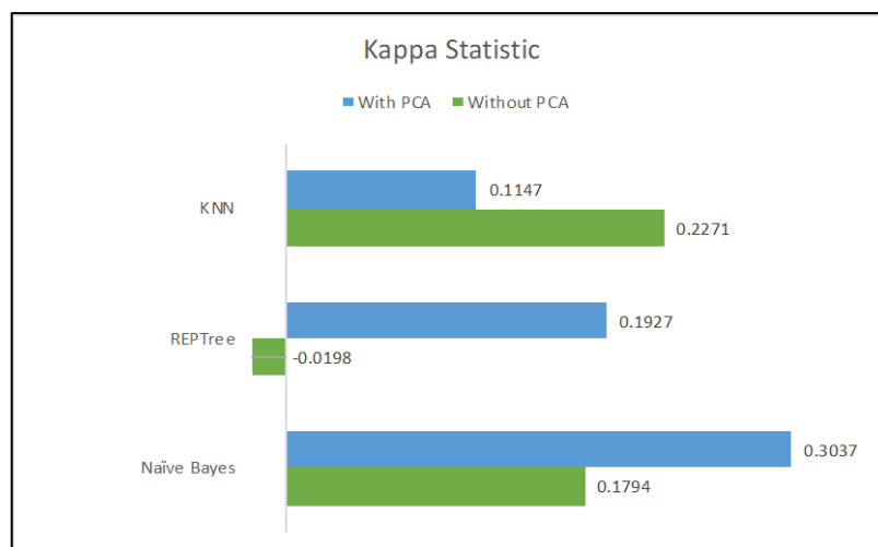
Fig. 6. Kappa statistic for three models with and without PCA
