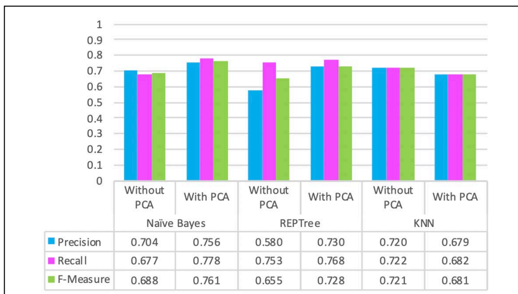
Fig. 7. Precision, recall, and F-measure for three models with and without PCA
