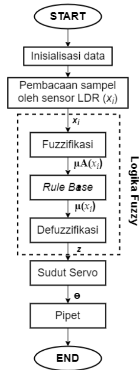
Gambar 6. Flowchart Sistem
