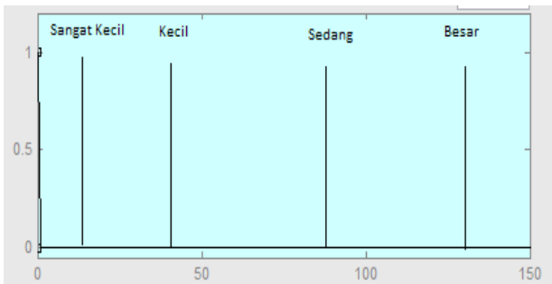
Gambar 5. Representasi Variabel Fuzzy Sugeno output
