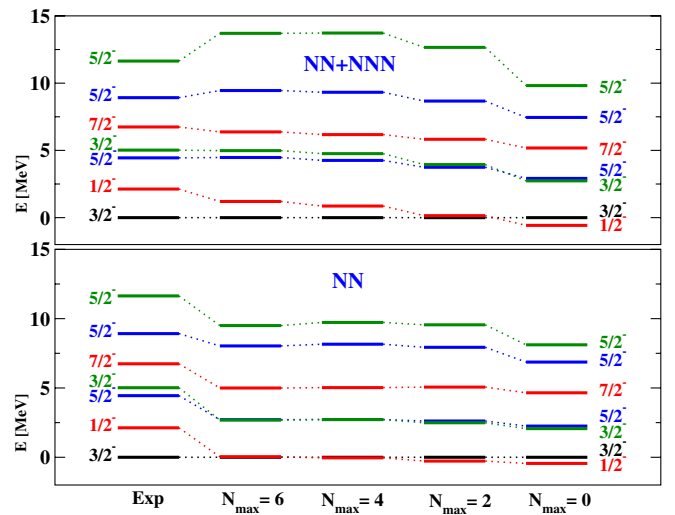
FIG. 3 (color online). {}^{11}\text{B} excitation spectra as function of the basis space size N_{\text{max}} at \hbar\Omega = 15 MeV and comparison with experiment. The isospin of the states depicted is T = 1/2 .
