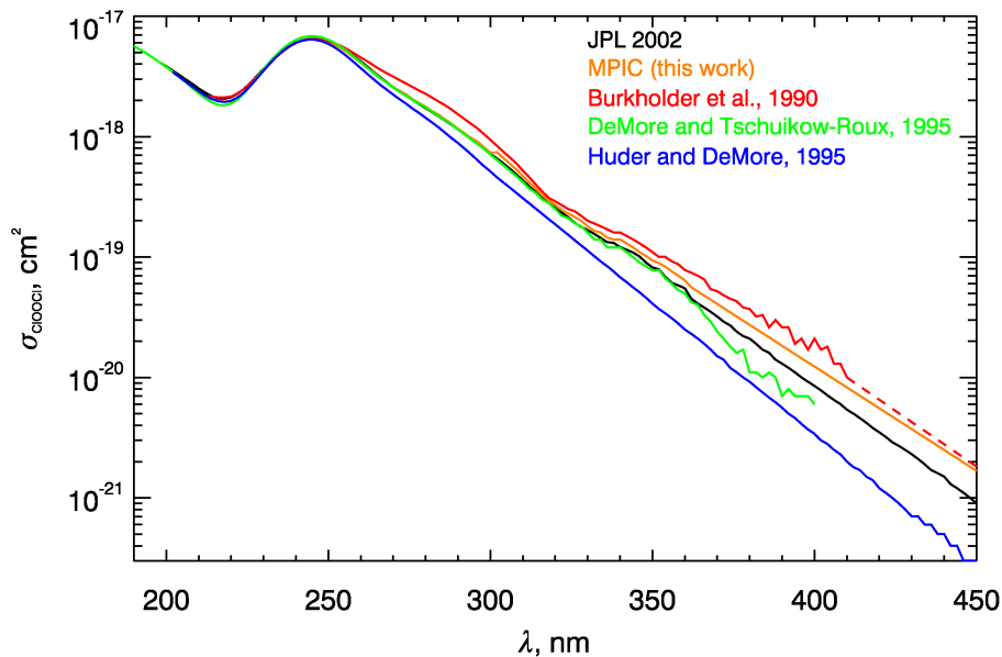
Fig. 5. Comparison of UV-Vis absorption spectra of ClOOCl.
